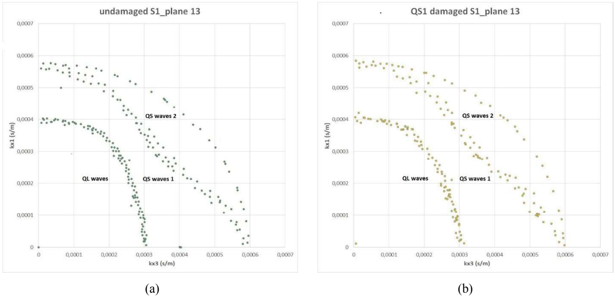
Figure 12: Experimental slowness curves of undamaged and QSI damaged sample S1 (propagation in \pi_{13} plane)
