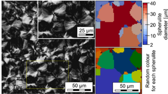
Fig. 17. Comparison of the spherulite diameter in the core area of section S2. To distinguish the different spherulites a random color has been assigned to each one, which is shown in the bottom right.
