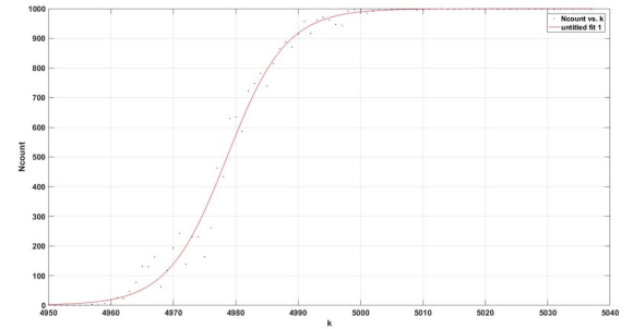
Figure 4: S-Shape Curve vs. Input Charge @ fixed threshold.
