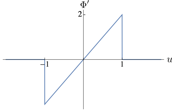
FIGURE 2. Approximation the the source term \Phi in Eq.(4.1) with u^* = 1 and \epsilon = 10^{-4} .
