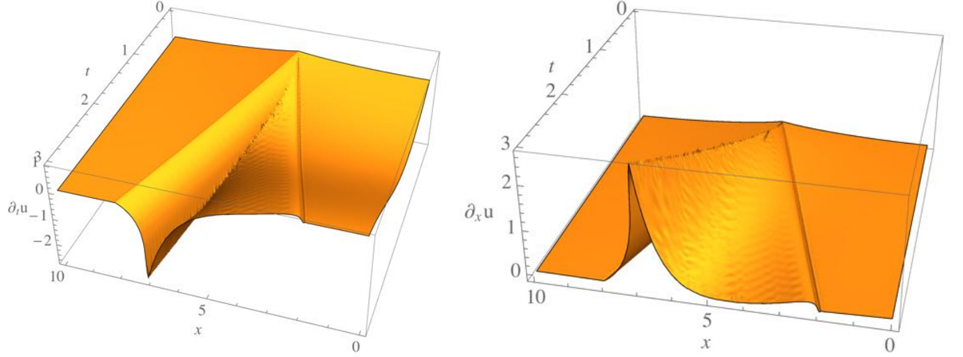
FIGURE 14. Left: derivative with respect to time of u shown in Figure 13. Right: derivative with respect to space of u shown in Figure 13. See text for the numerical values used in the simulation.
