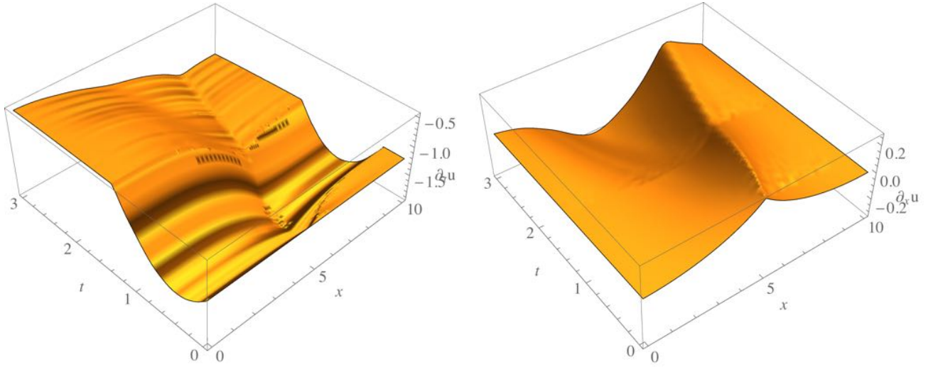
FIGURE 10. Left: derivative with respect to time of u shown in Figure 9. Right: derivative with respect to space of u shown in Figure 9. See text for the numerical values used in the simulation.
