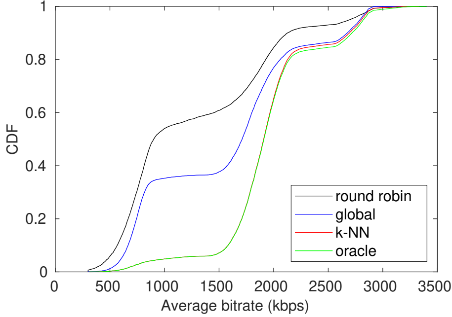
Figure 6: CDF of the Average Bitrate AB .
