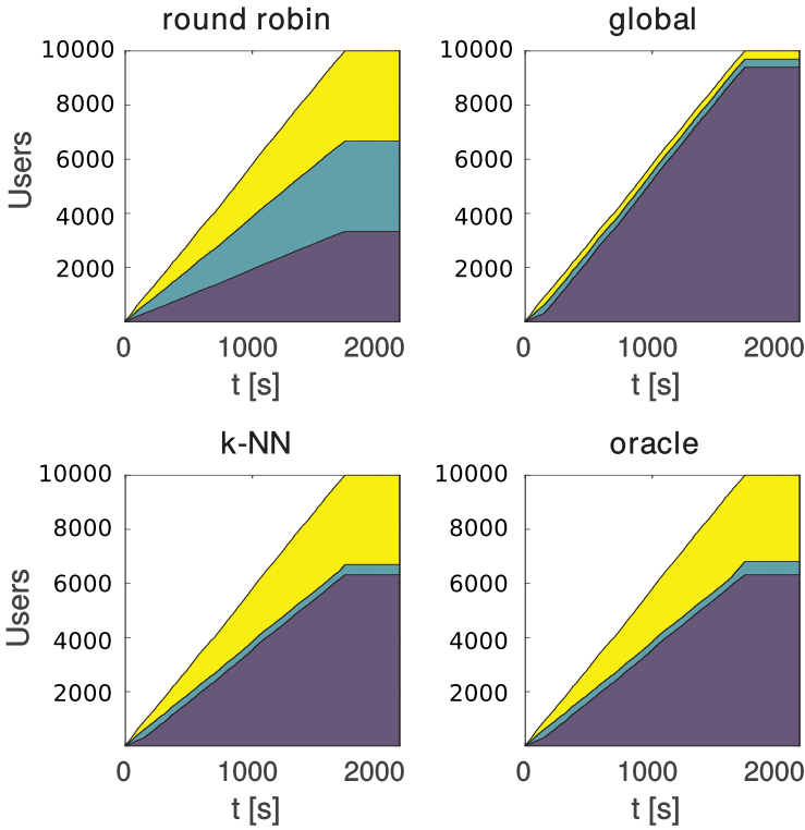
Figure 4: Evolution over time of the CDN assignment.
