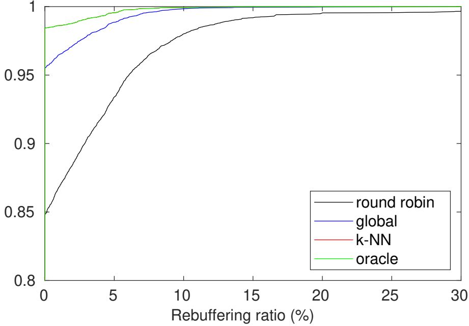
Figure 5: CDFs of the Rebuffering Ratio RR .
