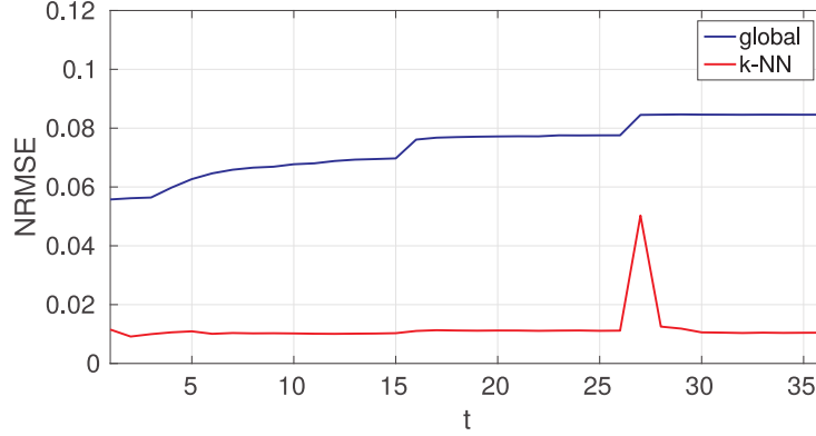
Figure 3: NRMSE for the assignment algorithms based on QoE prediction, k -NN and global .
