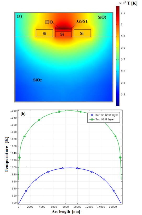
Fig. 13. (a) Temperature distribution in the plane cross section placed at the middle of the O-PCM length in the case of 2 \times 2 optical switch. (b) Temperature profile as a function of the longitudinal coordinate at the top and bottom O-PCM layer surface
