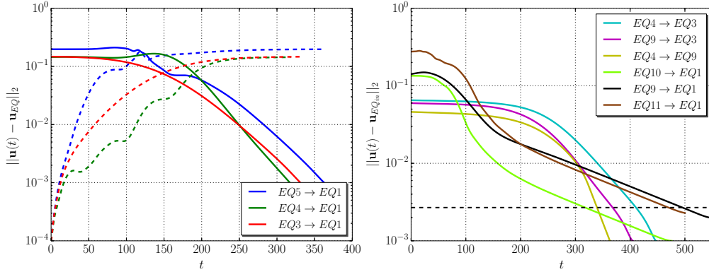
FIGURE 2. Left: Distances of the velocity field \mathbf{u}(t) to the final equilibrium \mathbf{u}_{EQ_{in}} (continuous line) and to the initial one \mathbf{u}_{EQ_{out}} (dashed line) along three heteroclinic connections found by Halcrow et al. (2009) versus time. Right: Distances to the final equilibrium \mathbf{u}_{EQ_{in}} for the new computed heteroclinic connections (continuous lines). The dashed line represents the highest residual value for the heteroclinic connections computed in Halcrow et al. (2009). The L2-norm of the considered equilibria ranges from 0.1259 to 0.4049. (Gibson et al. 2009)
