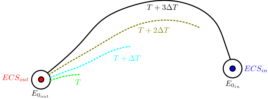
FIGURE 1. Sketch describing the CHELA algorithm: the initial condition and the related trajectory towards the final EQ change after updating the time T (dashed lines). The algorithm stops when T is sufficiently large to lead the flow field close enough to the final state (solid line).
