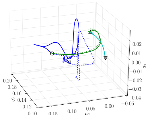
FIGURE 4. State space projection (Gibson et al. 2008) of the orbit connecting EQ5 \rightarrow EQ1 (blue) and EQ4 \rightarrow EQ1 (green), for which the dimension of the intersection is 3 and 2 respectively. For a specific connection, changing the energy shell around the initial equilibrium from E_{0_{out}} = 10^{-6} (solid line) to E_{0_{out}} = 10^{-8} (dashed line) results in finding different orbits. For those connections for which the dimension of the intersection is one, g. e. EQ4 \rightarrow EQ3 (cyan), the algorithm finds the only existing connection.
