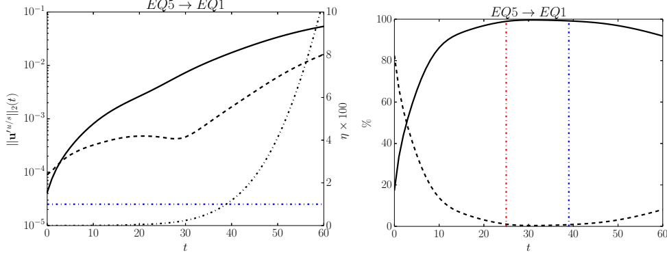
FIGURE 3. Time-evolution of contributions in the stable and unstable subspaces of EQ_{out} during the initial part of the trajectory EQ5 \rightarrow EQ1 . Left: L2-norms \|\mathbf{u}'^{s/u}\|_2 of the projections onto the unstable ( \mathbf{u}'^u , solid line) and stable ( \mathbf{u}'^s , dashed line) subspace. The difference between the linearised and the full nonlinear evolution \eta = \frac{\|\mathbf{u}'_{lin}(t) - \mathbf{u}'(t)\|_2^2}{\|\mathbf{u}'_{lin}(t)\|_2^2} (dotted line, right axis) characterizes the deviation of the invariant manifolds from the approximating linear subspaces due to manifold curvature in the direction of the trajectory. Right: Relative contribution measured in terms of relative energy in the unstable (solid line) and stable (dashed line) subspace. Vertical red dotted lines indicates when the relative contribution of the stable subspace E^s(t)/E(t) drops below 1%. Vertical blue dotted line indicates when the difference between the linearised and the full nonlinear evolution \eta reaches 1%
