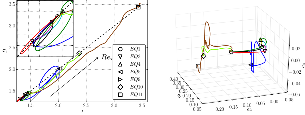
FIGURE 5. Left: Projection of the heteroclinic connections onto the energy input, I , and the dissipation rate, D , normalized by their value in the laminar flow. Right: State-space projection onto the 3D orthonormal basis \mathbf{a}_{1,2,3} of all the computed heteroclinic connections. Colours are the same as in figure 2.
