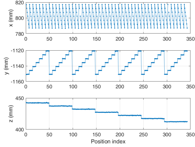
236 Fig. 8 Estimated positions at about 0.6 m from FG, as a function of index i.
