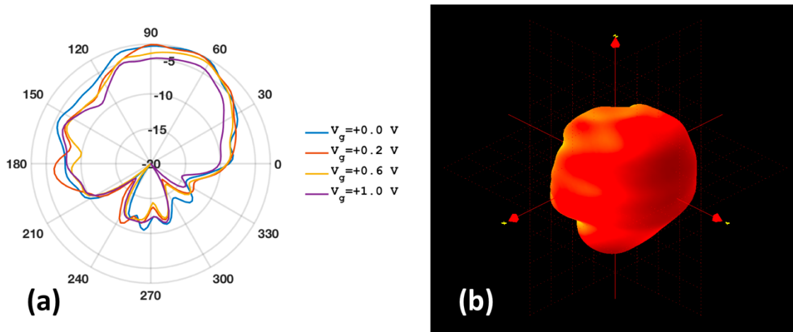
Figure 5: (a) Radiation pattern in the xz -plane ( \phi=90^\circ ), at 1.55 GHz when the gate voltage is varied. The tilt in the patterns is also evident in the unloaded GPS antenna. (b) Experimental 3D radiation pattern at V_g=0 V.
