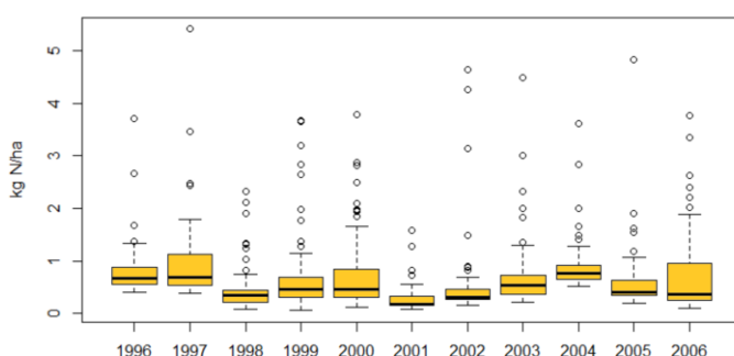
Figure 6. DIN load ( \text{kg ha}^{-1} ) estimated by SWAT for the HRUs under durum wheat production. The horizontal line within the boxplot indicates the median, the boundaries of the box indicate the 25 th and 75 th percentiles and the whiskers indicate the 1 st and 99 th percentiles of the values.
