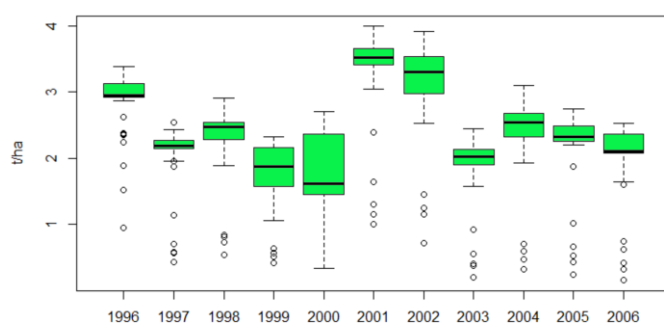
Figure 5. Yield ( \text{t ha}^{-1} ) estimated by SWAT for all the HRUs under durum wheat production. The horizontal line in the boxplot indicates the median, the boundaries of the box indicate the 25 th and 75 th percentiles and the whiskers indicate the 1 st and 99 th percentiles of the values.
