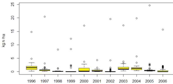
Figure 8. \text{NO}_3\text{-N} load ( \text{kg ha}^{-1} ) leaching from the soil into the groundwater estimated by SWAT for the HRUs under durum wheat production. The horizontal line within the boxplot indicates the median, the boundaries of the box indicate the 25 th and 75 th percentiles and the whiskers indicate the 1 st and 99 th percentiles of the values.
