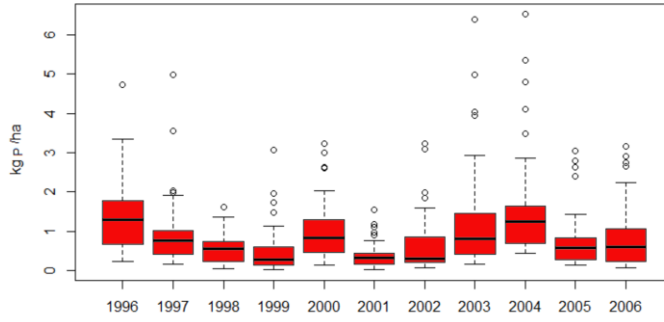
Figure 7. TP load ( \text{kg ha}^{-1} ) estimated by SWAT for the HRUs under durum wheat production. The horizontal line within the boxplot indicates the median, the boundaries of the box indicate the 25 th and 75 th percentiles and the whiskers indicate the 1 st and 99 th percentiles of the values.
