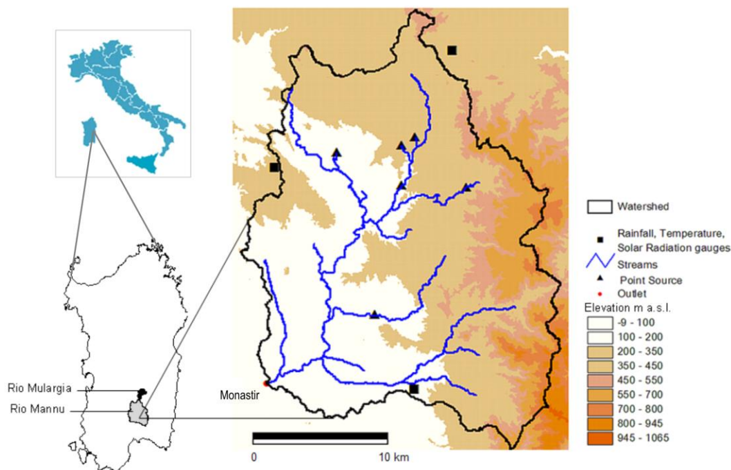
118 119 Figure 1. Study area: Rio Mannu River Basin (Sardinia, Italy).
