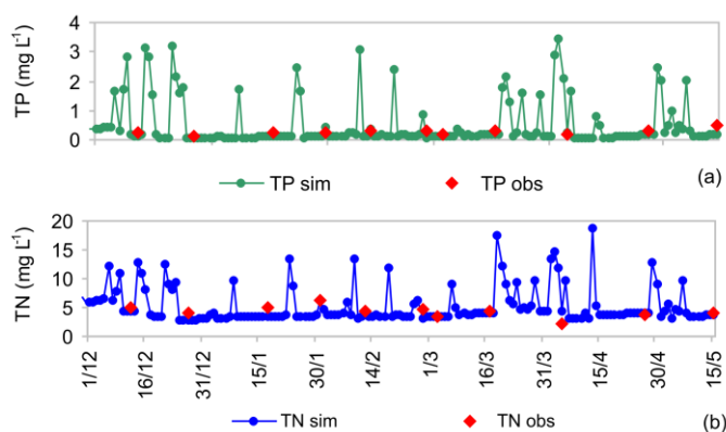
Figure 4. Simulated and observed concentrations of total phosphorus (TP) and total nitrogen (TN) at the outlet (Monastir).
