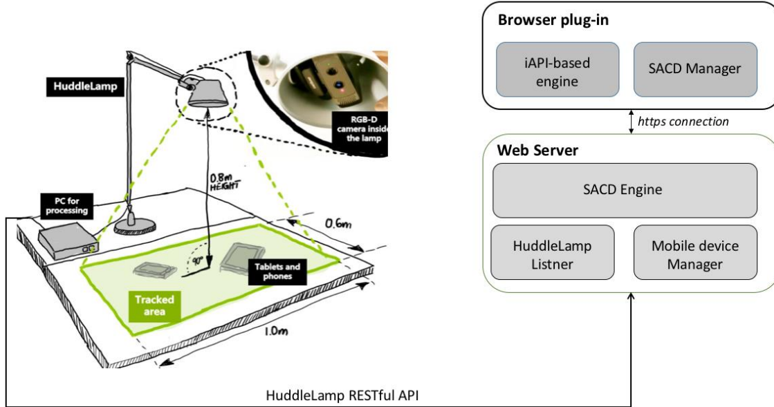
Figure 6. Overview of the final system including hardware and software modules
