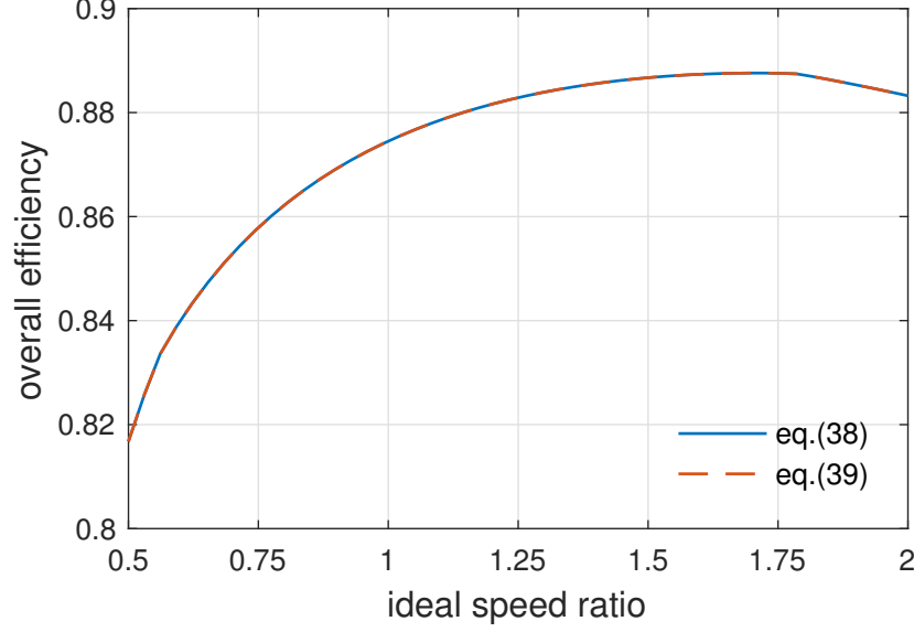
Figure 11. Overall efficiency of the transmission vs ideal speed ratio. The efficiency values are calculated by the eq. (38) and by the eq. (39) for comparison. F_{N0} = 2.0 \text{ kN}
