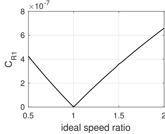
Figure 12. Creep coefficient on the single-idler as a function of speed ratio. F_{N0} = 2.0 \text{ kN}
