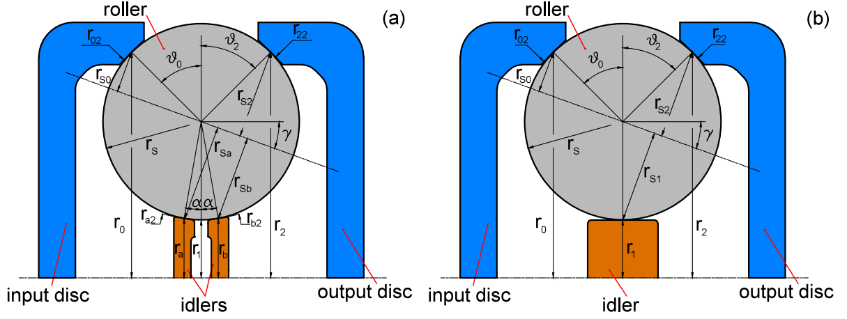
Figure 2. Schematic picture of the variator and related geometrical quantities for double-idler (a) and single-idler (b) geometries.
