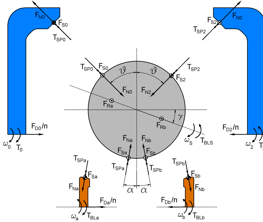
Figure 6. Free-body diagrams of the transmission parts. Single arrows are forces, double arrows are torques.
