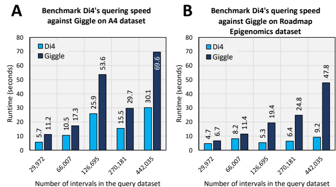
Fig. 7: The runtime plotted here is the average of 10 executions of each query. The results show that Di4 runs up to 3× faster than Giggie on a large dataset (panel A), and up to 6× faster on a small dataset (panel B).
