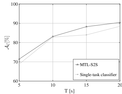
Fig. 14. Classification performance with six application classes.
