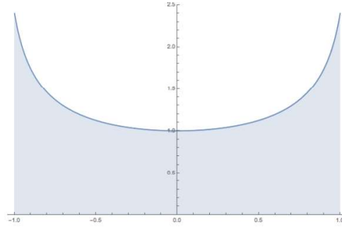
Figure 5. Representation of the self-weight projected on the horizontal plane for a barrel vault.
