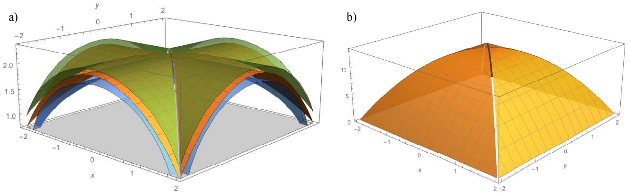
Figure 14. Estimation of the Geometrical Factor of Safety: (a) the unilateral membrane f entirely contained between intrados and extrados surfaces of the vault; (b) the dual Airy stress function F .
