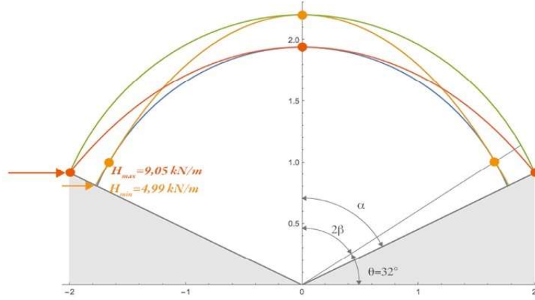
Figure 11. Minimum thrust (yellow) and maximum thrust (red) solutions in a section of the case study vault.
