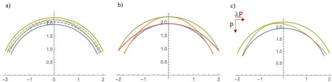
Figure 4. Objective functions: (a) Estimation of the Geometrical Factor of Safety; (b) Determination of the maximum and minimum thrust solutions; (c) lower bound estimation of the collapse multiplier \lambda_c of a generic live load condition.
