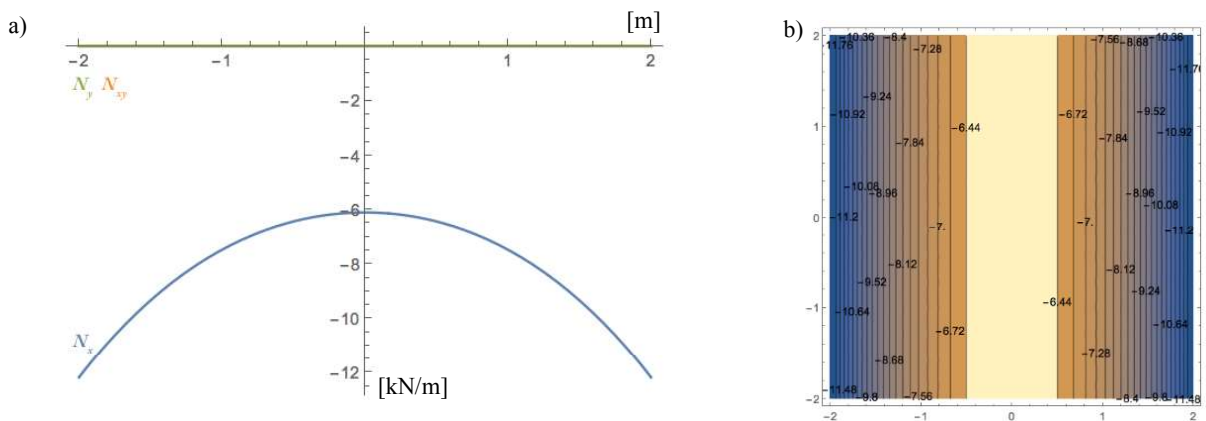
Figure 9. Admissible stress field corresponding to maximum GFS: (a) entity of N_x , N_y and N_{xy} [kN/m] in a generic section of the vault; (b) distribution of N_x [kN/m].
