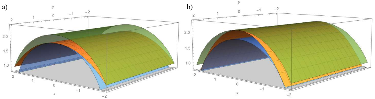
Figure 10. (a) Maximum thrust solution; (b) minimum thrust solution
