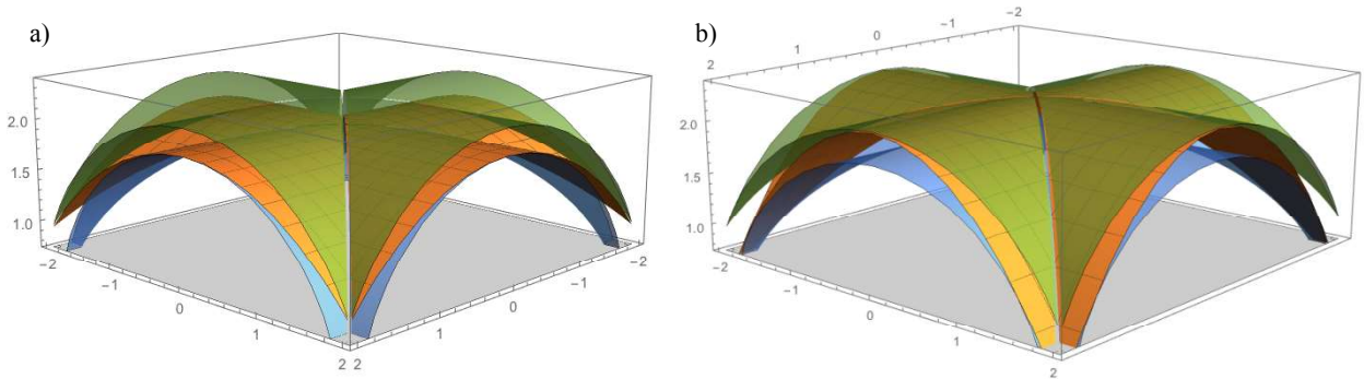
Figure 18. (a) Maximum thrust solution; (b) minimum thrust solution.
