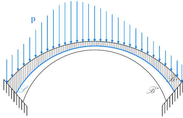
Figure 1. Scheme of a generic cross section of a vault [38]
