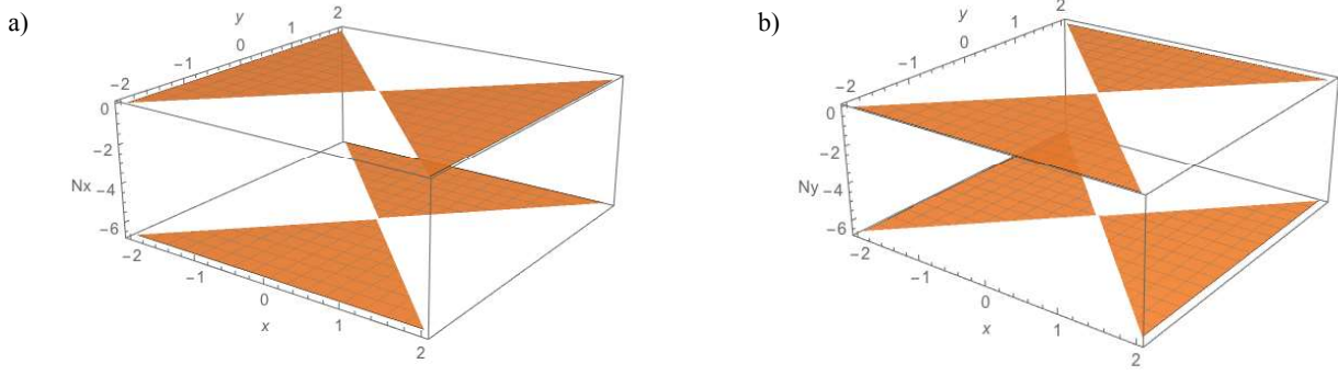
Figure 15. Projected membrane stresses on the horizontal plane: (a) \bar{N}_x [kN/m]; (b) \bar{N}_y [kN/m].
