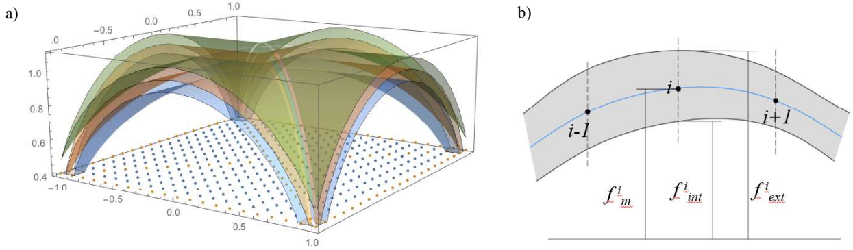
Figure 3. (a) Intrados, extrados and middle surfaces of the vault (in blue, green and orange, respectively); (b) Input data associated to each point P_{ij} of \mathcal{P} .
