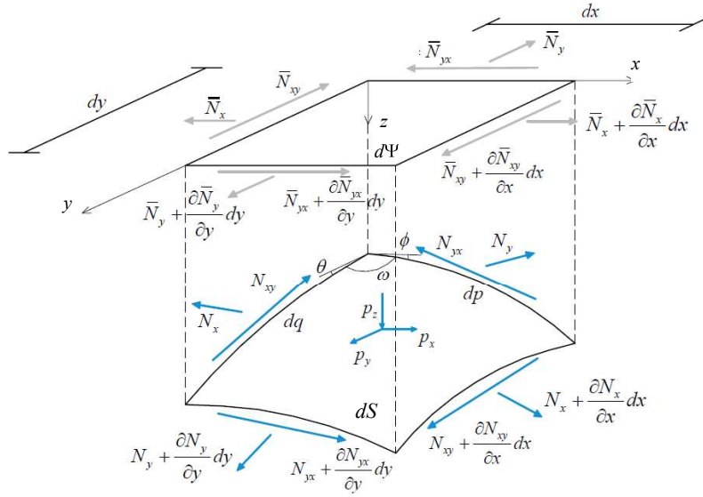
Figure 2. Equilibrium of an infinitesimal element of the membrane dS ; the edges dp and dq project in the (x,y) plane into dx and dy , respectively.
