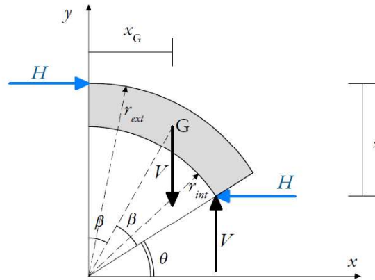
Figure 19. Scheme for the analytical expression of the minimum thrust for an arch having a segmental profile [4]
