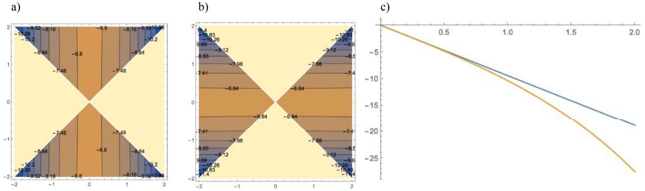
Figure 16. Admissible stress field for the case study cross vault: (a) distribution of N_x [kN/m]; (b) distribution of N_y [kN/m]; (c) projected axial force N [kN] along the diagonals (in blue) and actual axial force along the fold (in orange).
