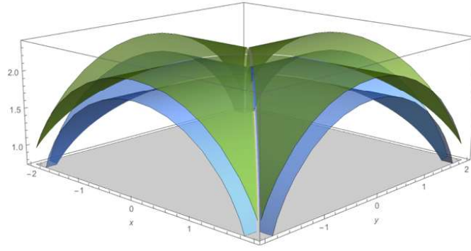
Figure 12. Intrados and extrados surfaces of the vault
