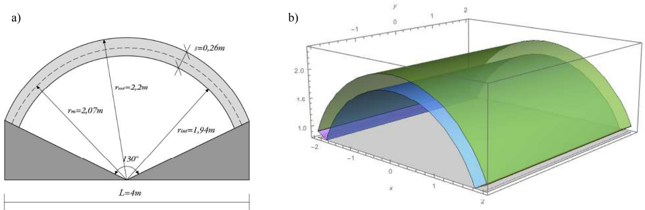
Figure 6. Geometrical description of the studied barrel vault: (a) section of the vault; (b) intrados and extrados surfaces of the vault
