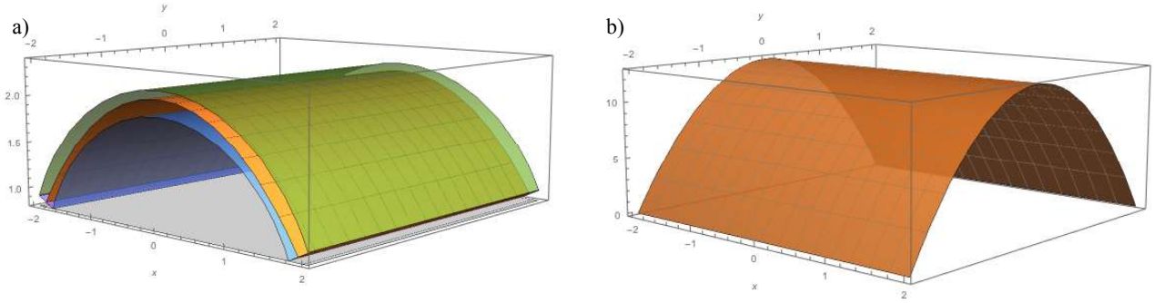
Figure 7. Estimation of the Geometrical Factor of Safety: (a) the unilateral membrane f ; (b) the Airy stress function F .
