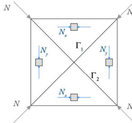
Figure 17. Scheme of the mechanical behavior of the cross vault subject to the self-weight
