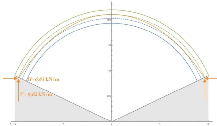
Figure 8. Generic cross section of the vault, entity of the GFS and corresponding horizontal and vertical reactions at supports.
