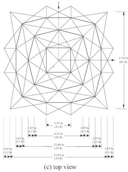
Fig. 4. Schematic of the spatial 942-bar tower.
