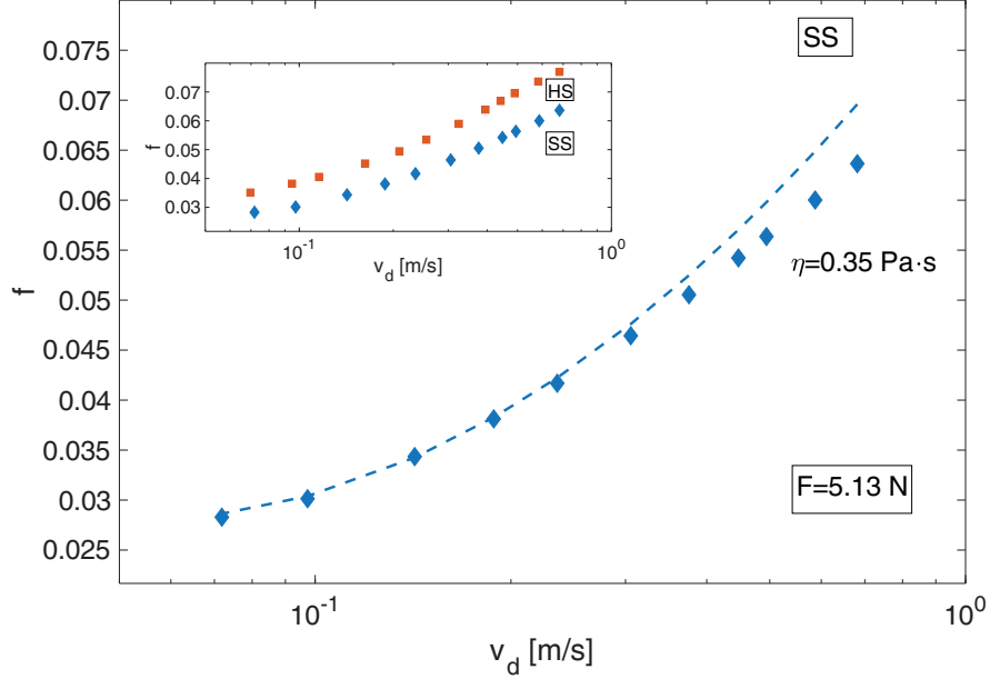
Figure 10: Friction coefficient as a function of the disk speed u_d for different values of viscosity \eta and for a normal load equal to F_n = 5.13 \text{ N} . Data in the main plot refer to the soft on soft configuration, i.e., to the contact of a NBR ball with a NBR layer. In the inset, we compare the experimental data in the such a configuration with the hard on soft case. Dotted lines show numerical results, whereas points are the experimental outcomes.
