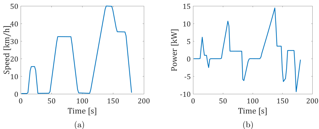
Figure A.3: Speeds (a) and power (b) of a vehicle during a ECE-15 urban cycle [129].
