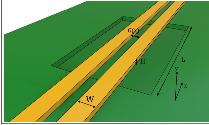
Figure 2.11: Structure of the optomechanical device [47].
