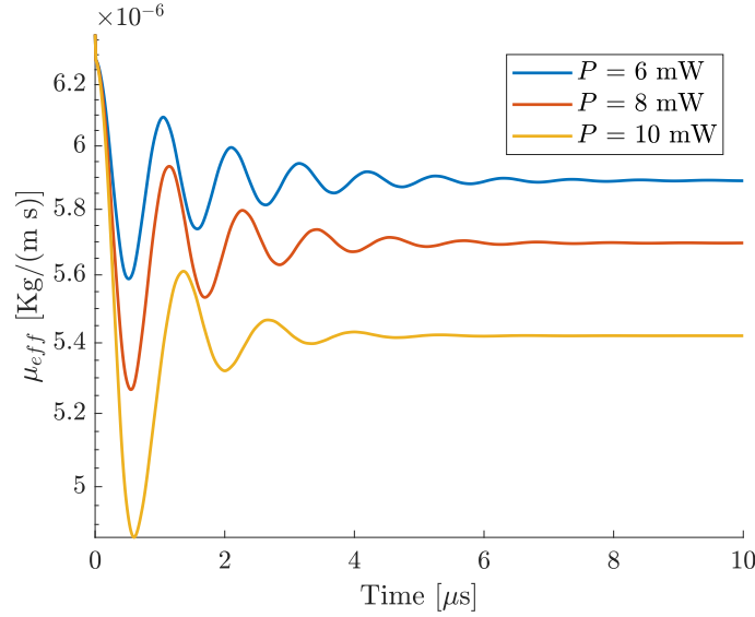
Figure 2.15: The value of \mu_{eff} as a function of time, during the settling of the silicon waveguides [47].
