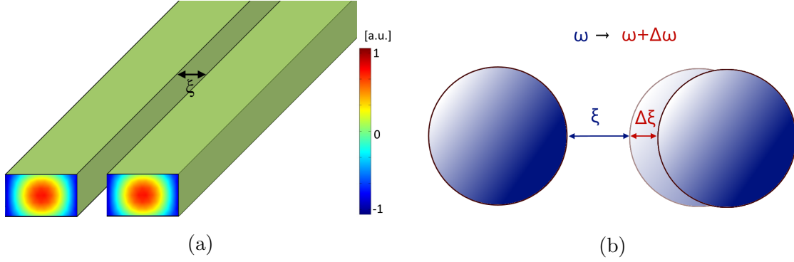
Figure 2.2: Systems of coupled waveguides (a). Closed system of two coupled resonators (b).
