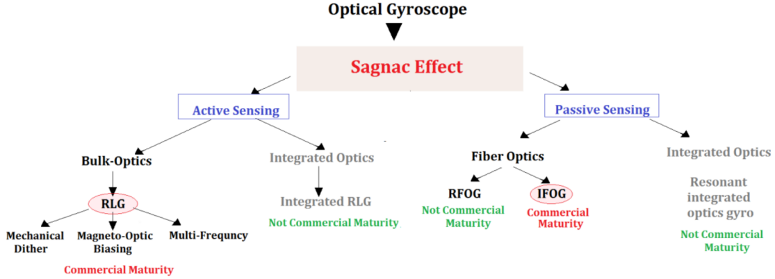
Figure 1.1: Classes of optical gyroscopes [2]
