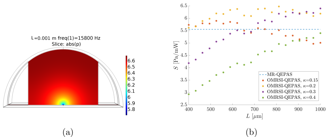
Figure 3.7: Pressure signal (Pa) per input power of 1 mW over a central cross section in OMRSI-QEPAS (a) and Pressure signal per input power ( S ) as a function of the length of the waveguide in OMRSI-QEPAS, compared with MR-QEPAS (b) [62].
