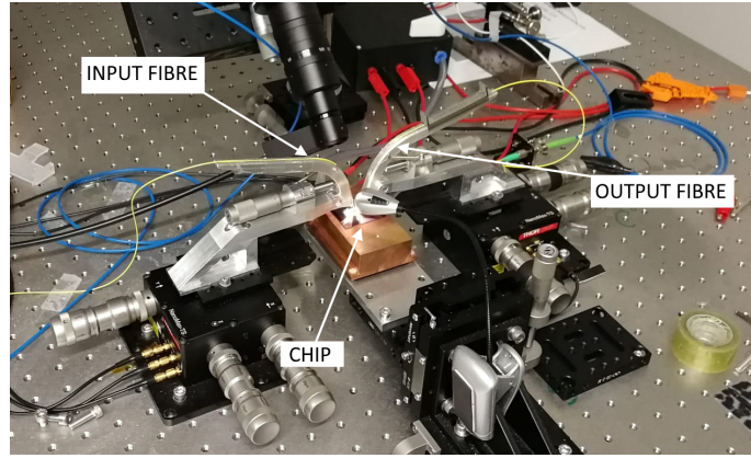
Figure 2.32: Photo of the experimental setup for the measurement. In the picture the two fibres are visible, together with a moveable stage where the integrated chip is fixed.
