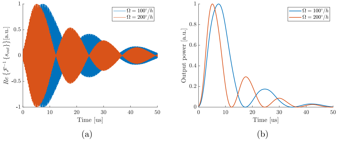
Figure 1.20: (a) Normalized real part of the output signal s_{out} in the time domain. (b) Normalized |s_{out}|^2 in the time domain, representing the average optical power at the photoreceiver.
