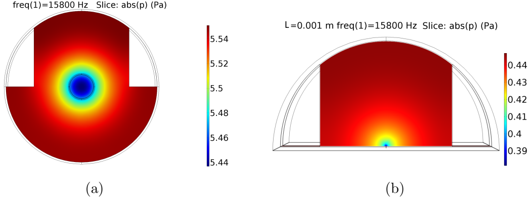
Figure 3.4: Acoustic pressure field (Pa), with optical power of 1mW without resonators in the MR-QEPAS configuration (a) and MRSI-QEPAS configuration (b) [62].
