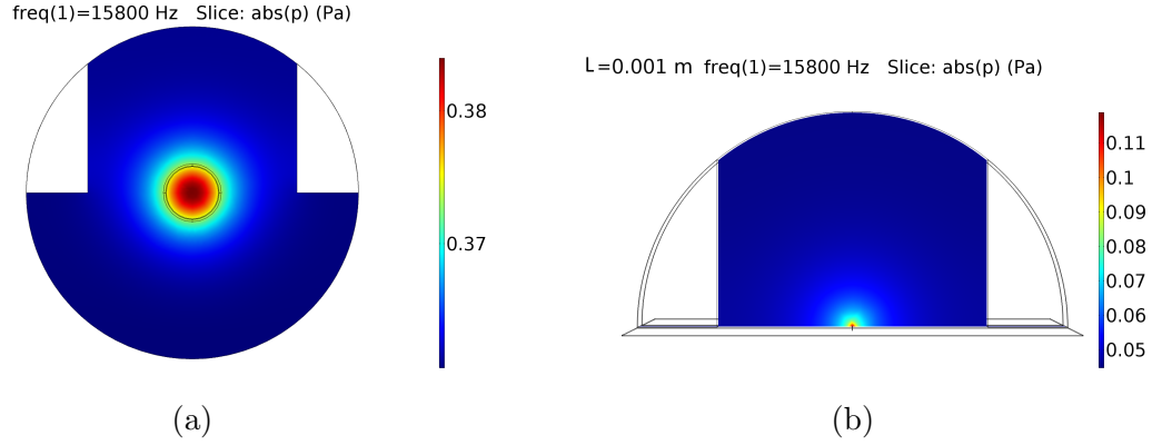
Figure 3.3: Acoustic pressure field (Pa), with optical power of 1mW without resonators in FS-QEPAS configuration (a) and SI-QEPAS configuration (b) [62].
