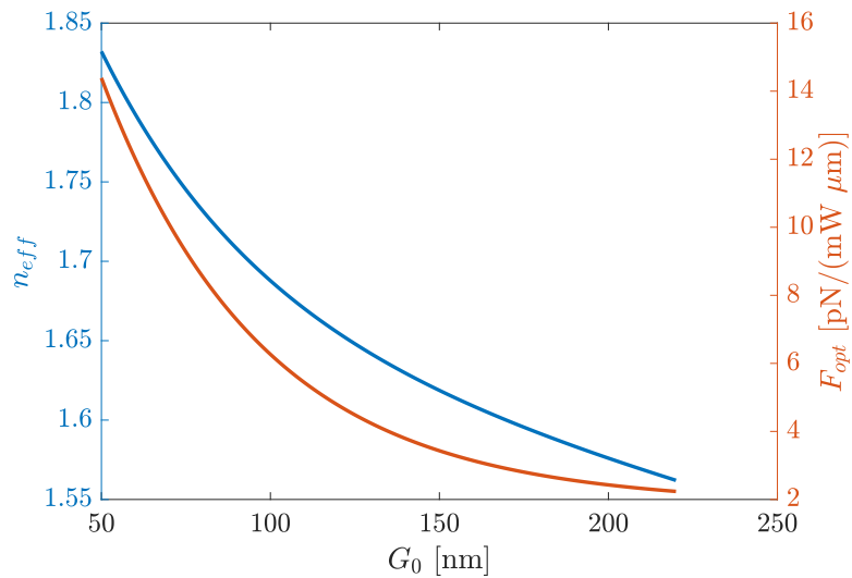
Figure 2.13: Effective index of the symmetric supermode (left y-axis) and optical attractive force (right y-axis) as a function of the initial gap G_0 [47].
