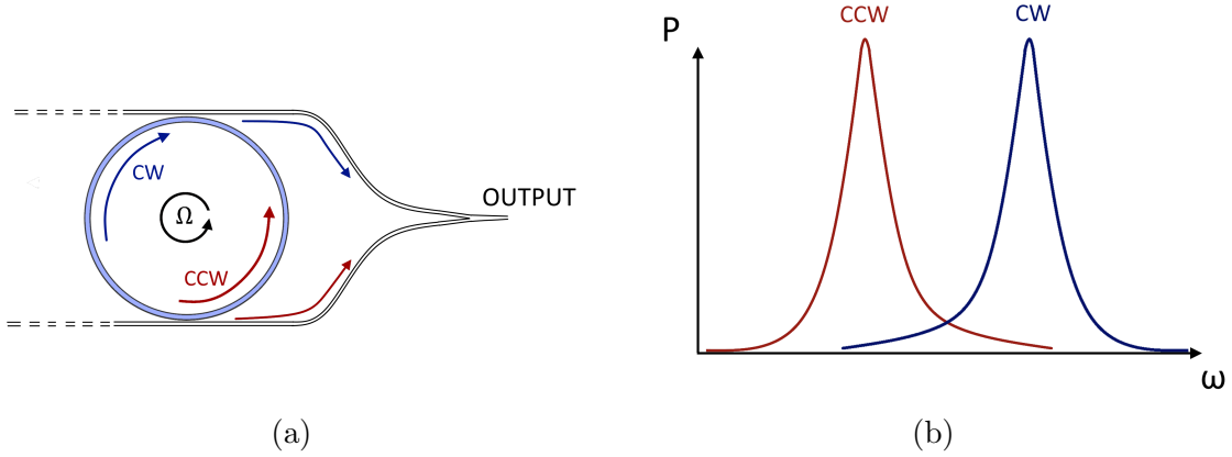
Figure 1.3: Structure of a resonant ring Sagnac gyroscope (a). Resonance peaks of the CCW and CW waves during rotation. (b).
