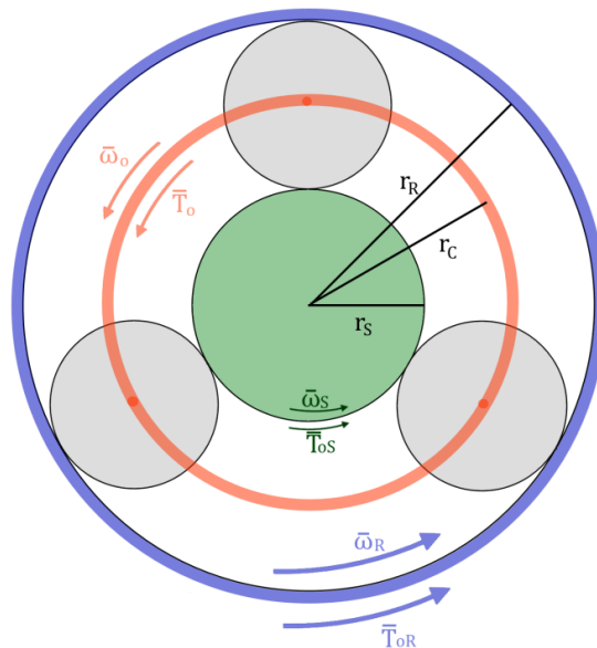
Figure A.1: Schematic of a classical planetary gear [129].
