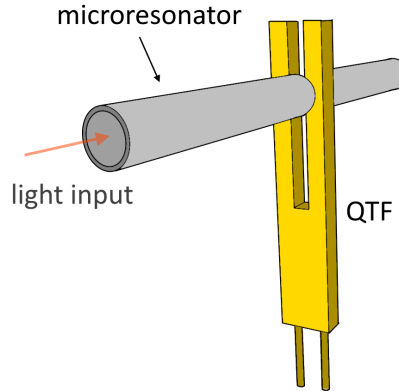
Figure 4: Acoustic Detection Module (ADM).
