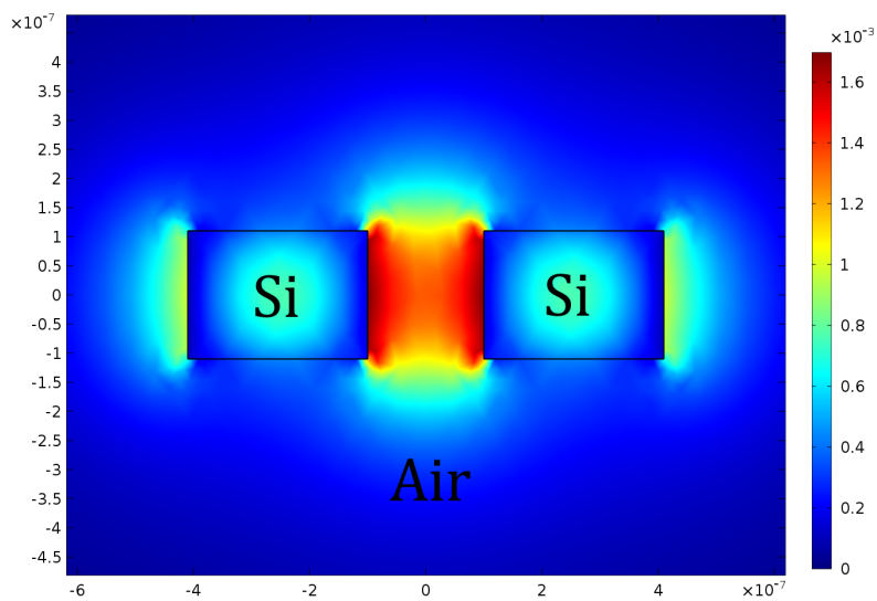
Figure 2.12: Squared norm of electric field of the symmetric mode in the coupled waveguides [47].
