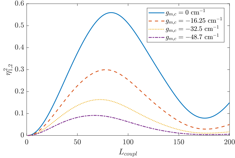
Figure 1.18: Coupling efficiency \eta_{1,2} for different values of the material gain of the InGaAsP region, corresponding to the carrier density N marked in Figure 1.17b.
