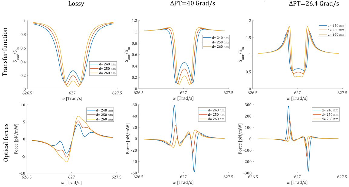
Figure 2.7: Transfer function and optical forces (normalized to the input optical power) as a function of the angular frequency for different gap d between the straight arms of the racetracks, in case of lossy resonators (left) and in case of \Delta PT equal to 40 Grad/s (center) and 26.4 Grad/s (right) ( \gamma_1 - \gamma_2 equal to 2 Grad/s). Approaching the Parity-Time condition, the forces change their sign with respect to the lossy case [46].
