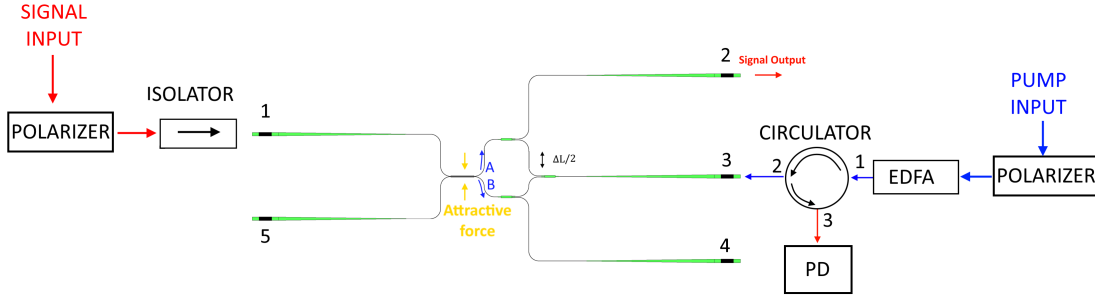
Figure 2.31: Conceptual setup for experimental measurement.
