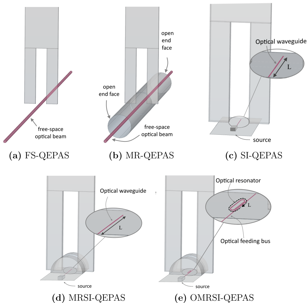
Figure 3.1: Different configurations of QEPAS setups analysed in this work. FS-QEPAS (a) is a simple QEPAS configuration without any mechanical resonator. MR-QEPAS (b) is a free space configuration with a mechanical resonator. SI-QEPAS (c) is a semi-integrated version of QEPAS without mechanical resonators. MRSI-QEPAS (d) is a semi-integrated version of QEPAS with a mechanical resonator. OMRSI-QEPAS (e) is a semi integrated version of QEPAS with a mechanical resonator and an optical resonator (fed by an optical bus). [62]
