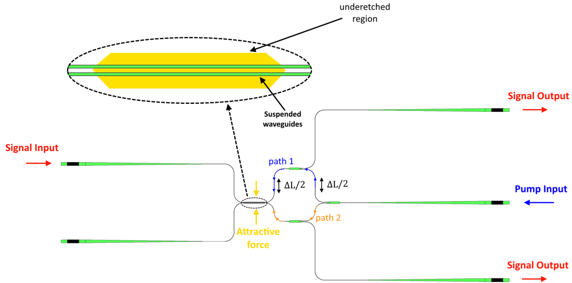
Figure 2.22: Design of the optomechanical switch
