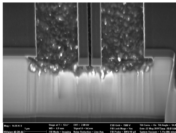
Figure 2.24: Test suspended waveguides after vapor HF
