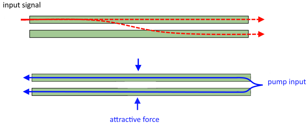
Figure 2.21: Working principle of the switch. The pump input excites an attractive force and the input signal is directed to one of the output ports.
