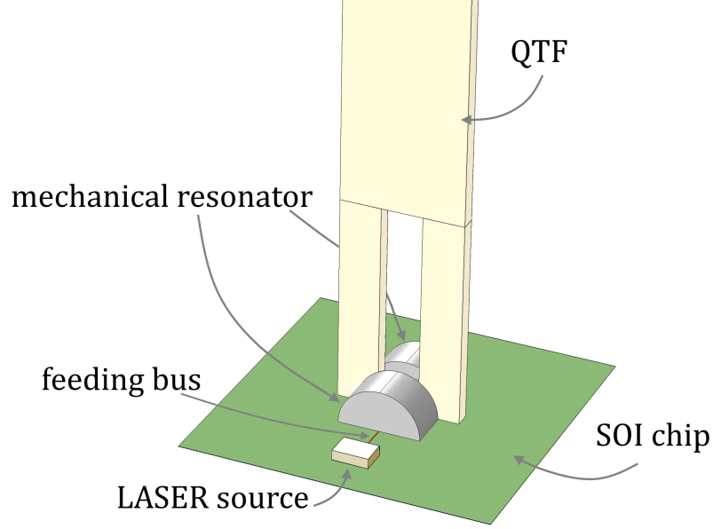
Figure 3.8: Final configuration of the OMRSI-QEPAS setup [62].
