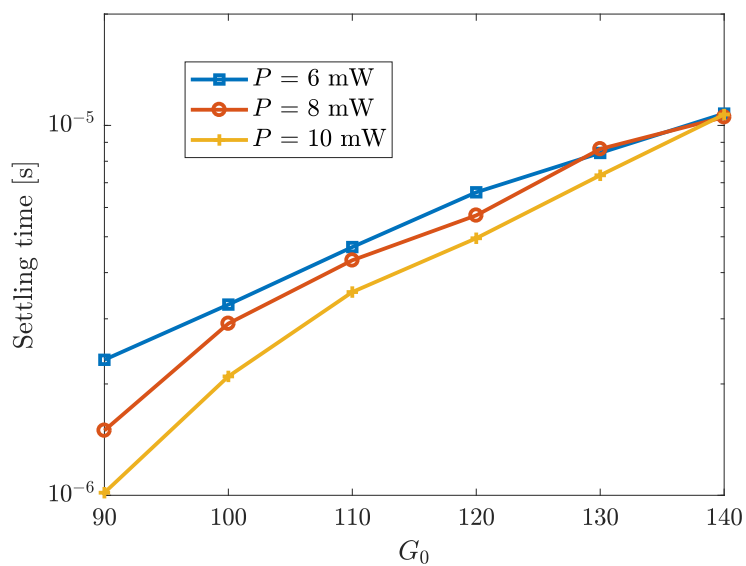
Figure 2.17: Settling time t_s as a function of initial gap G_0 .
