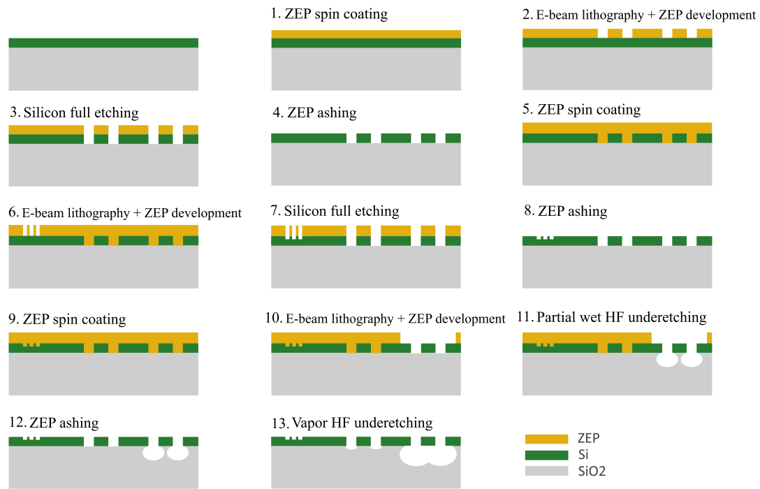
Figure 2.26: Process flow with strip design
