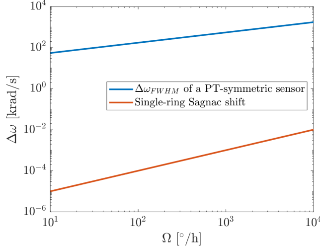
Figure 1.11: Full width at half maximum of the designed PT-symmetric gyroscope as a function of the angular velocity (on a log-log graph) compared with the classical Sagnac spectral shift on a gyroscope with a single ring with the same radius.
