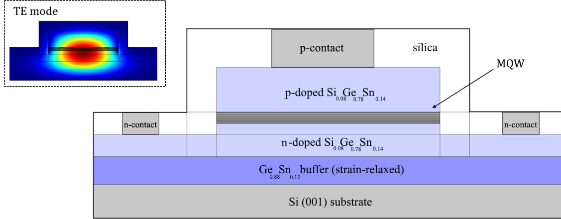
Figure 1.9: Waveguide cross-section: structure design. Inset: TE optical field [12].
