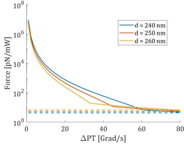
Figure 2.8: Optical maximum force as a function of the parameter \Delta PT for different values of the distance d . Dashed lines represent the peak of the optical forces in the case of lossy cavities. The discontinuity in the first derivative of the function is due to the changing of the sign of the force [46].
