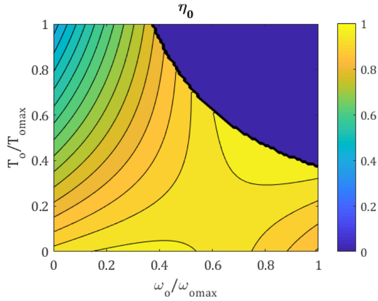
Figure A.5: Efficiency map of a standard electric motor [129].
