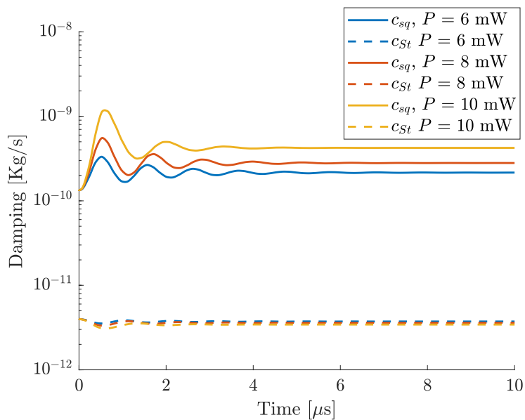
Figure 2.16: Damping coefficients (due to laminar drag and squeezing effect): time evolution.
