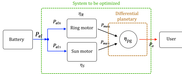
Figure A.2: Schematic of the system to be optimized: power flow with both motors supplying power [129].
