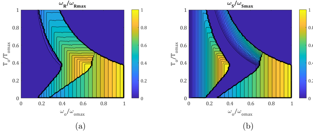
Figure A.9: Speed of the motor of the ring (a) and the sun (b) maximizing the overall efficiency during power supply [129].
