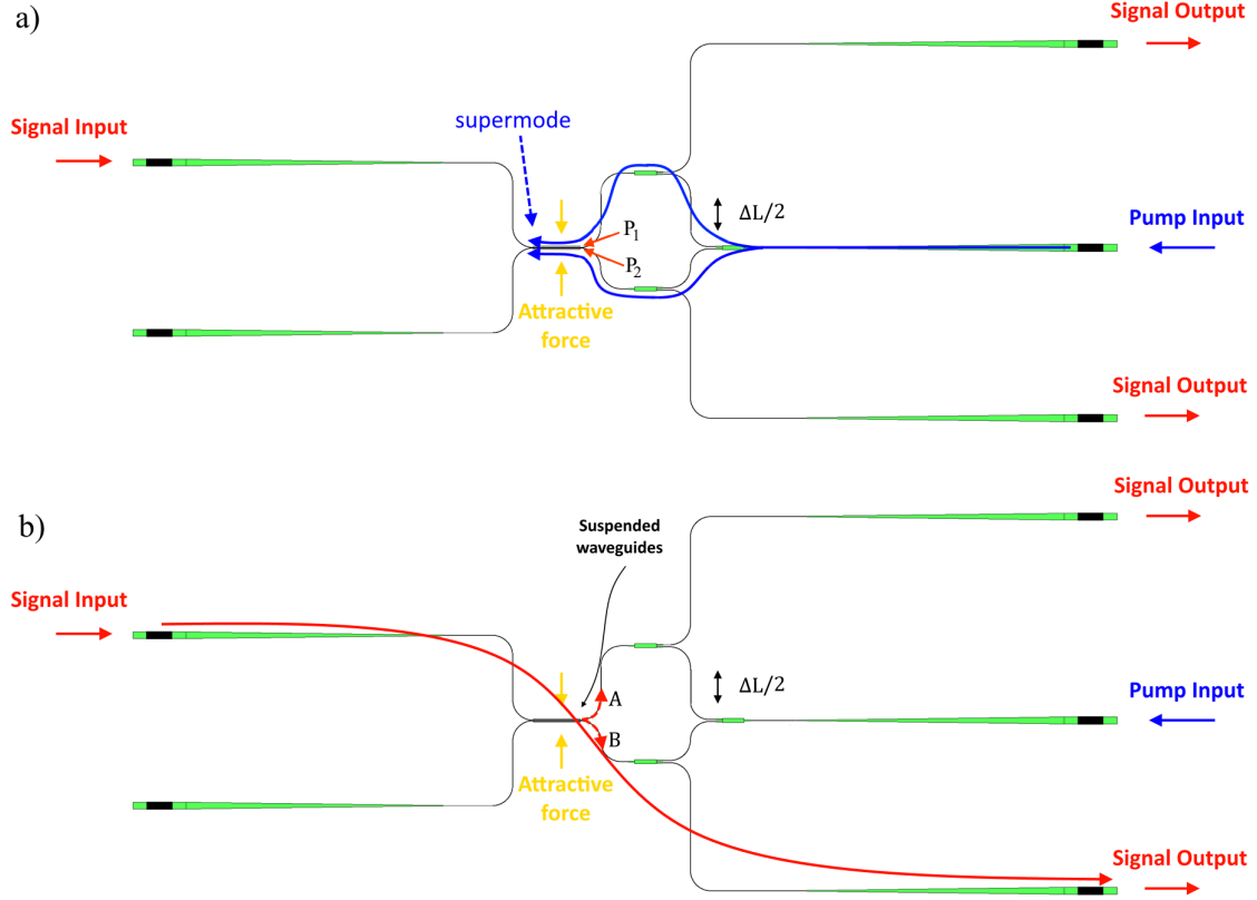
Figure 2.23: Working principle of the optomechanical switch. The pump input power in (a) is divided in two paths with an optical path difference \Delta L n_{eff} . Depending on the wavelength of the pump input, a symmetric or antisymmetric supermode (or a combination of both) can be excited in A and B, thus exciting optical forces. So, the input signal power coupled fraction can be controlled (b).
