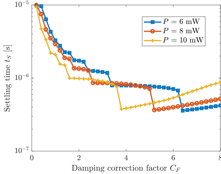
Figure 2.18: Settling time t_s as a function of the damping coefficient [47].
