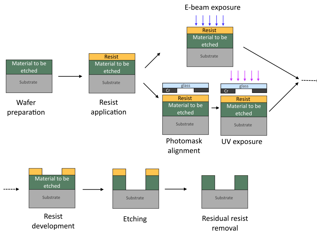
Figure 5: Microfabrication processes of integrated devices including lithography and etching.
