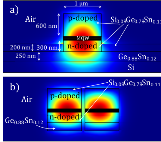
Figure 2.5: Field E_y in the cross section of the fixed part of each racetrack resonator [46] (a). Field E_y of the symmetrical mode in the cross section of the movable part of each racetrack resonator [46] (b).
