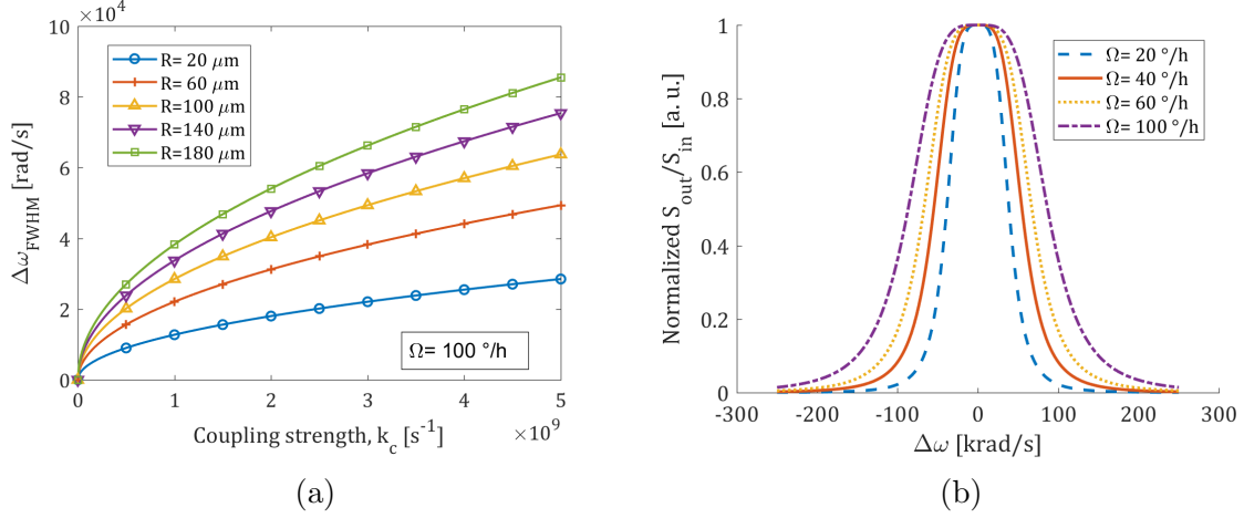
Figure 1.7: Coupling strength as a function of the full width at half maximum, at different radius sizes [12] (a). Normalized transfer function S_{\text{out}}/S_{\text{in}} at different angular velocities, with g_1 = -g_2 = 5\ \text{cm}^{-1} , \mu = 2.17 \cdot 10^5\ \text{s}^{-1/2} [12] (b).
