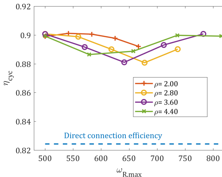
Figure A.8: \eta_{cyc} for different combinations of \rho and \omega_{maxR} [129].
