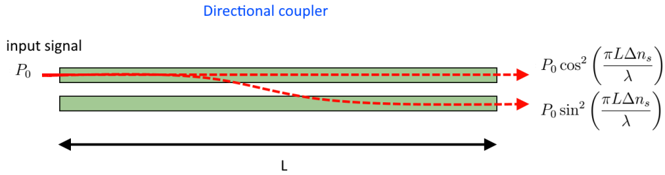
Figure 2.19: Working principle of the directional coupler.
