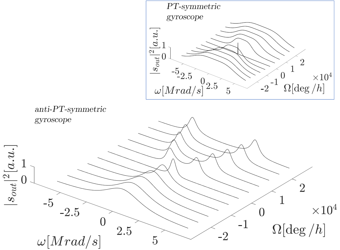
Figure 1.13: Normalized output spectrum in the proximity of the exceptional point of an anti-PT-symmetric gyroscope (with R_1 = 20 \mu\text{m} , R_2 = 19.95 \mu\text{m} and \gamma_1 = \gamma_2 = -0.5 \text{ Mrad/s} ) around \lambda = 1.55 \mu\text{m} . The inset shows the output spectrum of a PT-symmetric gyroscope (with R_1 = 20 \mu\text{m} , R_2 = 20 \mu\text{m} and \gamma_1 = -\gamma_2 = 1 \text{ Trad/s} ) [13].
