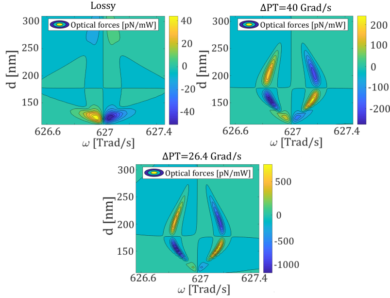
Figure 2.9: Optical forces as a function of the angular frequency for different gaps d between the straight arms of the racetracks [46].
