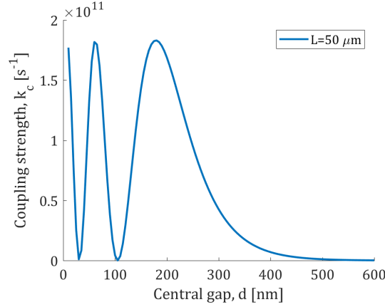
Figure 2.6: Coupling strength k_c as a function of the gap d between the edges of the suspended part of the racetracks [46].
