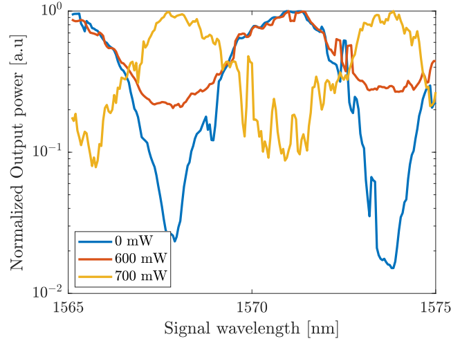
Figure 2.33: Normalized output power as a function of the wavelength of the input signal, for different amount of optical power at the pump input. The power of the mode exerting the optical force is estimated to be 20-30 times lower than than laser injected power, due to the grating couplers and the MMIs losses.
