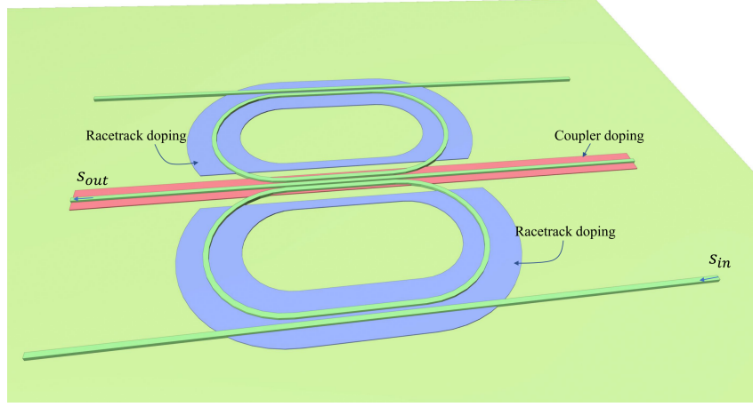
Figure 1.16: Design proposal for an optical anti-parity-time-symmetric optical gyroscope on InP platform.
