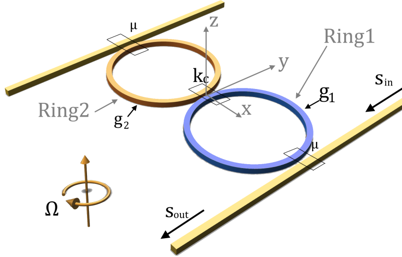
Figure 1.6: Schematic of a PT-symmetric gyroscope system [12].
