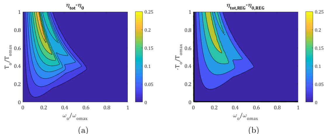
Figure A.7: Difference between the efficiency map of the optimized system and that of a single motor during power supply (a) and power regeneration (b) for \rho=3 , \omega_{maxR}=0.8\omega_{o,max} and \omega_{maxS}=1.6\omega_{o,max} [129].
