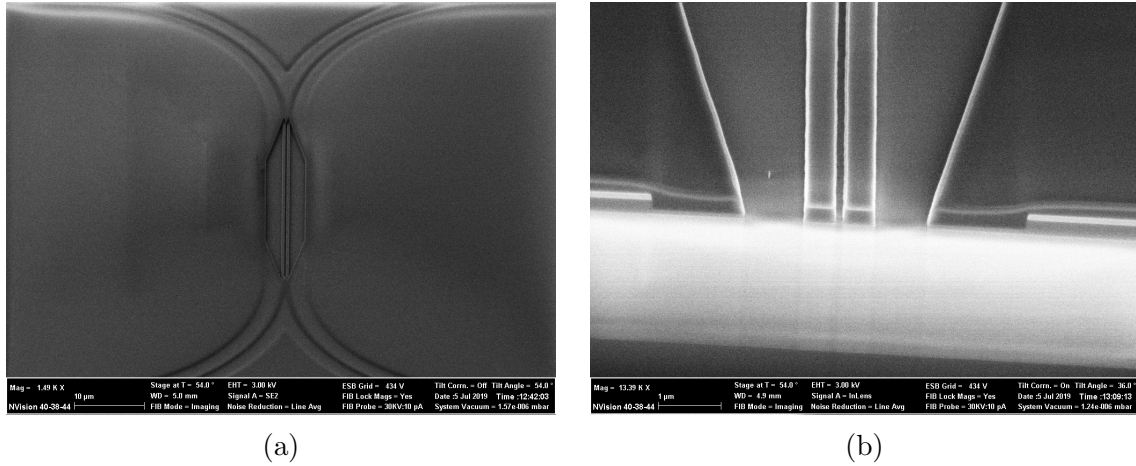
Figure 2.29: SEM pictures: cross section of suspended waveguides before the last step (Vapor HF), before (a) and after (b) FIB
