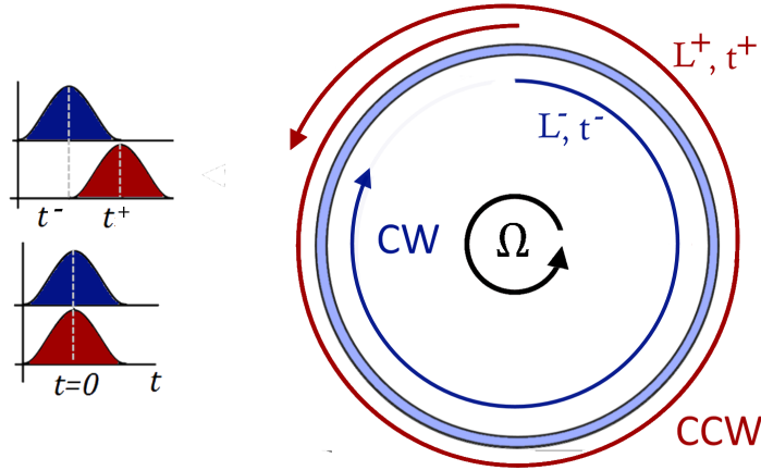
Figure 1.2: Counterpropagating beams in a ring structure, and revolution times.
