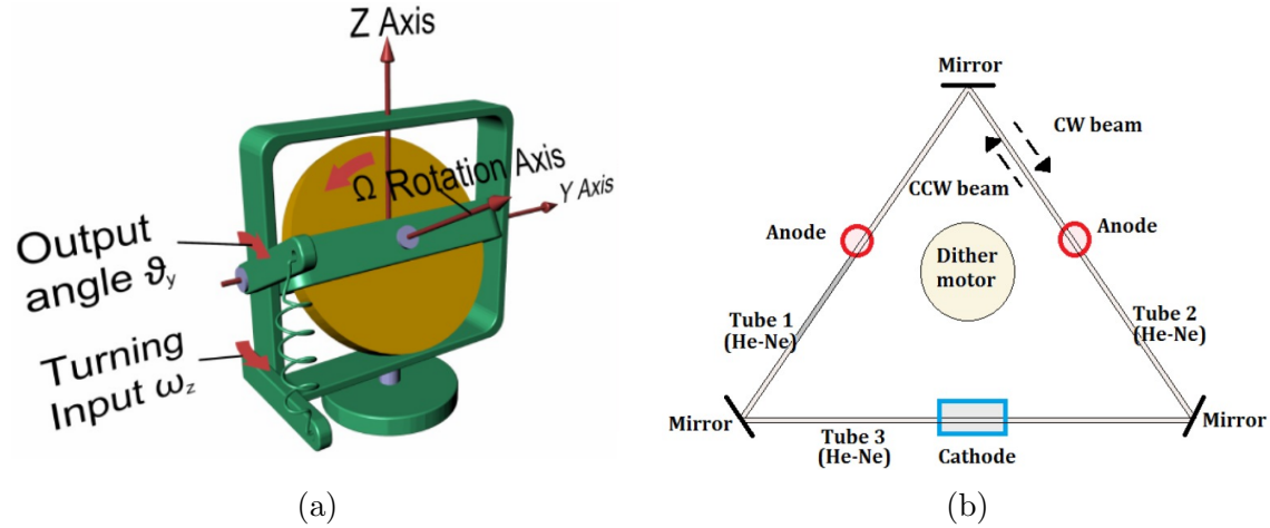
Figure 2: Spinning mass gyroscope [2] (a). Ring Laser Gyroscope [2] (b).
