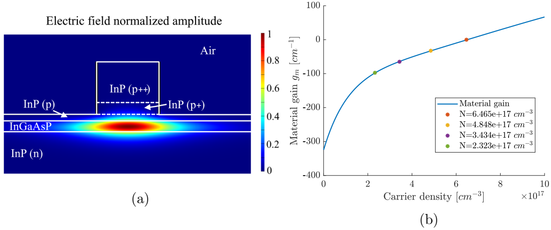
Figure 1.17: (a) Normalized electric field and cross section of the waveguide adopted in all the regions of the integrated gyroscope. (b) Material gain of InGaAsP as a function of the density of the injected carriers, obtained by halving the material gain obtained from model in [101] (to obtain the amplitude gain). The marked dots in the legend represent the values of the carrier density, used in the design of the coupler.
