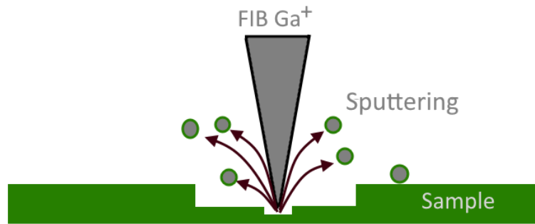
Figure 6: FIB milling process via a beam of \text{Ga}^+ ions.
