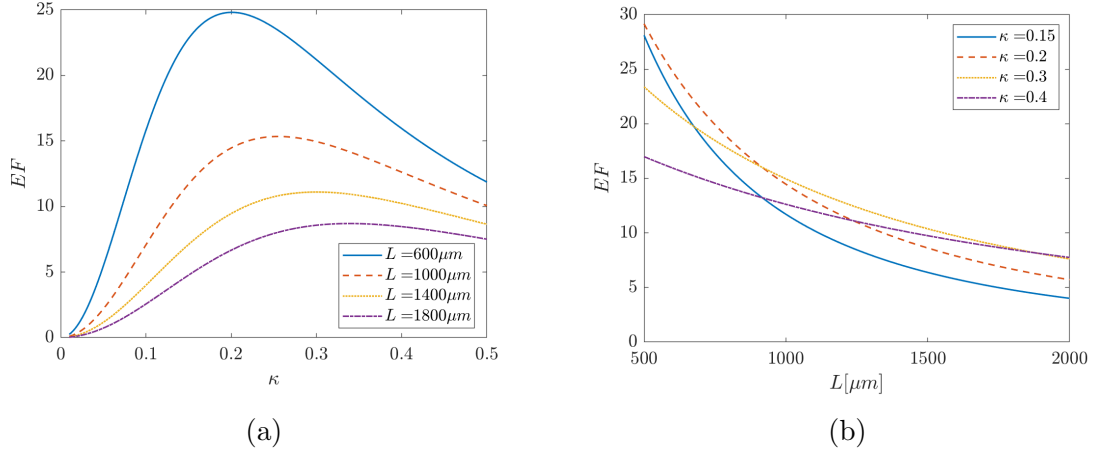
Figure 3.6: Enhancement factor as a function of \kappa for different values of L (a) and enhancement factor as a function of L for different values of \kappa , with estimated loss \alpha_{wg} = 0.69\text{dB/cm} (b) [62].
