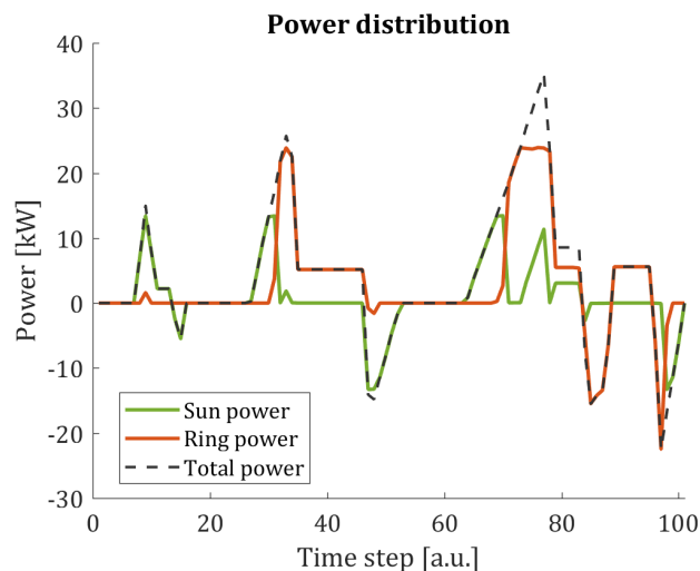
Figure A.10: Power distribution of the optimized system over the sun and the ring motors [129].
