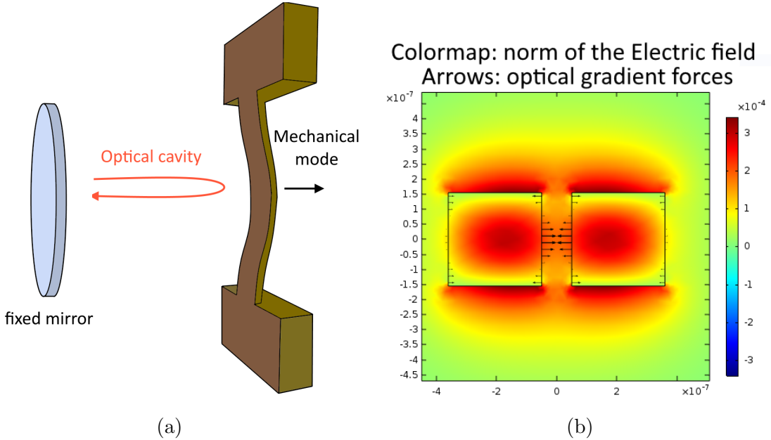
Figure 3: Classical optomechanical cavity (a). Arrow lines representing optical gradient forces evaluated through Maxwell Stress Tensor (b).
