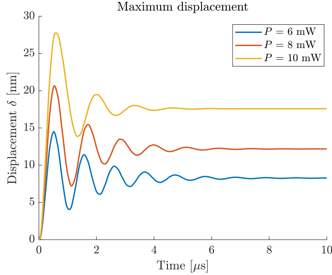
Figure 2.14: Maximum displacement as a function of time, for three different values of input power [47].
