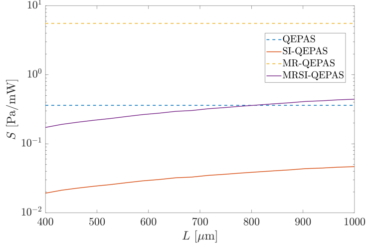
Figure 3.5: Pressure signal per input power ( S ) as a function of the length of the waveguide in the SI-QEPAS and MRSI-QEPAS compared to the pressure signal per input power in QEPAS and MR-QEPAS [62].
