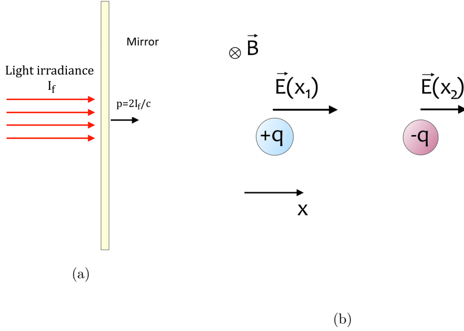
Figure 2.1: Radiation pressure on a moveable mirror (a). Electric field and magnetic field on a dipole, causing optical gradient force (b).
