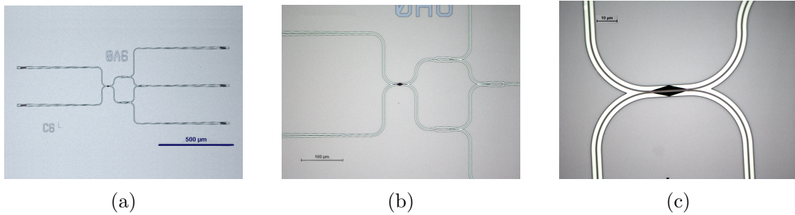
Figure 2.30: Microscope image of the fabricated device with three different zooms on the suspended part.
