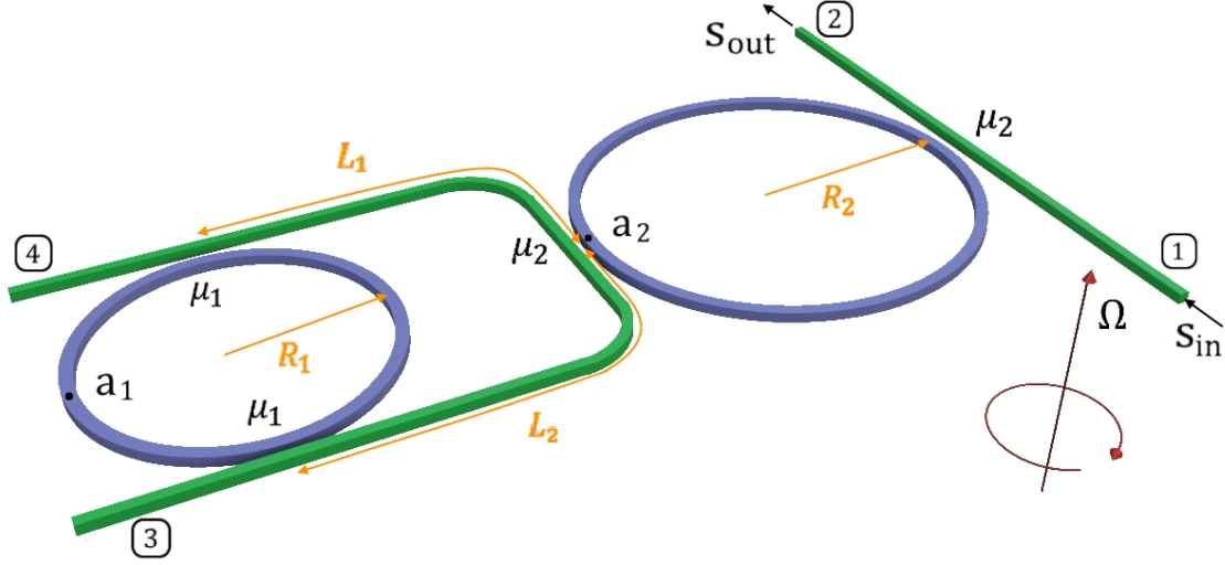
Figure 1.12: Example of the structure of an anti-PT-symmetric gyroscope [13].
