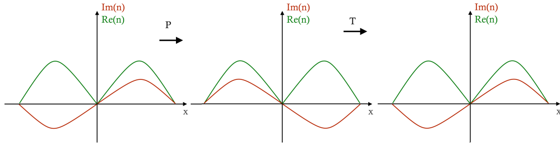
Figure 1.5: Real part and imaginary part of refractive index in parity-time-symmetric systems.
