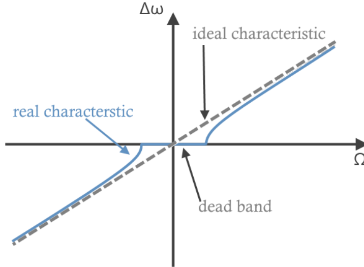
Figure 1.4: Lock-in effect.
