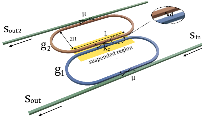
Figure 2.4: General scheme of the racetrack coupled cavities under analysis [46].
