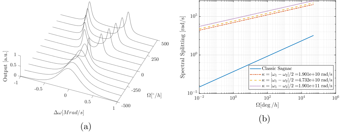
Figure 1.19: (a) Spectrum of the output signal of the gyroscope as a function of the angular velocity and of the frequency detuning from \omega_0 . (b) Splitting as a function of the angular velocity.
