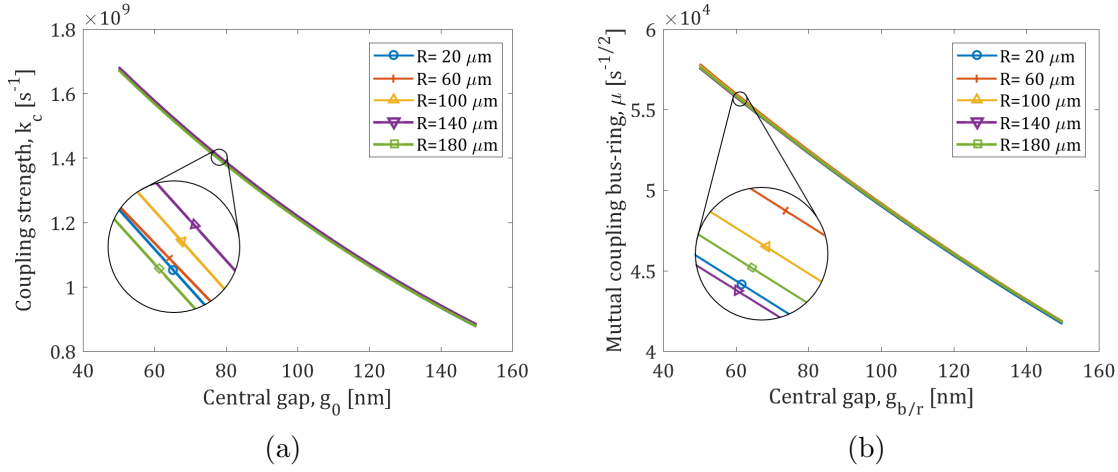
Figure 1.10: Coupling strength as a function of gap g_0 [12] (a). Mutual coupling \mu as a function of gap g_{b/r} [12] (b).
