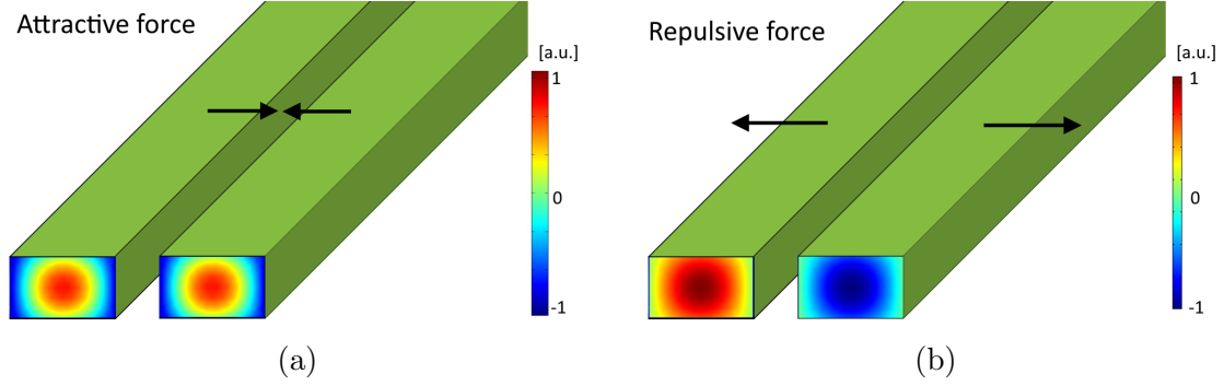
Figure 2.20: Electric field of an even (a) supermode and an odd supermode (b)
