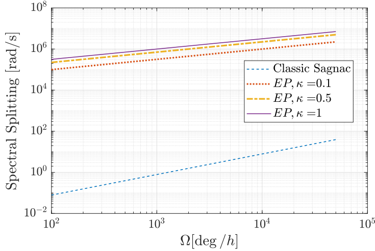
Figure 1.14: Comparison between the spectral splitting at the exceptional point of an anti-PT-symmetric gyroscope (with R_1 = 20 \mu\text{m} and R_2 = 19.95 \mu\text{m} ) and the splitting due to the classical Sagnac effect in a single ring with radius (R_1 + R_2)/2 , around \lambda = 1.55 \mu\text{m} [13].
