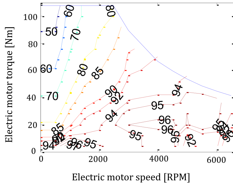
Figure A.4: Efficiency map of an electrical motor [140].
