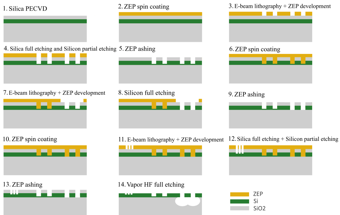
Figure 2.28: Process flow with rib design and hard mask
