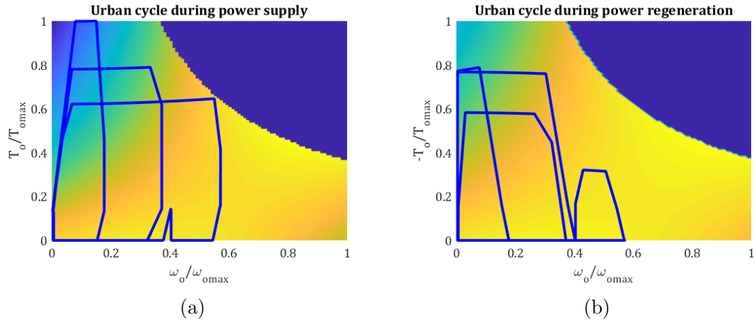
Figure A.6: Working points during an urban cycle over the efficiency map during supplying (a) and regeneration (b) of power [129].
