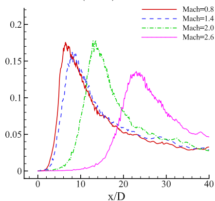
(c) (\overline{w''w''})^{1/2}/u_e
