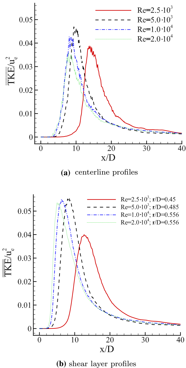
Fig. 16 Normalized \overline{\overline{TKE}} profiles for different Reynolds numbers: a along the centerline; b along the streamwise direction at r/D where the peak value is located (see legend and Fig. 11b)
