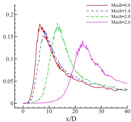
(b) (\overline{v''v''})^{1/2}/u_e
