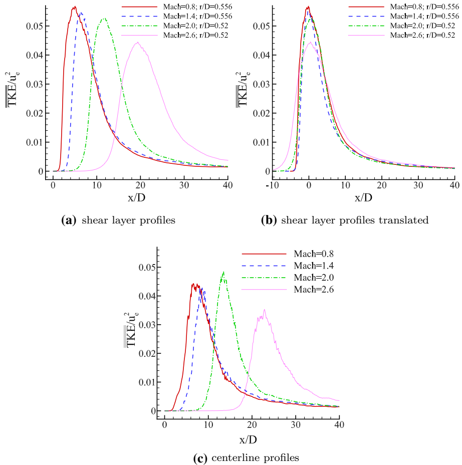
Fig. 12 Normalized \overline{TKE} profiles for different Mach numbers: a along the streamwise direction at r/D where the peak value is reached (see legend and Fig. 11a); b the same profile as (a) but translated by the potential core length; c along the centerline
