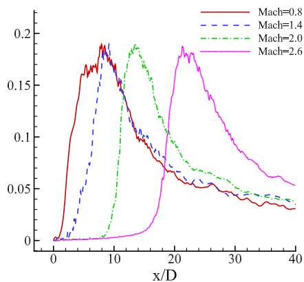
(a) (\overline{u''u''})^{1/2}/u_e
