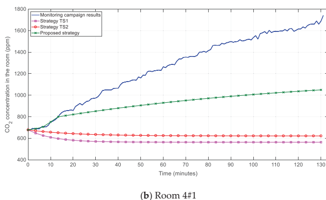
Figure 8. Comparison among monitoring results (without mechanical ventilation) and three strategies involving mechanical ventilation for a two hours experience.
