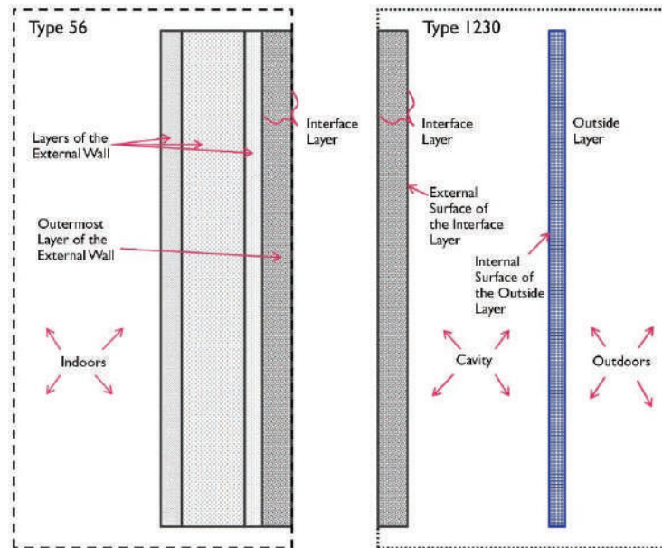
Figure 9. Coupling between Type 56 and Type 1230 [61].
