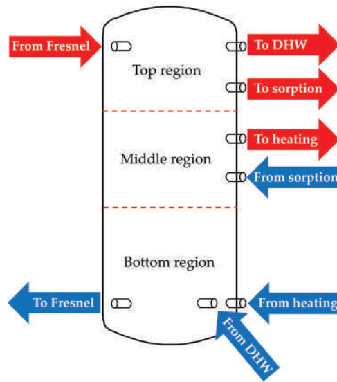
Figure 2. Schematic of the different inlets and outlets of the buffer tank.
