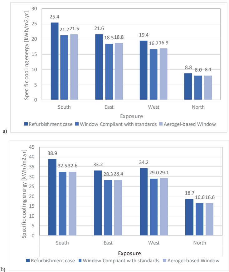
Figure 7. Cooling energy consumptions (kWh/m 2 ·yr) in Toronto (a) and in Bari (b), according to exposures and window type.
