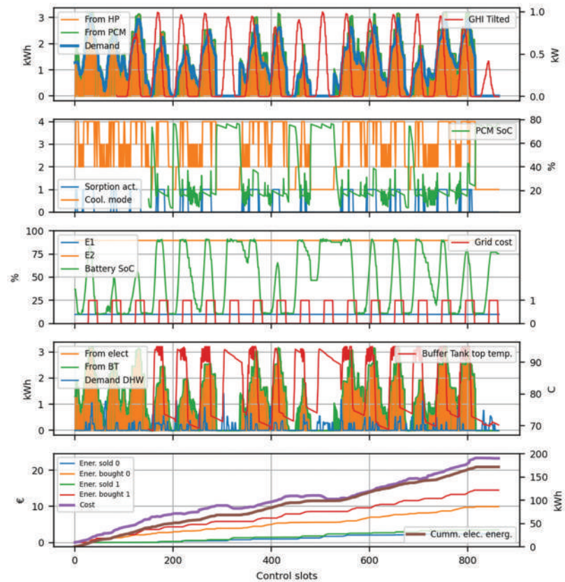
Figure 8. RBC performance results for the test set in cooling mode.
