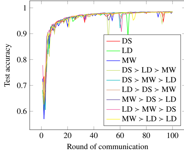
(a) IID distribution
