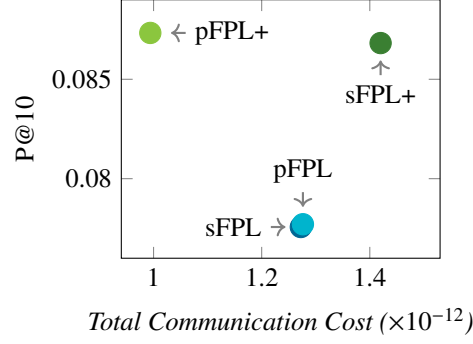
Figure 4.6: Total Communication Cost ( \times 10^{-12} ) compared to precision (P@10) on Brazil dataset. The colors represents the four configurations: dark blue is sFPL, dark green is sFPL+, light blue is pFPL, light green is pFPL+. For each configuration, the best accuracy performance is shown. The top-left corner of the plot is the best trade-off between accuracy and communication costs.
