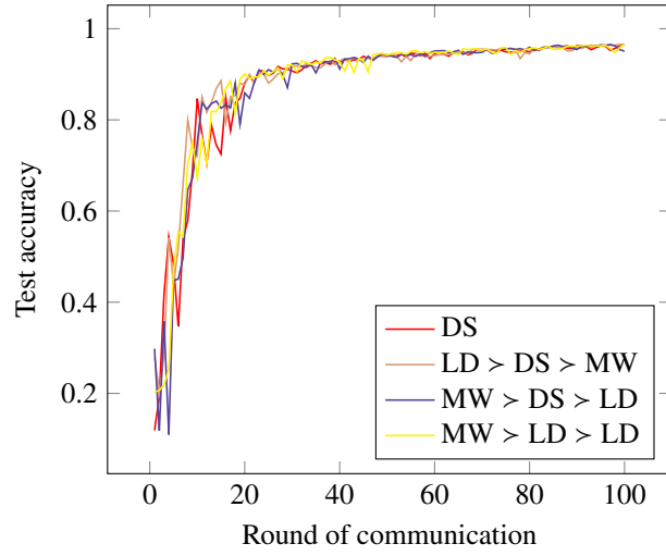
(b) Non-IID distribution
