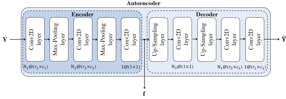
FIGURE 4.2: Architecture of the adopted convolutional autoencoder.
