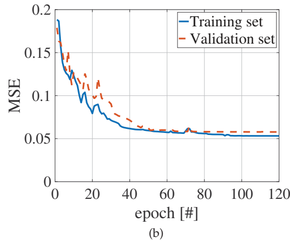
FIGURE 3.6: Prediction loss (i.e., MSE) vs number of epochs for a) ConvLSTM architecture and b) LSTM architecture with attention.
