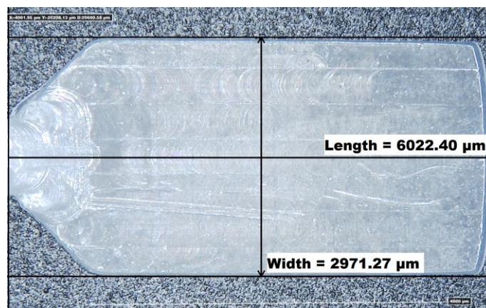
Fig. 9 Component image acquired by microscope
