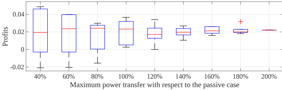
Figure 7.4: Boxplot of the players' net costs with different maximum power transfer.
