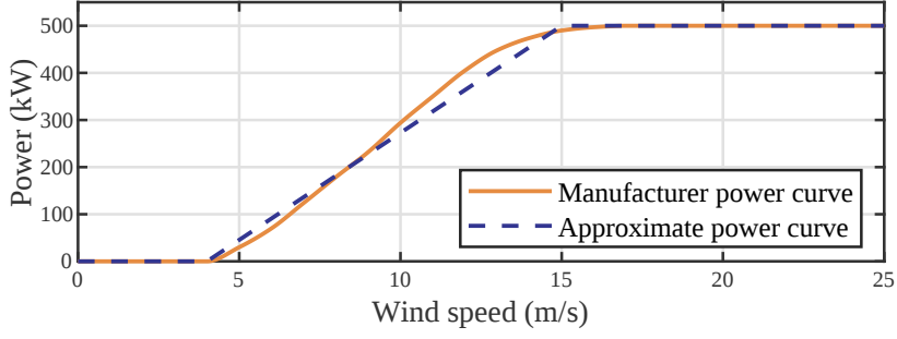
Figure 5.2: Manufacturer and approximate power curve for the NedWind-40 wind turbine [26]. The turbine power curve has characteristic parameters: v_{in} = 4\text{m/s} , v_{rated} = 15\text{m/s} , v_{out} = 25\text{m/s} and \omega_{rated} = 500\text{kW} .
