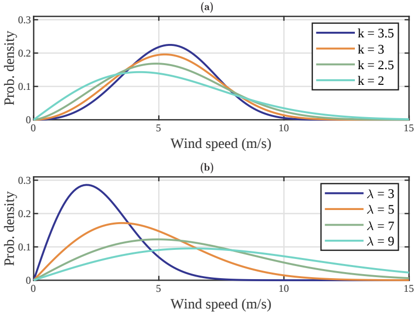
Figure 5.3: Weibull distributions with: (a) \lambda_w = 6 and different k_w values; (b) k_w = 2 and different \lambda_w values.
