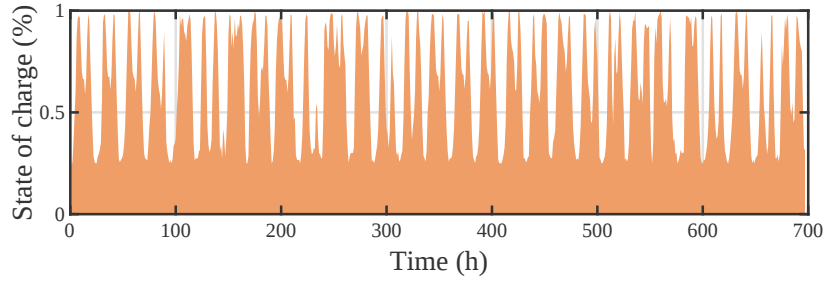
Figure 5.12: Results for station 62121: Mean state of charge of all batteries
