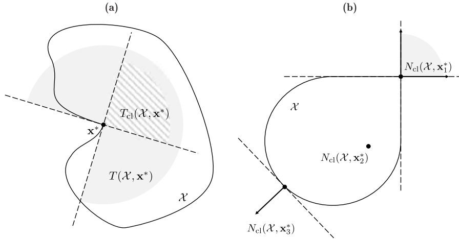
Figure 6.10: Example of a nonconvex set \mathcal{X} with its Bouligand T(\mathcal{X}, \mathbf{x}) and Clarke's tangent cone T_{cl}(\mathcal{X}, \mathbf{x}) in a generic point \mathbf{x} (a). Example of a set \mathcal{X} with three different Clarke's normal cones. (b).
