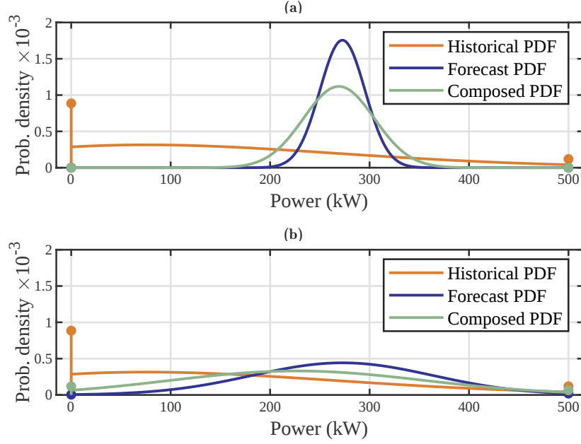
Figure 5.6: Composed wind power PDF (5.25) with different standard deviation values. Calculated for the NedWind-40, with v_{in} = 4\text{m/s} , v_{rated} = 15\text{m/s} , v_{out} = 25\text{m/s} , \omega_{rated} = 500\text{kW} , \mu = 10\text{m/s} , \lambda_w = 8 and k_w = 2 . (a) \sigma = 0.5\text{m/s} . (b) \sigma = 2\text{m/s} .
