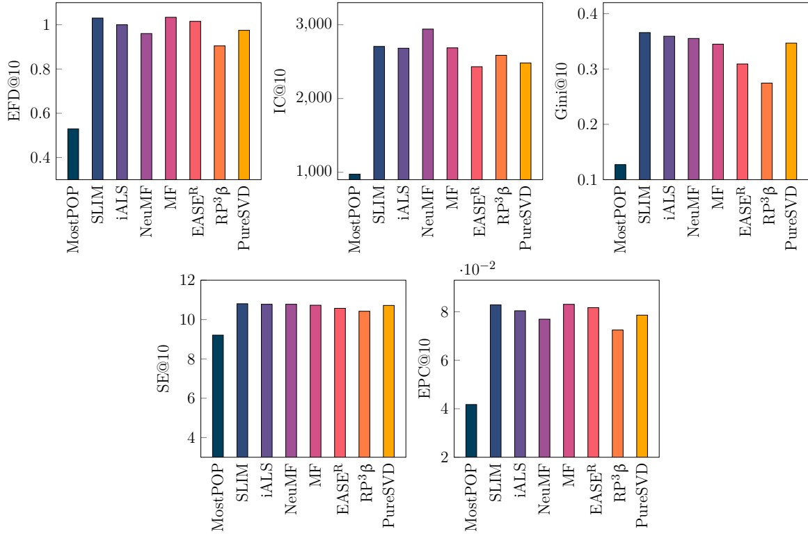
Fig. 4.3 Novelty and Diversity comparison of NeuMF and MF with various baselines (higher is better) for MovieLens dataset.
