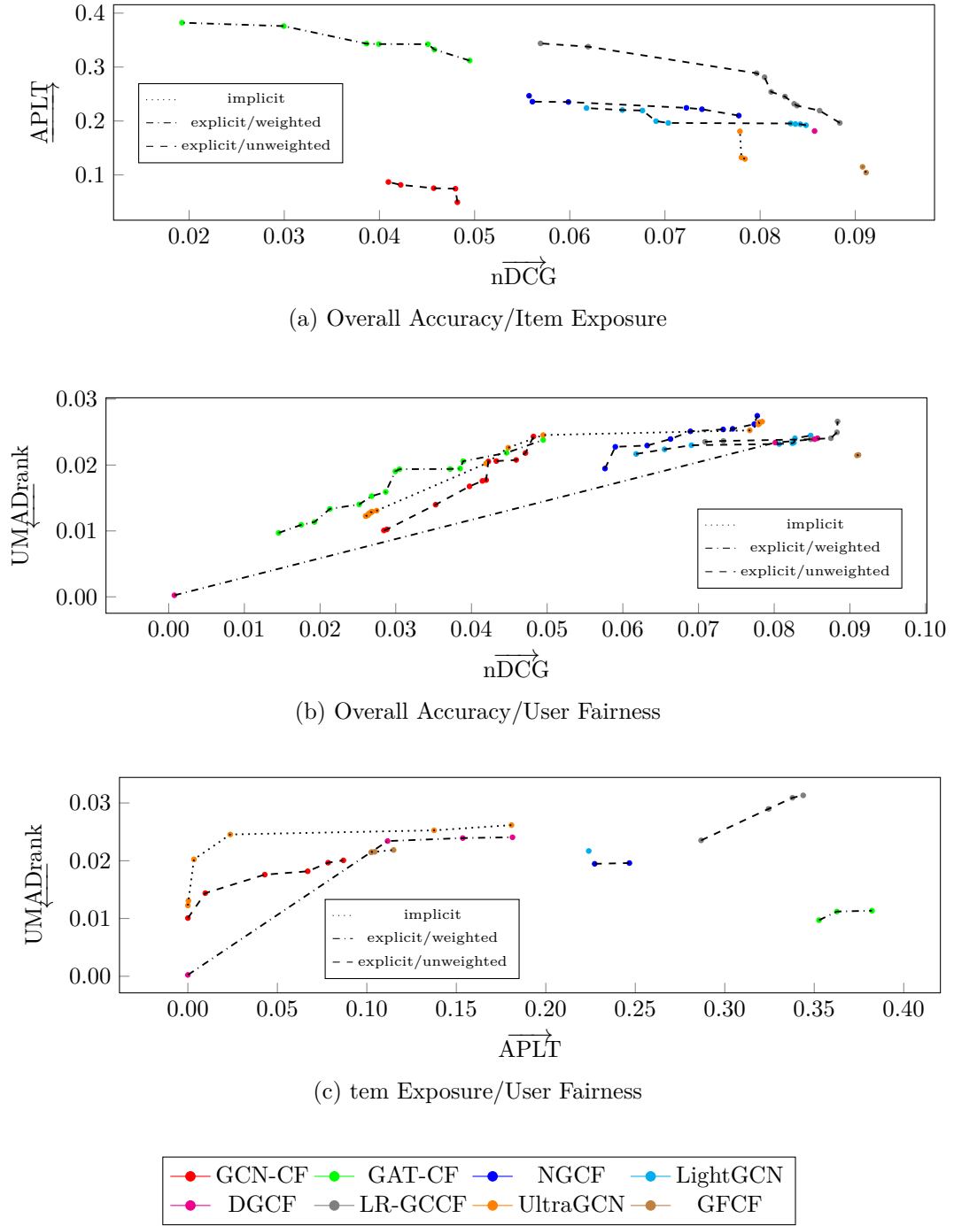
Fig. 5.4 Overall Accuracy/Item Exposure, Overall Accuracy/User Fairness, and Item Exposure/User Fairness trade-offs on Amazon Men, assessed through nDCG/APLT , nDCG/UMADrank , and APLT/UMADrank , respectively. Each point depicts a model hyper-parameter configuration set belonging to the corresponding Pareto frontier. Colors refer to a particular baseline, while lines styles discern their technical characteristics based on the proposed taxonomy. Arrows indicates the optimization direction for each metric on x and y axes.
