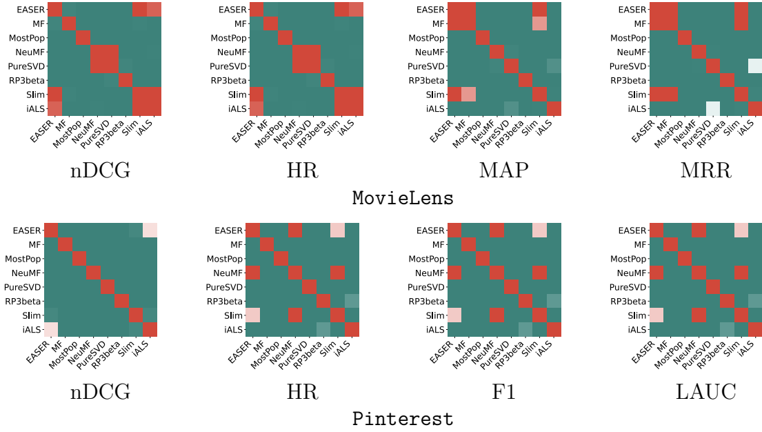
Fig. 4.2 Statistical hypothesis tests using Student's paired t-test with a threshold value (light red) of p=0.05 . Algorithm pairs which results are statistically significant are in green, the results that are not statistically significant are in red.
