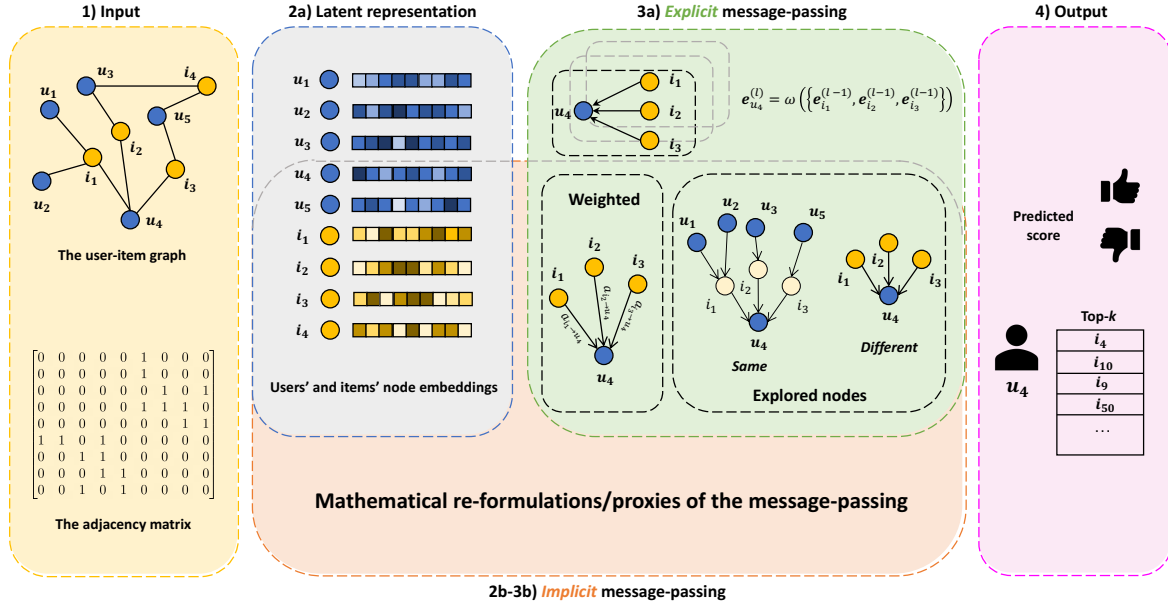
Fig. 5.2 Recommendation stages in graph CF. Starting from the user-item graph and the adjacency matrix (1), a latent representation of the users' and items' nodes is initialized (2a). Afterwards, the node embeddings are iteratively updated by exploring same - or different -type node-node connections through an explicit message-passing schema, which might be optionally weighted (3a). The final outcome is the predicted user-item score, which allows to build a ranked list of items (4). Note that the latent representation and explicit message-passing stages may be substituted (or complemented) through mathematical proxies (i.e., implicit message-passing).
