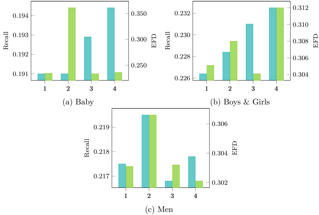
Fig. 5.7 Recommendation performance of EGCF, i.e., Recall@k (histogram bars in teal blue) and EFD@k (histogram bars in lime green), on top-10 recommendation lists, when varying the number of explored hops from 1 to 4.
