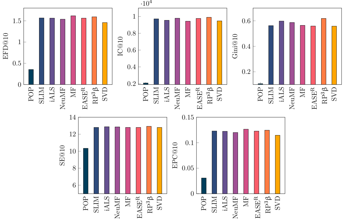
Fig. 4.4 Novelty and Diversity comparison of NeuMF and MF with various baselines (higher is better) for Pinterest dataset.
