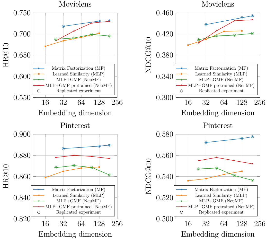
Fig. 4.1 Comparison of learned similarities (MLP, NeuMF) with a dot product: The results for MLP and pretrained NeuMF are from He et al. [113] and Rendle et al. [200]. MF substantially outperforms MF, NeuMF, and pretrained NeuMF. Nonetheless, on MovieLens , when considering large embeddings, pretrained NeuMF is competitive.
