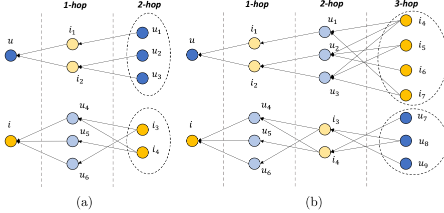
Fig. 5.1 User and item neighborhood exploration after (a) 2 and (b) 3 hops. Contributions to the ego node update are highlighted through dashed ovals. Edge direction indicates the message propagation from neighbor to ego nodes.
