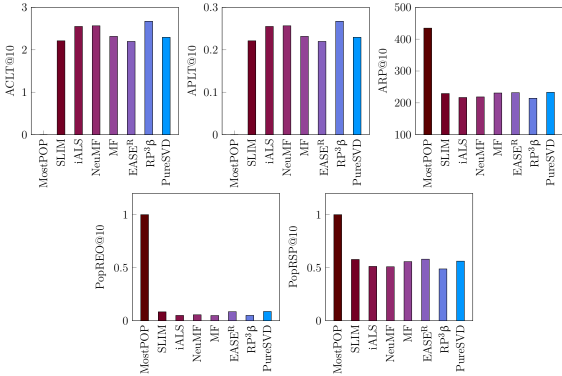
Fig. 4.6 Analysis of Bias for NeuMF, MF and various baselines on the Pinterest dataset. For ACLT, and APLT, higher is better; for ARP, PopREO, and PopRSP, smaller is better.
