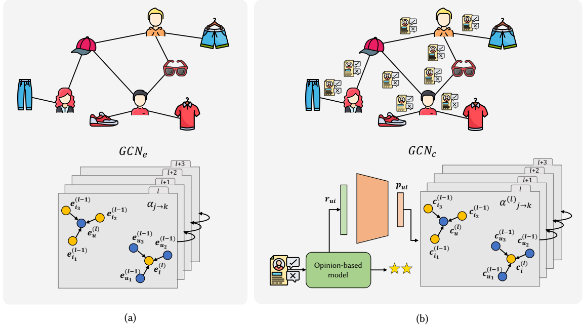
Fig. 5.6 Overview of the node refining algorithm proposed for EGCF. A statically-weighted GCN network affected by node representation error (a) is corrected through another GCN network (b), where an opinion-based embedding is extracted from each review as edge side information to weight the importance of the neighbor nodes on their ego nodes.
