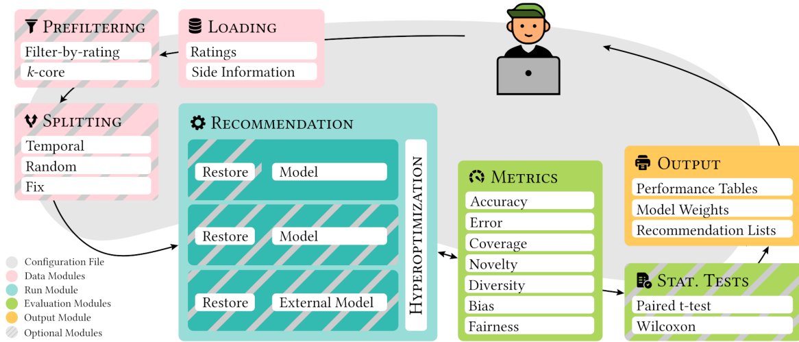
Fig. 3.1 Overview of ELLIOT.
