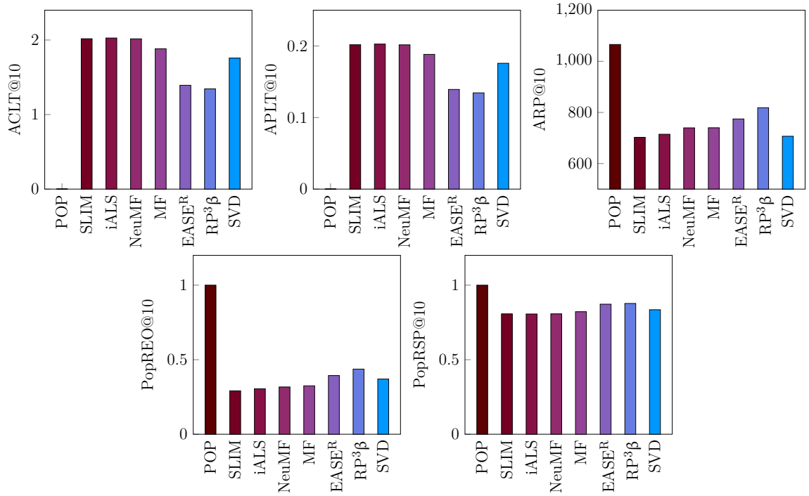
Fig. 4.5 Analysis of Bias for NeuMF, MF and various baselines on the MovieLens dataset. For ACLT, and APLT, higher is better; for ARP, PopREO, and PopRSP, smaller is better.
