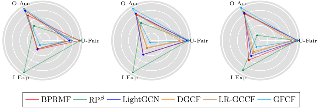
Fig. 5.3 Kiviati diagrams indicating the different performance of selected pure and graph CF recommender models on overall accuracy (i.e., O-Acc, calculated with the nDCG@20 ), item exposure (i.e., I-Exp, calculated with the APLT@20 ), and user fairness (U-Fair, calculated with the UMADrat@20 ). For all dimension the higher values means the better in that dimension.
