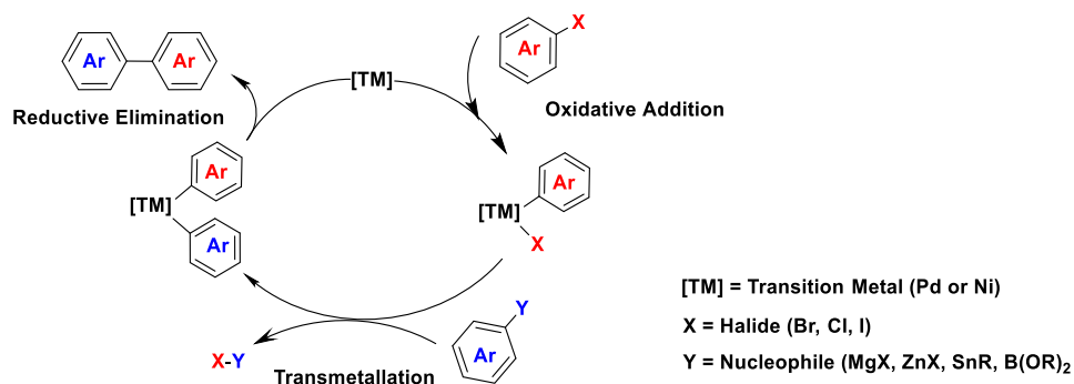
Scheme 1.8. General mechanism for transition metal catalysed cross-coupling reaction.
