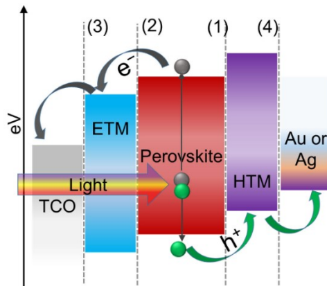
Figure 5.4. Working principles of a conventional n-i-p type perovskite solar cells.
