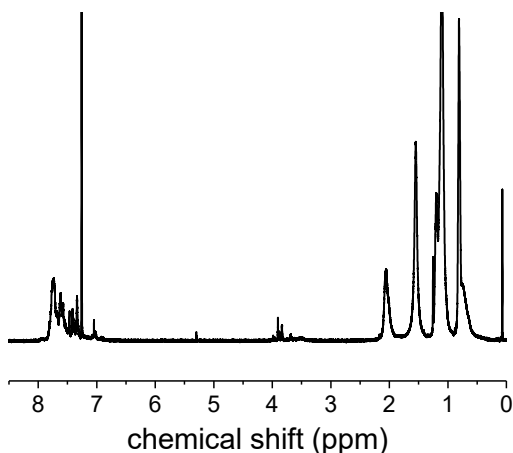
Figure 4.22. ^1\text{H} NMR spectrum of P5 recorded in \text{CDCl}_3 .
