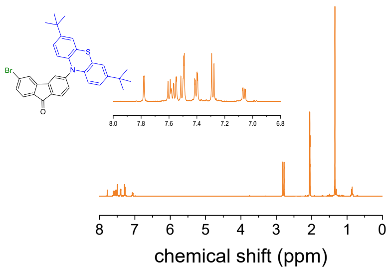
Figure 6.55. ^1\text{H} NMR spectrum of Br-FL-DTP recorded in acetone- d_6 .
