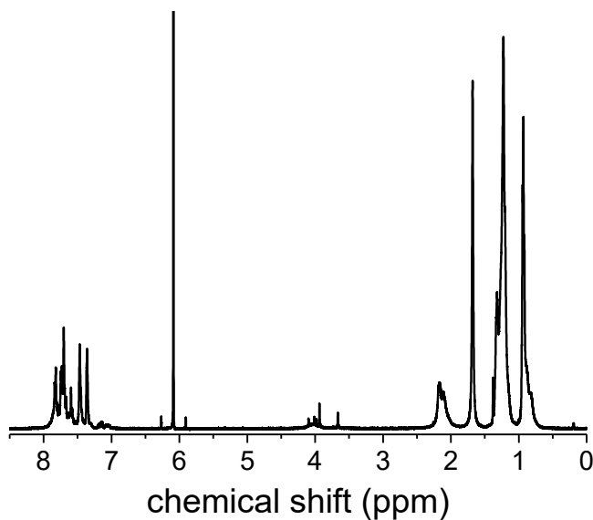
Figure 4.17. ^1\text{H} NMR spectrum of P1 (entry 5) recorded in \text{C}_2\text{D}_2\text{Cl}_4 .
