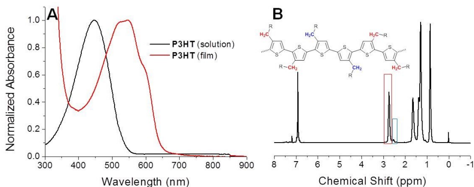
Figure 3.6. (A) Comparison between the absorption spectra of P3HT (entry 5 of Table 2) in solution ( \text{CHCl}_3 ) and in the solid state. (B) ^1\text{H} -NMR spectrum of the same polymer recorded in \text{CDCl}_3 for the determination of their regioregularity by the comparison of the integrals of the marked resonances.
