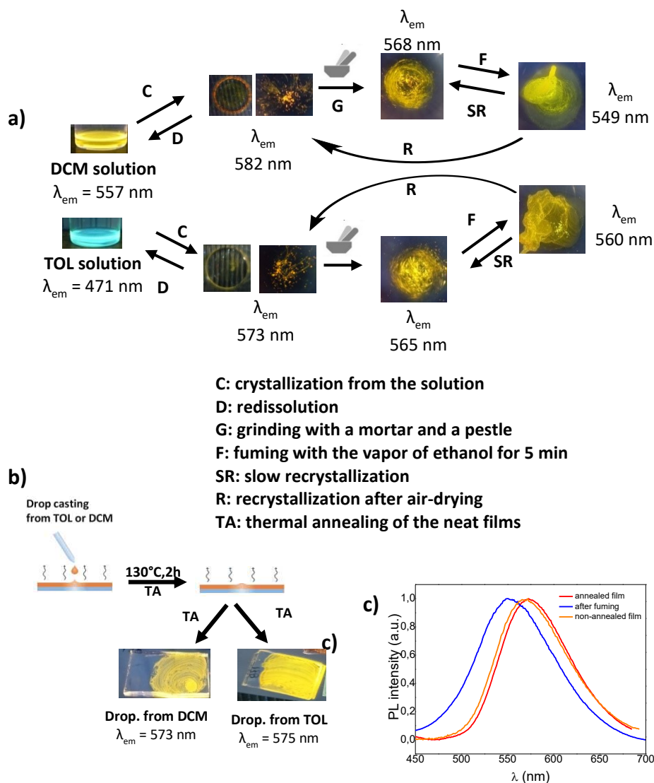
Figure 6.34. a) Schematic diagrams of the multicolor-changing MCL behavior of IN-Ph-DTC (photographs were taken under irradiation with UV light (365 nm)). b) Thermal annealing process of IN-Ph-DTC on quartz slides drop-casted by solutions. c) Overlaid PL emission spectra of the neat film of IN-Ph-DTC, on quartz slide drop-casted by DCM, before annealing (orange), annealed (red) and after fuming with ethanol vapor for 5 min.
