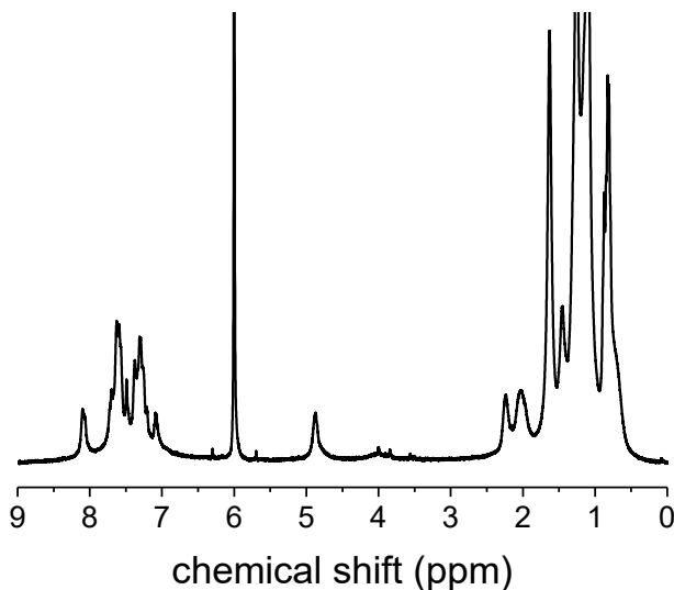
Figure 4.21. ^1\text{H} NMR spectrum of P4 recorded in \text{C}_2\text{D}_2\text{Cl}_4 .
