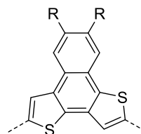
Naphthodithiophene
