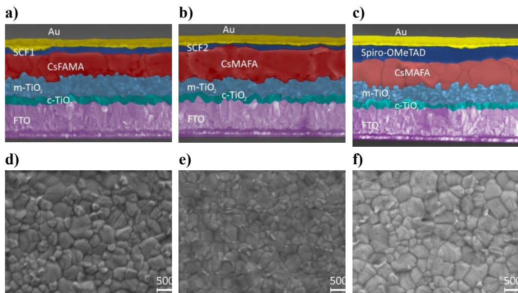
Figure 5.55. Colored cross-section SEM images obtained via scanning electron microscopy of devices utilizing a) SCF1, b) SCF2, and c) Spiro-OMeTAD as the HTM. Top-view SEM-images of 'FTO/c-TiO 2 /m-TiO 2 /Perovskite/HTM' samples, where HTM is d) SCF1, e) SCF2, or f) Spiro-OMeTAD.
