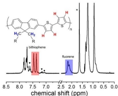
Figure 4.6. ^1\text{H} NMR spectrum of P1 (entry 5) recorded in \text{C}_2\text{D}_2\text{Cl}_4 at 70^\circ\text{C} . (*) Water traces. Signal attributable to the bromo-fluorene (▼) and bithiophene (●) terminating chain.
