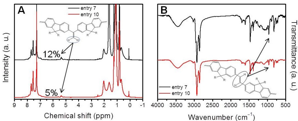
Figure 3.4 (A) ^1\text{H} -NMR spectra ( \text{CDCl}_3 ) of the PFVs synthesized in anisole (entry 7) and in a mixture of anisole and propylene carbonate (4/1 vol/vol, entry 10) indicating the resonances ascribable to the 1,1-diarylene-vinylene defects. (B) IR spectra of the same polymers highlighting the bands ascribable to the out-of-plane C–H bending mode of trans-vinylene moieties.
