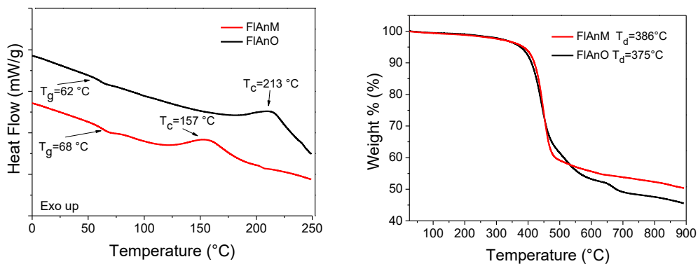
Figure 5.15. a) DSC traces of FIA n O (black) and FIA n M (red) (second heating scans) identifying the glass transitions ( T_g ) and cold crystallization ( T_c ) events. b) TGA curves of a) FIA n O (black) and FIA n M (red).
