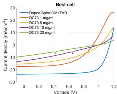
Figure 5.18. J-V curves of PSCs using polymers FIAnO (DC73 in the legend) and doped Spiro-OMeTAD as HTMs.
