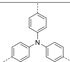
Triphenylamine
