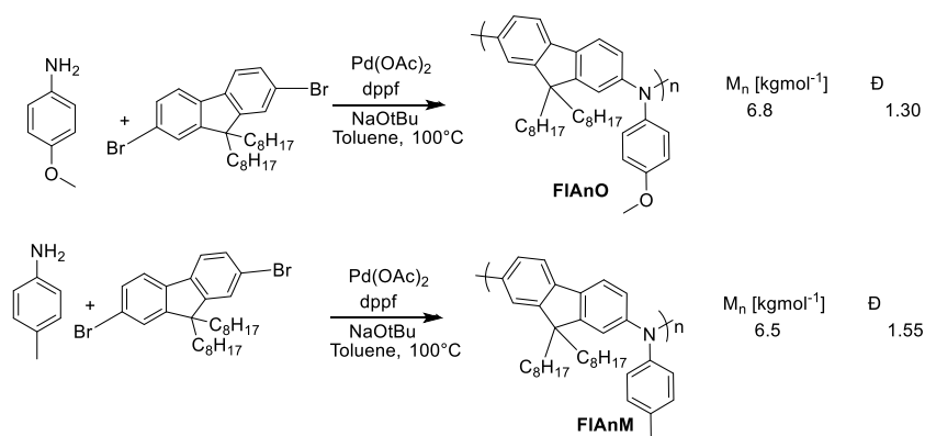
Figure 5.13. Synthetic sequence for the obtainment of P1 and P2 with the related number average molecular weight ( M_n ) and dispersity ( \bar{D} ).
