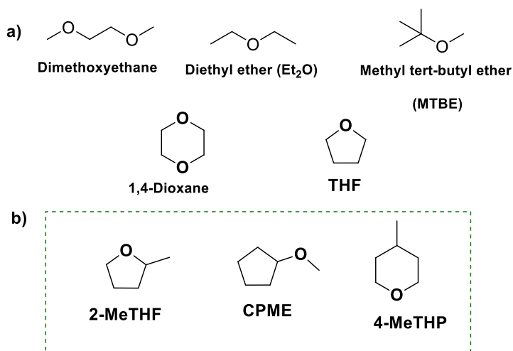
Figure 2.1 a) Traditional etheral solvents used in laboratories and b) low environmental impact alternatives.
