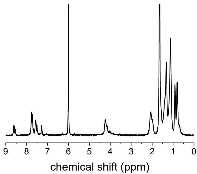
Figure 4.24. ^1\text{H} NMR spectrum of P8 recorded in \text{C}_2\text{D}_2\text{Cl}_4 .
