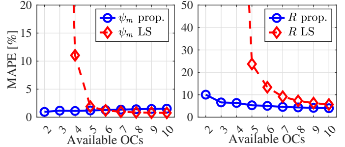
Fig. 11: Estimations of \psi_m and R in different scenarios with the proposed and the LS method.
