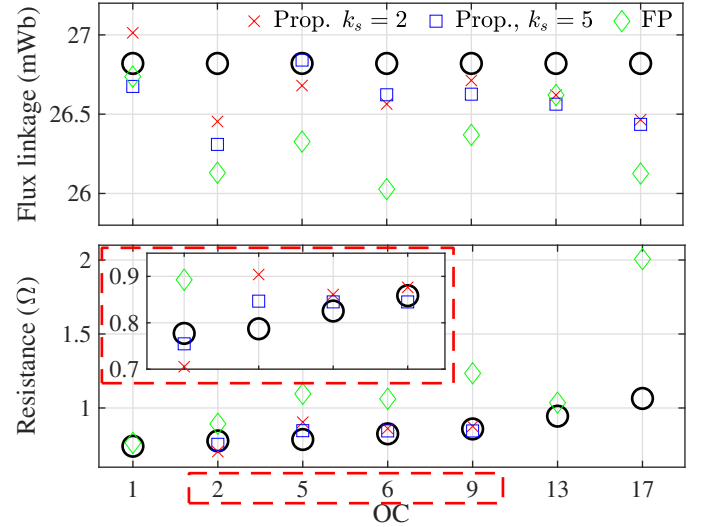
Fig. 10: Estimations of \psi_m and R with 2 and 5 OCs compared with the FP method. The black circles denote measured values.
