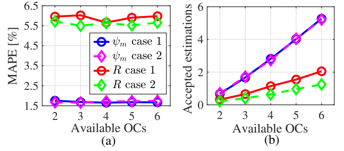
Fig. 5: Estimation of \psi_m and R in different scenarios: (a) MAPE of the estimation results, (b) average number of accepted estimations compared with the number of available OCs.
