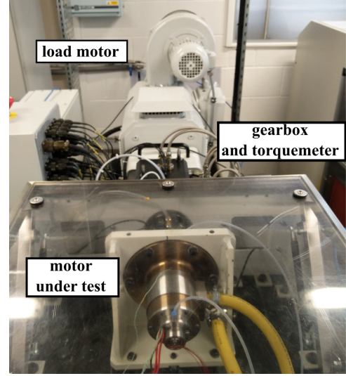
Fig. 6: Experimental setup layout.
