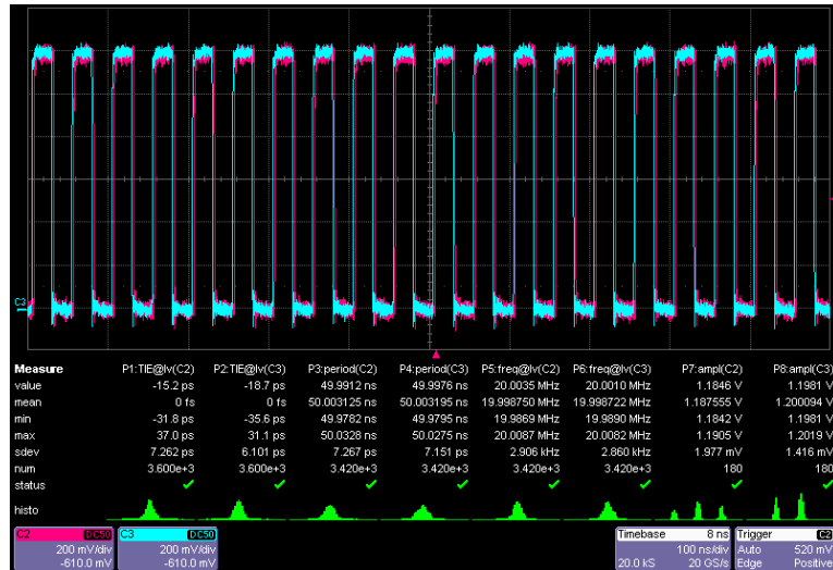
Figure A.17: Statistics on the output of the squaring board for the jitter analysis in the time domain.
