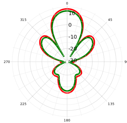
Figure A.7: Simulated gain (in green) and directivity (in red) of the designed patch antenna.
