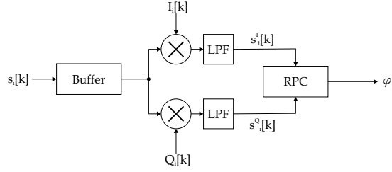
Figure 3.2: Block diagram sketching the operations performed by IQ LPM for channel i .
