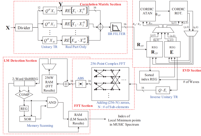
Figure 2.8: Block diagram of the MUSIC algorithm implementation proposed by Kim et al. in [14] © 2003, IEEE.
