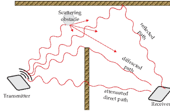
Figure 1.7: A sketch of the basic propagation mechanisms which may generate artifacts on the positioning systems.
