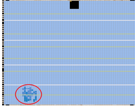
Figure 5.16: Layout of the proposed architecture mapped on the Intel Cyclone IV E EP4CE115F29C7 FPGA (4 channels, L = C = 8 bits, A = 7 bits).
