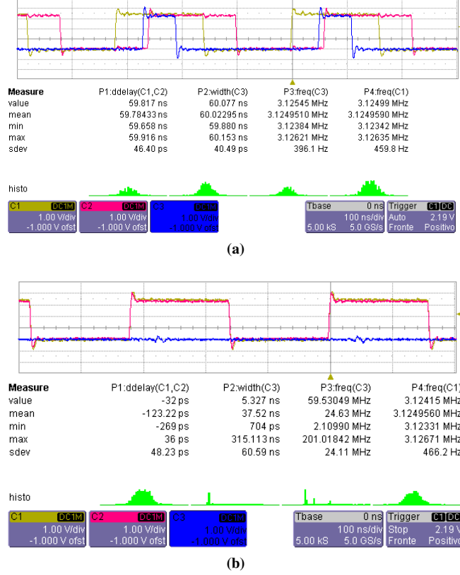
Figure 5.6: Oscilloscope screenshot with traces and statistics showing the case of (a) two phase shifted channels (on CH1 and CH2 respectively) and the PCS signal (on CH3). In (b) the same setup is showing the behavior for two nominally synchronous signals.
