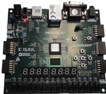
Figure 6.9: Digilent Nexys A7 Evaluation and Development board for the Xilinx Artix-7 100T.
