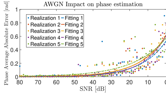
Figure 3.3: Simulation realizations and exponential fitting of the AWGN impact analysis on phase estimation accuracy.
