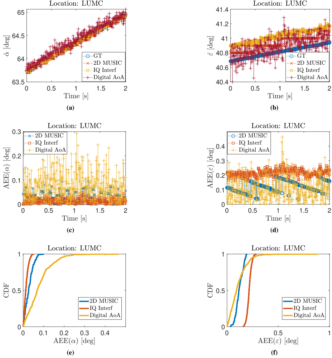
Figure 6.17: Results of the AoA estimation and Location "LUMC" using the three approaches under comparison: (a) Azimuth angle tracking over time, (b) Elevation angle tracking over time, (c) AEE for the azimuth angle over time, (d) AEE for the elevation angle over time, (e) CDF of the AEE for the azimuth angle, and (f) CDF of the AEE for the elevation angle.
