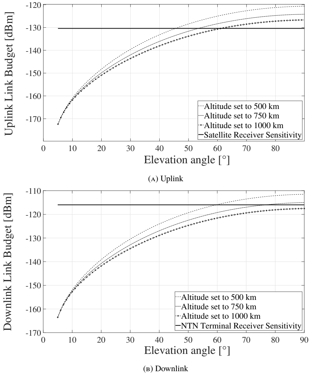
FIGURE 1.6: Link Budget in the function of Elevation Angle for different orbital altitudes.
