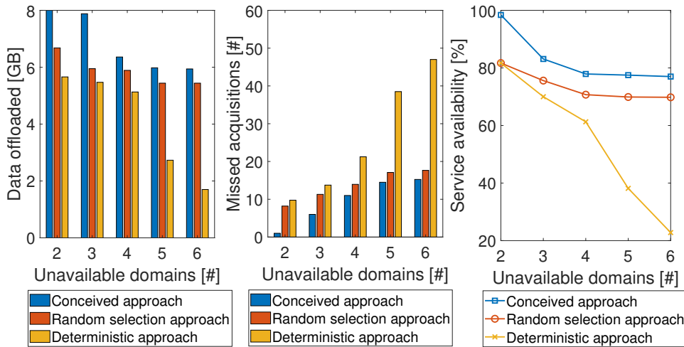
FIGURE 3.4: Offloaded data, missed acquisitions and overall service availability for CPU SLA focus.
