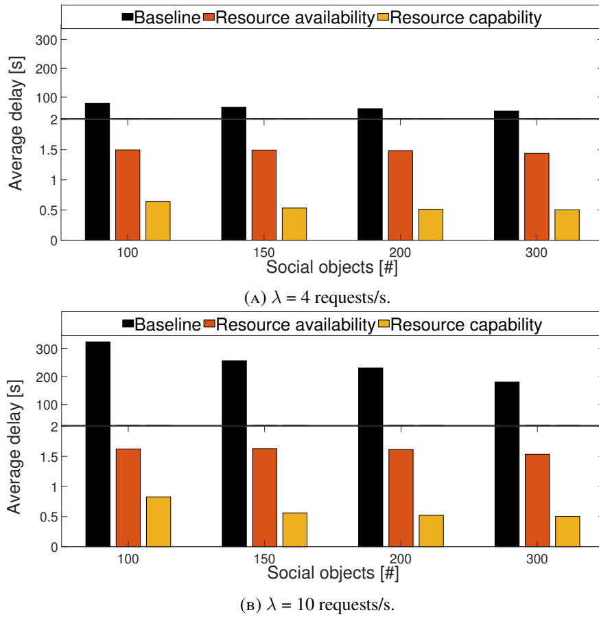
FIGURE 2.8: Average delay.
