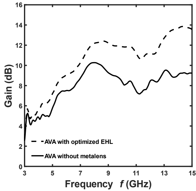
Figure 4.8 Full-wave simulation of the gain G as a function of frequency for AVA (solid curve) and AVA with EHL having a thickness of d_{EHL} = 0.832 \text{ mm} for the optimized effective permittivity \epsilon_{eff \text{ MG}} and effective permeability \mu_{eff \text{ MG}} (dashed curve) [6].
