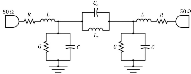
Figure 5.6 Equivalent circuit of the single-slot SIW applicator [10].
