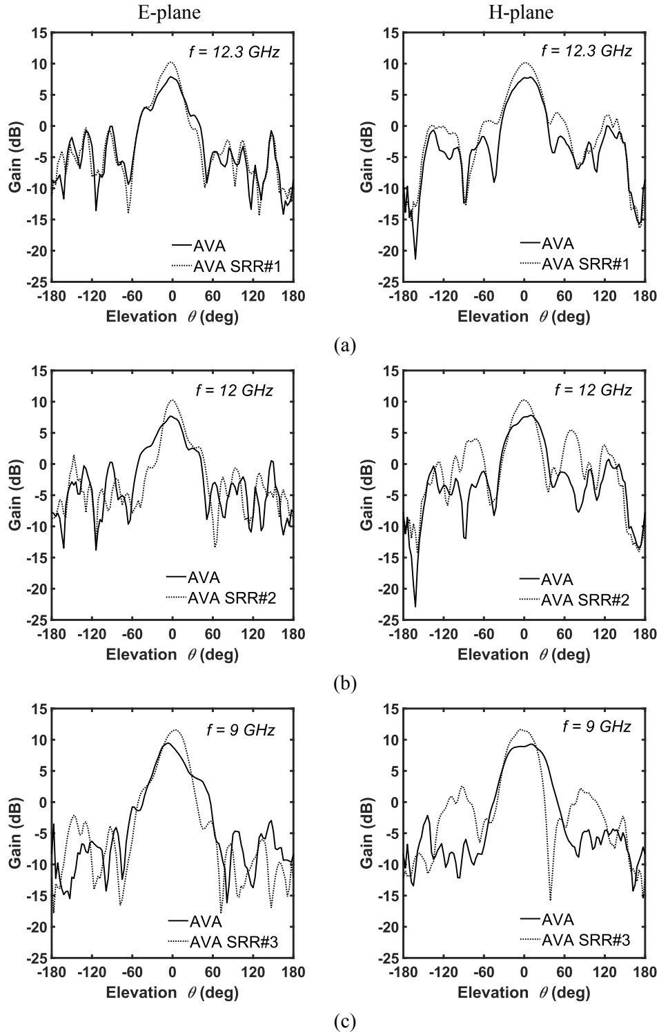
Figure 4.29 Measured E-plane (left column) and H-plane (right column) radiation patterns of the AVA (solid curve) and (a) AVA SRR#1 (dotted curve) at frequency f = 12.3 GHz, (b) AVA SRR#2 (dotted curve) at frequency f = 12 GHz, and (c) AVA SRR#3 (dotted curve) at frequency f = 9 GHz [7].
