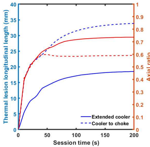
Figure 3.19 Simulated longitudinal length and axial ratio of the thermal lesion as a function of ablation time duration t of the 14G MW applicator, Figure 3.2b, with cooler stopped at choke (dashed curve) and extended at slot (solid curve), average power P_{avg} = 20\text{ W} [2].
