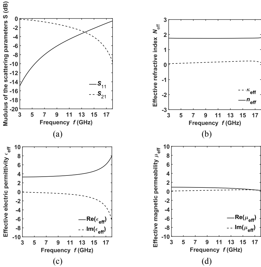
Figure 4.6 (a) The simulated S-parameters and the retrieved effective parameters as a function of the frequency f : (b) complex refractive index N_{eff} , (c) effective electric permittivity \epsilon_{eff} , and (d) effective magnetic permeability \mu_{eff} of SRR unit cell [7].
