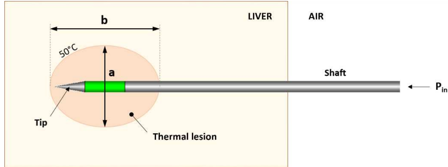
Figure 3.4 Scheme of the ablation zone. The T = 50^\circ\text{C} isothermal line determinate the boundary of the thermal lesion.
