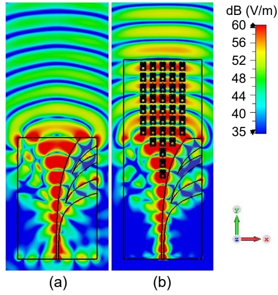
Figure 4.22 Full-wave simulation of the E-field distribution in xy -plane at f = 14 GHz of (a) AVA without metalens and (b) AVA-L-shaped#1 [6].
