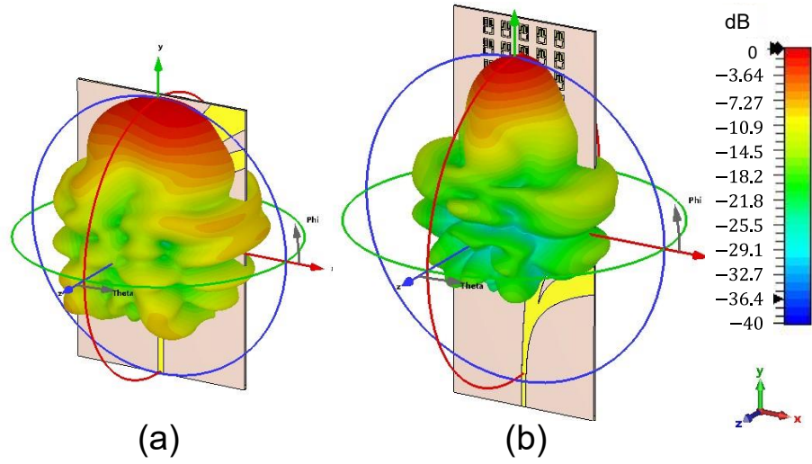
Figure 4.23 Full-wave simulation of the normalized radiation patterns 3D view at frequency f = 14 GHz of (a) AVA without metalens and (b) AVA L-shaped#1 [6].
