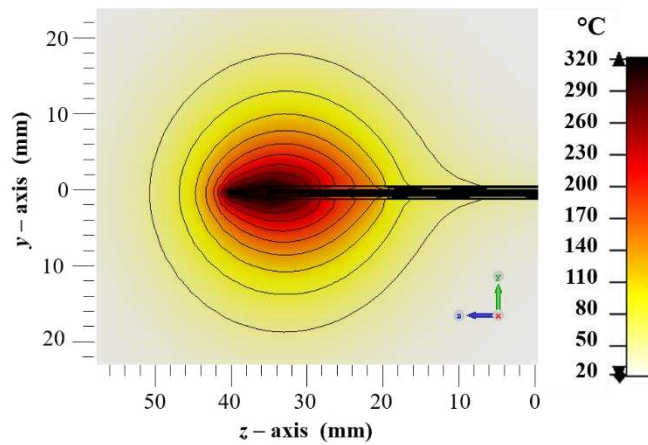
Figure 3.21 Longitudinal section of the temperature distribution into the hepatic tissue simulated with a power supply of P = 20\text{ W} , after an ablation duration time of t = 600\text{ s} . Ex-vivo thermal simulation of the 16G needle MW applicator optimized for the prototyping [3].
