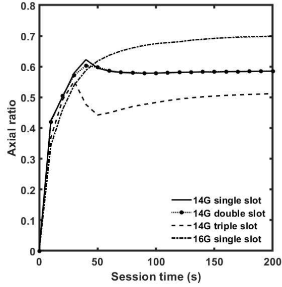
Figure 3.10 Simulated axial ratio of the thermal lesion as a function of the ablation time duration t , average input power P_{avg} = 20 \text{ W} . 16G MW applicator, Figure 3.2b vs. 14G MW applicator, Figure 3.2b, 14G MW applicator, Figure 3.2c, and 14G MW applicator, Figure 3.2d [2].
