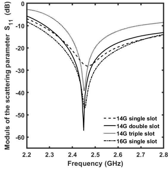
Figure 3.9 Modulus of the simulated scattering parameter S_{11} as a function of the frequency f , average input power P_{avg} = 20 \text{ W} . 16G MW applicator, Figure 3.2b vs. 14G MW applicator, Figure 3.2b, 14G MW applicator, Figure 3.2c, and 14G MW applicator, Figure 3.2d [2].
