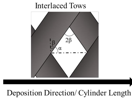
Fig. 3: Scheme of the angles in a helical winding pattern
