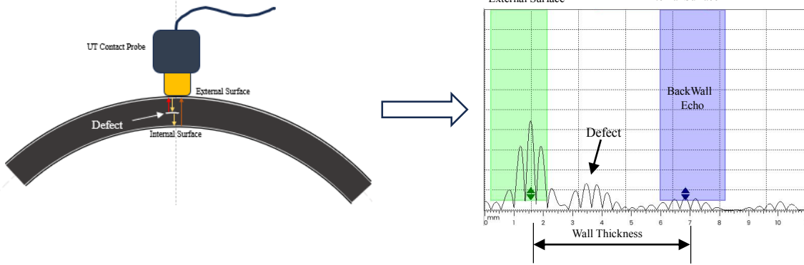
(b) Pulse-Echo with the presence of defect
