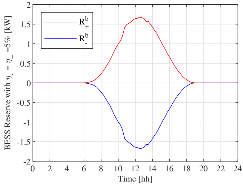
Figure 3.13: Positive and negative reserve in microgrid 1 provided by the BESS unit.
