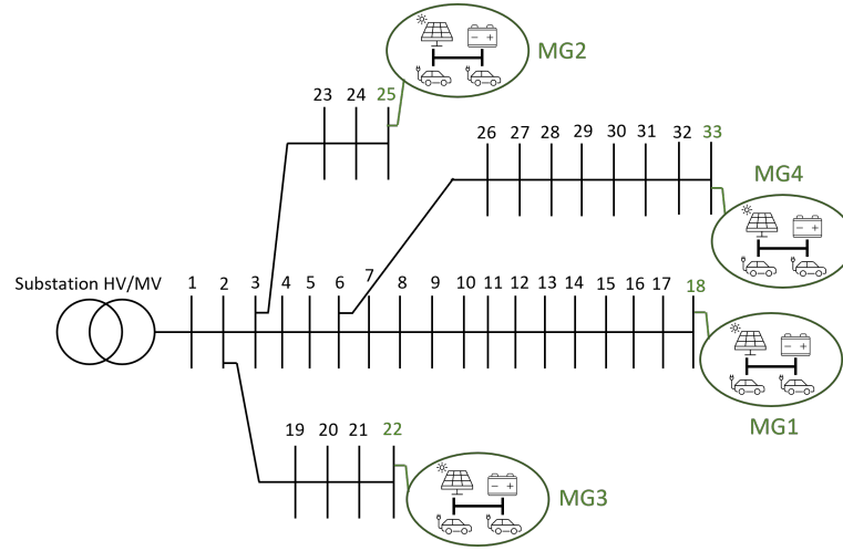
Figure 4.47: IEEE-33 grid topology with the integration of 4 DC microgrids.
