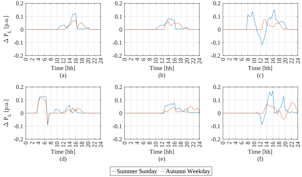
Figure 4.30: Delta energy losses considering 36 integrated EVs in scenarios S1 and A1 (a), S2 and A2 (b), S3 and A3 (c), S4 and A4 (d), S5 and A5 (e) and S6 and A6 (f).
