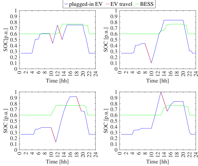
Figure 4.53: EV and BESS SOC levels in microgrid 1 (a), 2 (b), 3 (c), and 4 (d).
