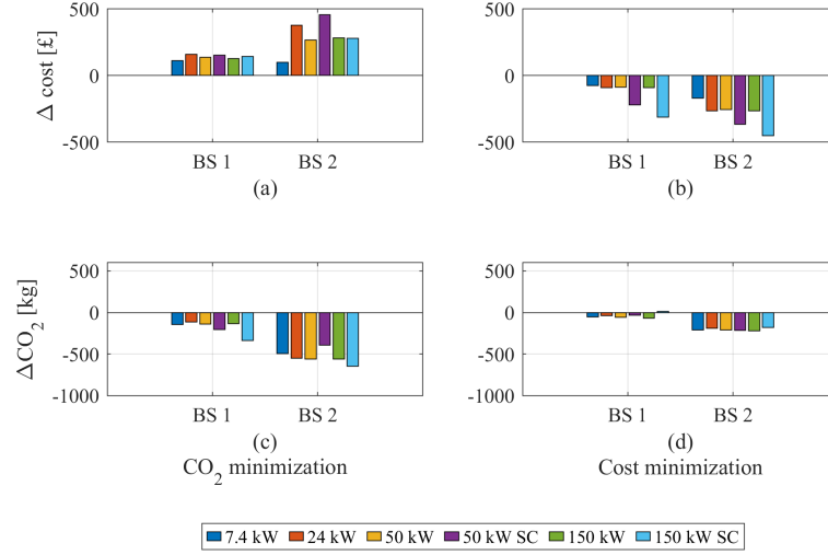
Figure 4.8: Winter week. Total daily cost variation (a)-(b) and CO 2 variations (c)-(d) for both BS configurations and optimal strategies.
