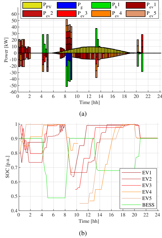
Figure 2.11: Application of OF3 to Configuration 1 in a summer day, considering EV Scenario 2. Power exchanges (a) and trends of EVs and BESS state of charge (b).
