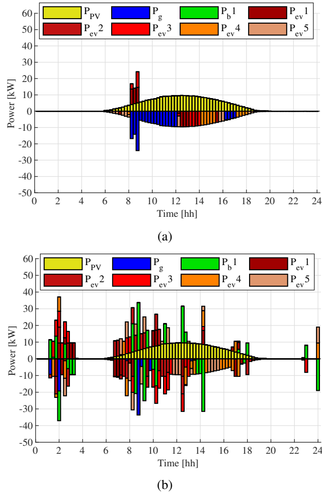
Figure 2.10: Application of OF1 (a) and OF2 (b) to Configuration 1 in a summer day, considering EV Scenario 2. Power exchanges.
