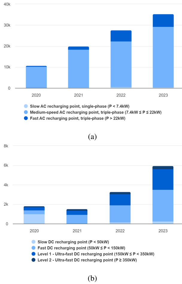
Figure 1.5: Total number of publicly accessible AC (a) and DC (b) EV charging points, according to AFIR categorization [8].
