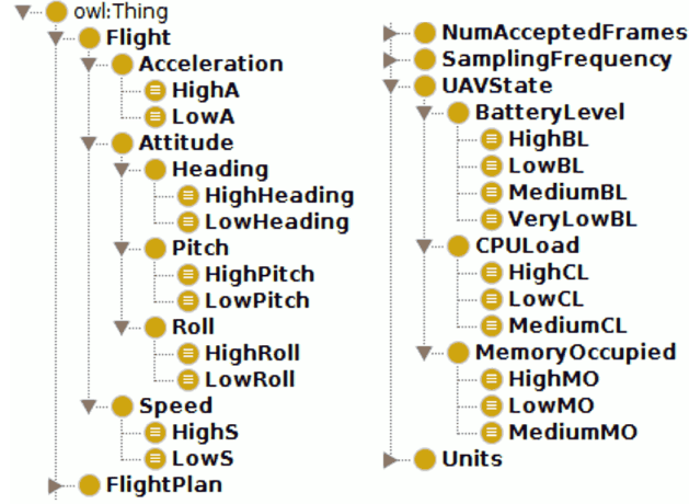
Figure 5.7: Excerpt of the context awareness knowledge base.
