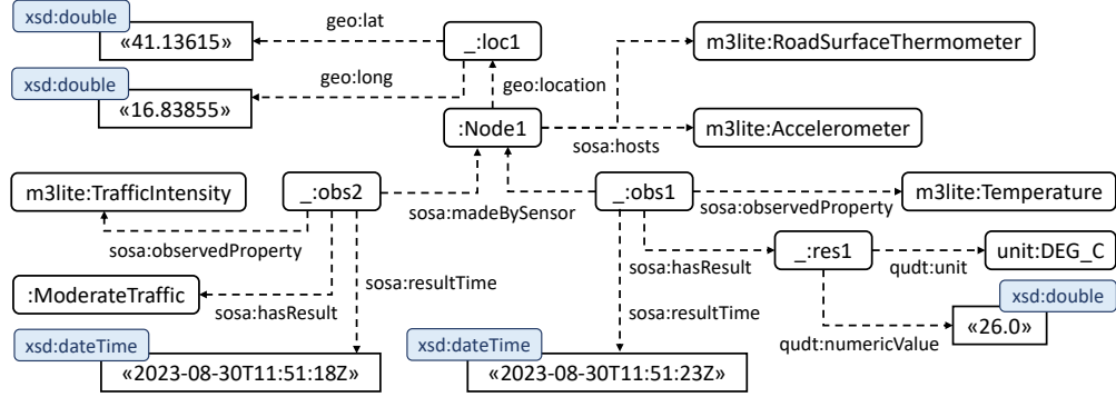
Figure 5.2: Example of road context annotation.
