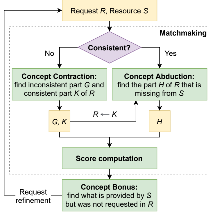
Figure 1.2: Semantic matchmaking framework.
