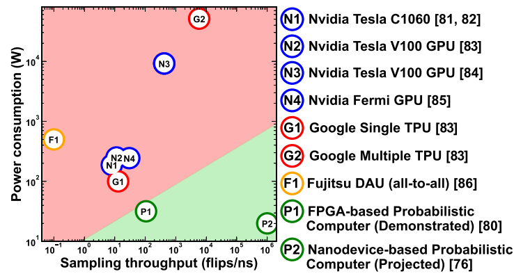
Figure 12. Published data on power consumption (W) vs. sampling throughput (flips/ns) on state-of-the-art probabilistic samplers. © [2023] IEEE. Reprinted, with permission, from [87].
