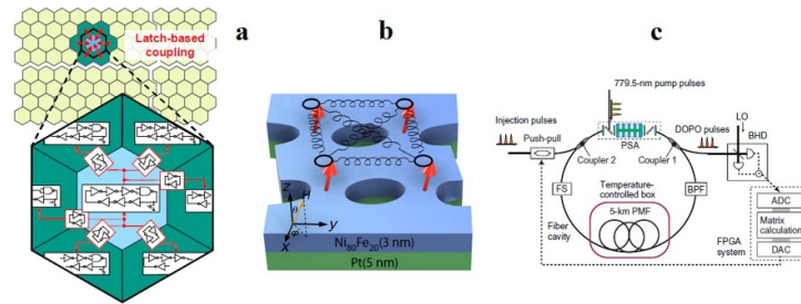
Figure 19. Sketches of different implementations for Ising Machines realized through coupled oscillators of different types: (a) hexagonal ring-oscillators [125], © [2020] IEEE. Reprinted, with permission, from [125]. (b) Nanoconstriction-based spin-Hall nano-oscillators [128], Reproduced from [128]. CC BY 4.0. (c) Optical parametric oscillators [131]. From [131]. Reprinted with permission from AAAS.
