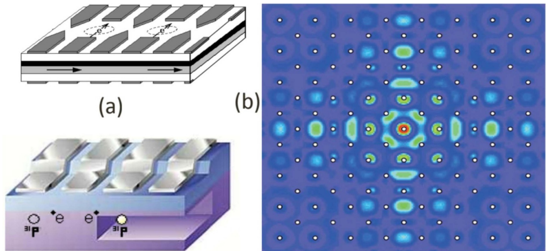
Figure 13. (a) Schematic representation of early (1998) QC architectures with spin qubits in semiconductors. Upper scheme represents Loss-DiVincenzo's proposal on GaAs (qubits bound to quantum wells [88]); bottom scheme represents Kane's proposal involving P substitutional donors in Si [89]. (b) Electron probability density around a P substitutional donor on the (001) plane of bulk Si for the donor ground state. The white dots give the in-plane atomic sites. Reproduced from [92]. CC BY 4.0.
