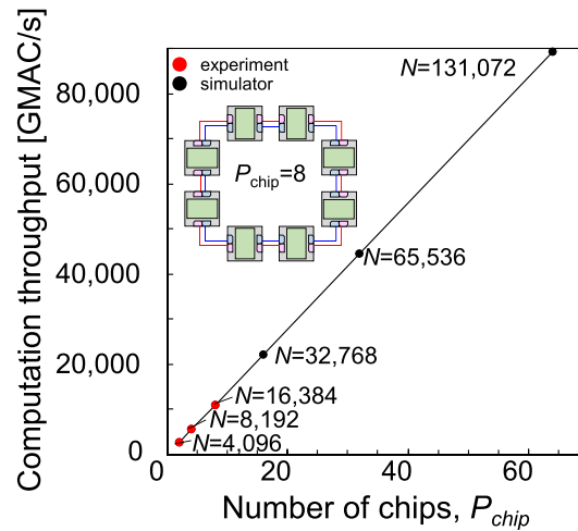
Figure 18. Scale-out architecture for SB [117]. Constant-efficiency scaling characteristic. (Inset) Connection of multiple chips in a bidirectional ring topology.
