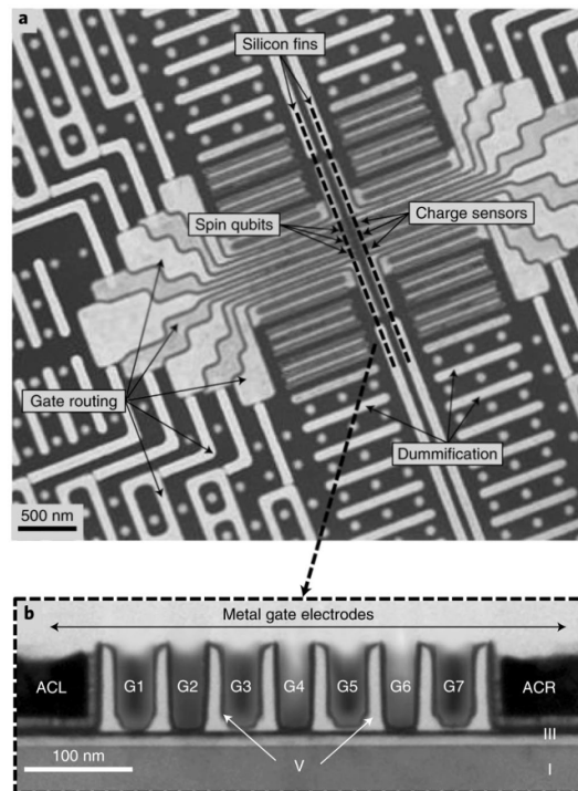
Figure 14. (a) Electron microscopy image of an industrially fabricated QD device by Intel and QuTech, showing two parallel silicon fins, one hosting the qubits (left) and the other hosting the sensing QDs (right). Gate routing and dummification (required for maintaining a constant metal density on the surface) are also clearly shown. (b) Image along a Si fin of a QD array showing seven metallic silver gates (G1-G7) between two accumulation gates (ACL and ACR). Reproduced from [93]. CC BY 4.0.
