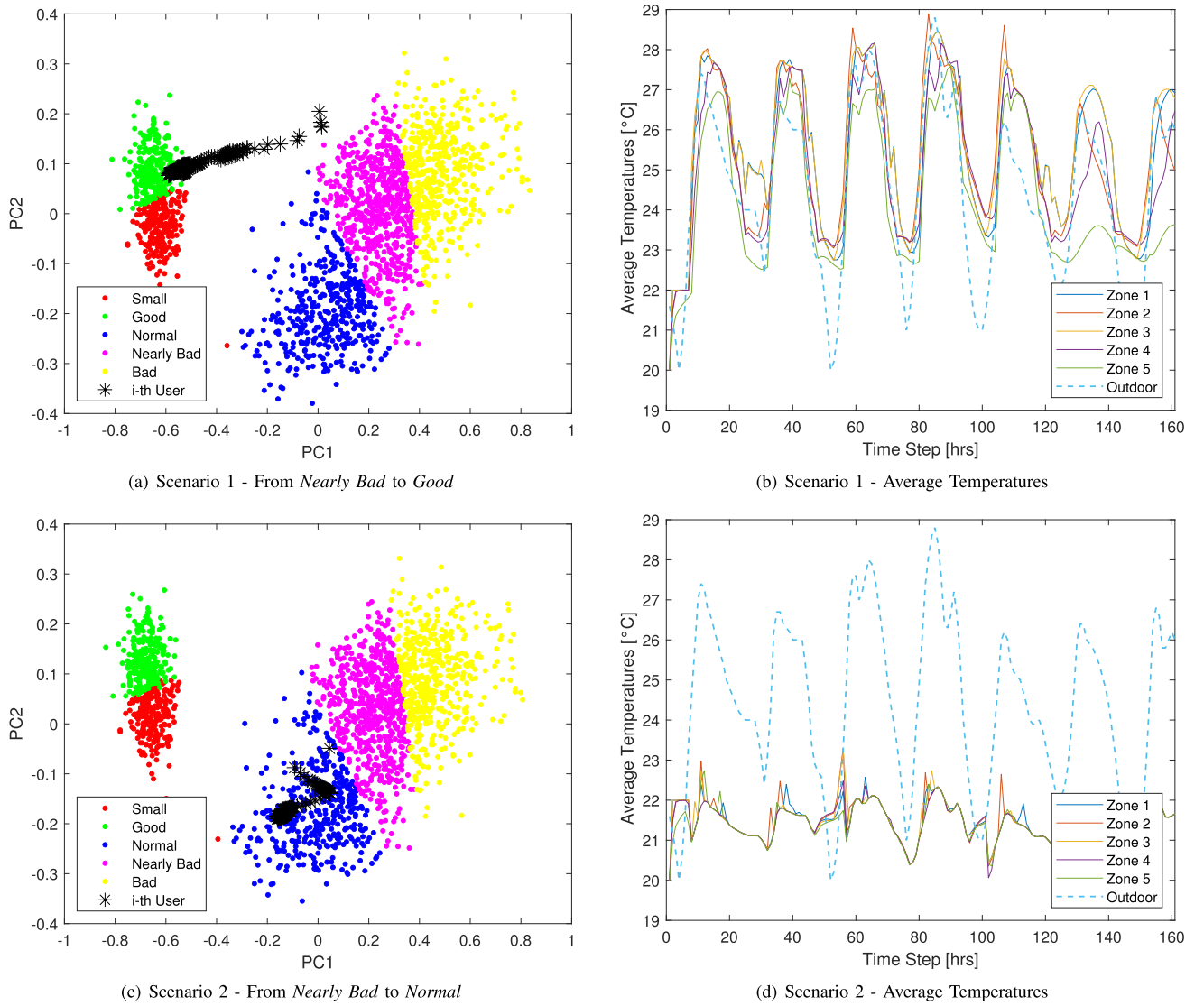
Fig. 9. Optimized Class Follower MPC scheme progress over the billing period.
