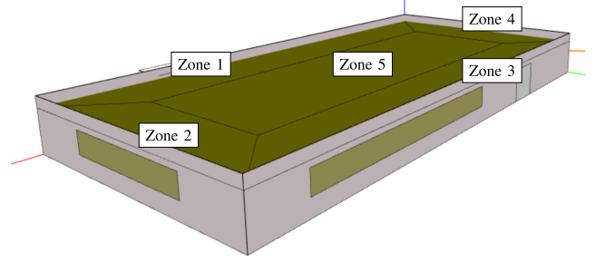
Fig. 7. 5-zones air-conditioned building.
