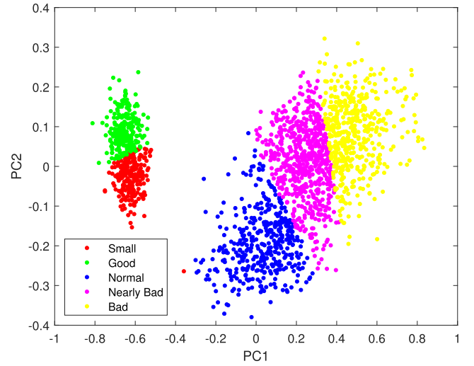
Fig. 3. K-means clustering.
