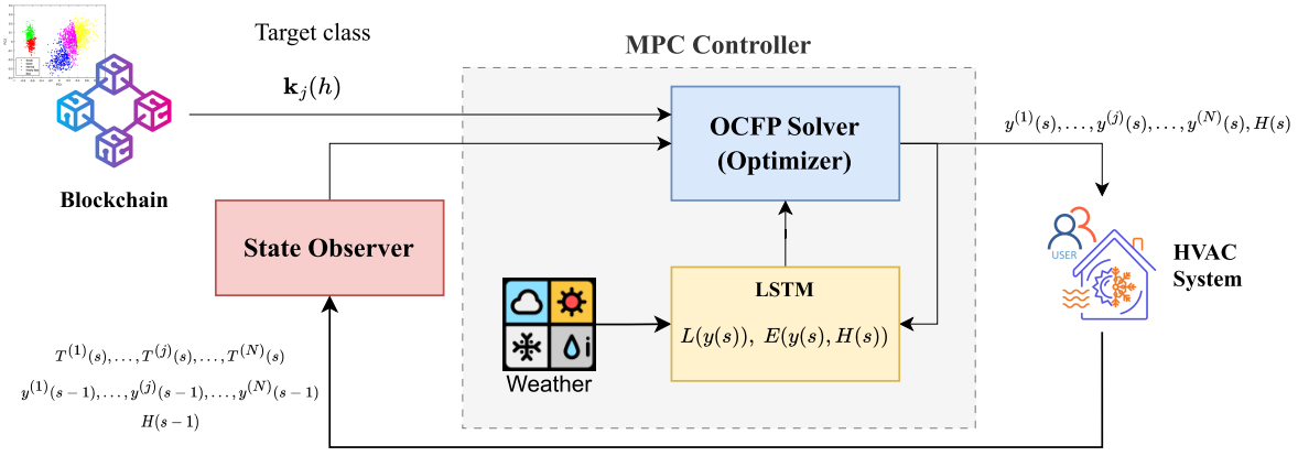
Fig. 4. MPC architecture.
