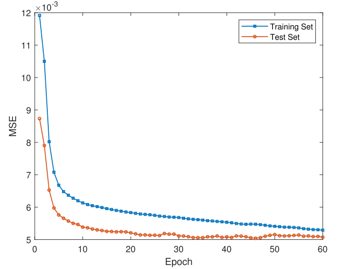
Fig. 8. LSTM training.
