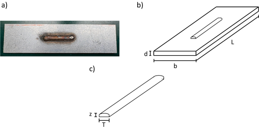
Fig. 5. a) Reinforced specimen before bending; b) reinforced specimen schematization with nominal dimensions of b = 20 mm, L = 80 mm, and d = 1.5 mm; c) dimensions of the elliptic-reinforce: T major axis, z minor semi-axis.
