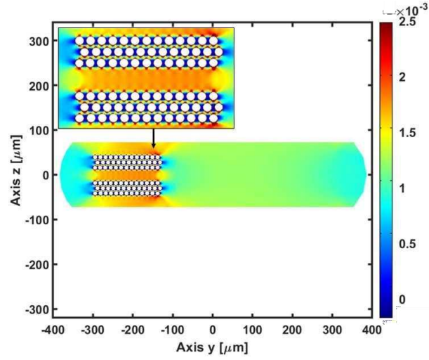
Figure 3.5 Strain distribution \epsilon_y in the MFOF cross-section embedded in the CFRP lamina, for a tensile stress \sigma_y = 35 \text{ MPa} along the y axis [40].
