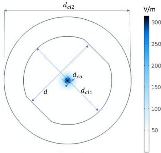
Figure 5.1 Fiber cross-section geometry and electric field norm E of the fundamental mode \text{HE}_{11} at signal wavelength \lambda_s [161].
