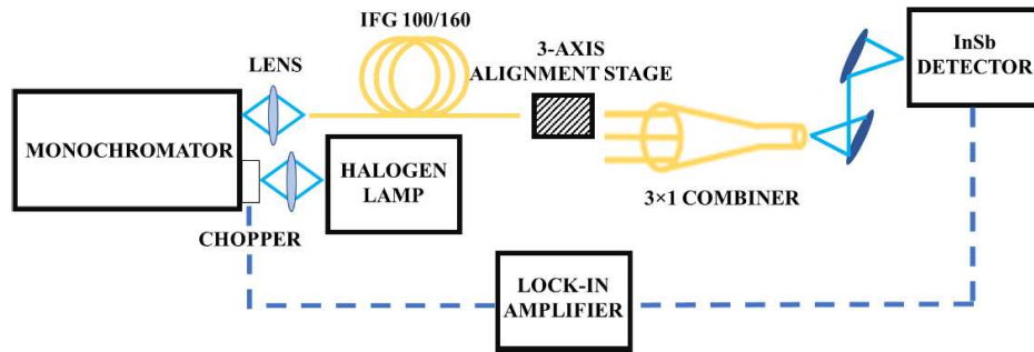
Figure 4.11 Schematic of the experimental set-up used for 3 \times 1 fluoroindate combiner characterization from NIR to Mid-IR [73].
