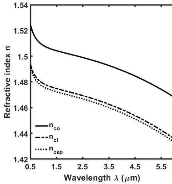
Figure 4.2 Refractive index n as a function of the wavelength \lambda ; core refractive index n_{co} (solid line), cladding refractive index n_{cl} (dashed line), capillary refractive index n_{cap} (dotted line) [73].
