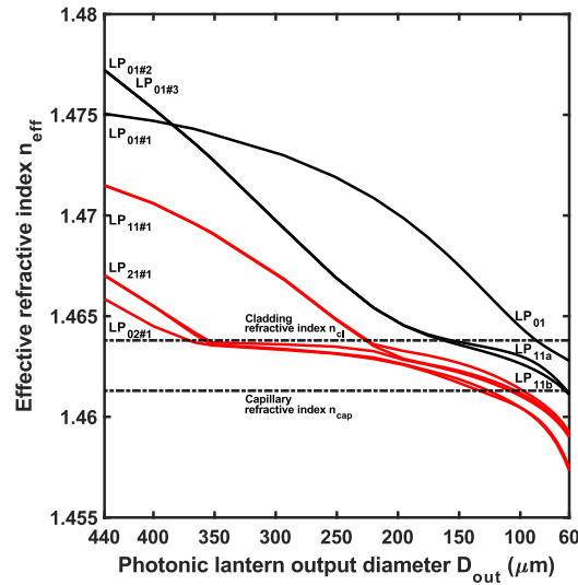
Figure 4.23 Effective refractive index n_{eff} of the first eight spatial modes at the wavelength \lambda = 3.34 \mu m of the mode-group selective photonic lantern based on indium fluoride glass, for different photonic lantern output diameter D_{out} [219].
