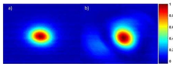
Figure 4.44 Measured farfield beam profile, captured with Pyrocam IIIHR at the wavelength \lambda = 3.34 \mu m ; a) before the down-taper, b) in the waist region [78].
