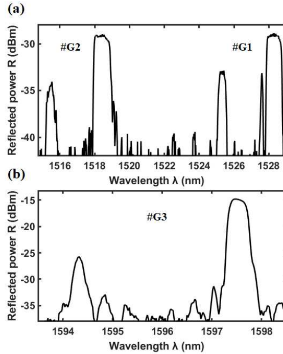
Figure 3.25 Measured reflection spectra of the unperturbed Bragg gratings (a) #G1, #G2 and (b) #G3; length of the Bragg grating L = 12 mm, refractive index modulation of the Bragg grating \Delta n_{BG} = 2 \times 10^{-4} [61].
