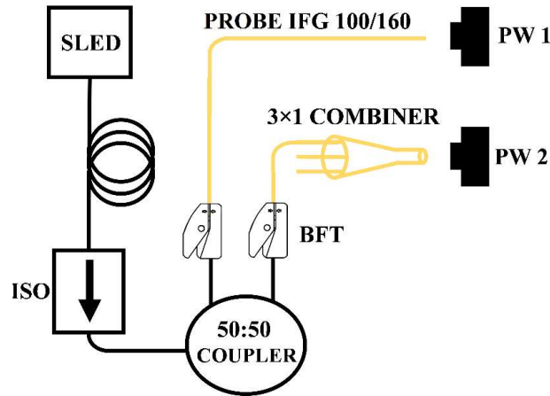
Figure 4.10 Sketch of the experimental set-up used to characterize 3 \times 1 fluoroindate combiner transmission efficiency \eta_{m,net} at the wavelength \lambda = 1.55 \mu\text{m} . The silica optical fibers are represented in black, the fluoroindate optical fibers in yellow [73].
