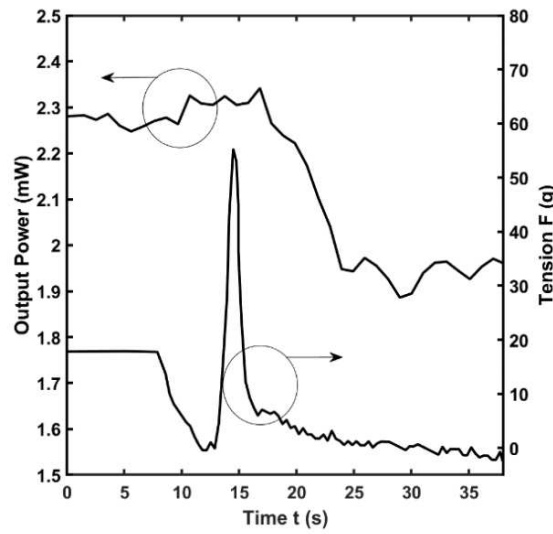
Figure 4.43 Output power P_{out} at wavelength \lambda = 635 nm and tension F measured during the fabrication of the non-adiabatic tapered optical fiber [78].
