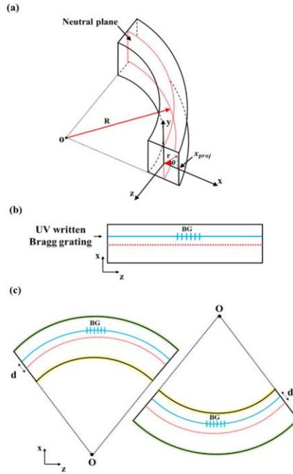
Figure 2.1 (a) 3D-sket of a curved waveguide. (b) 2D-sket of the straight optical waveguide. (c) 2D-sket of the curved optical waveguide with positive (left) and negative (right) curvature C (green colored line for tensile strain, yellow colored line for compressive strain) [60].
