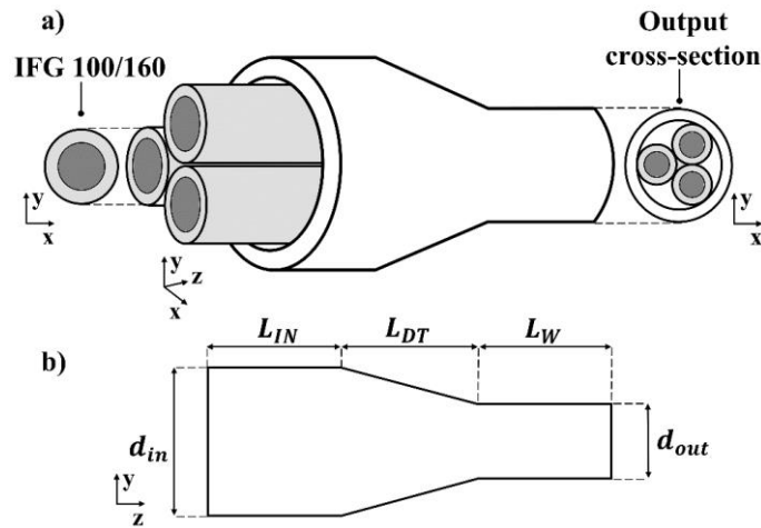
Figure 4.1 (a) 3 \times 1 fluoroindate combiner sketch; (b) longitudinal section in the y-z plane of the 3 \times 1 fluoroindate combiner with linear down-taper [73].
