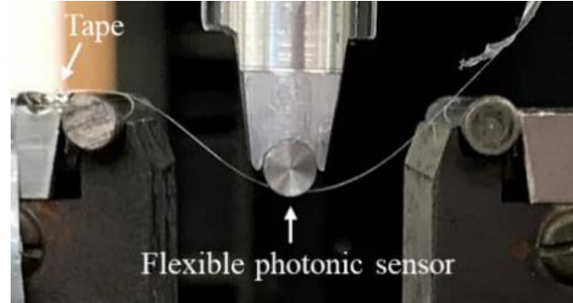
Figure 3.26 Photograph of the experimental set-up. Centre-to-centre separation of rollers s = 20 \text{ mm} , diameter of rollers d_{\text{roll}} = 6 \text{ mm} [61].
