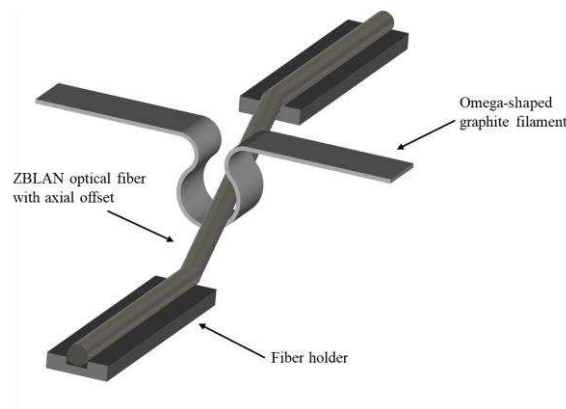
Figure 4.47 Schematic illustration of the fabrication procedure of the S-tapered ZBLAN optical fiber based on resistive filament heating and off-axis pulling.
