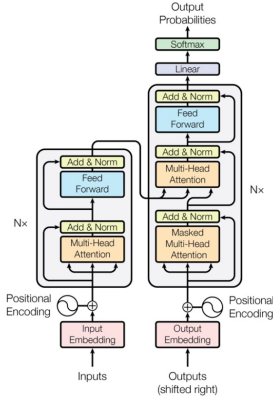
Fig. 2.5 Original Transformer architecture. Image from Vaswani et al. [95]
