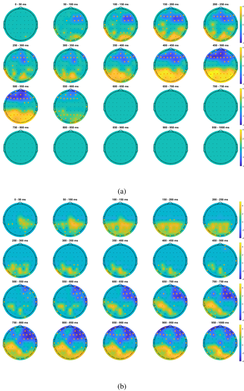
Fig. 5.6 Clustered t-value for AF (a) and NF (b) in Forward vs Backward. The color map represents the value of the t-statistic. Significant channels ( p < 0.05 ) are circled and highlighted in red.
