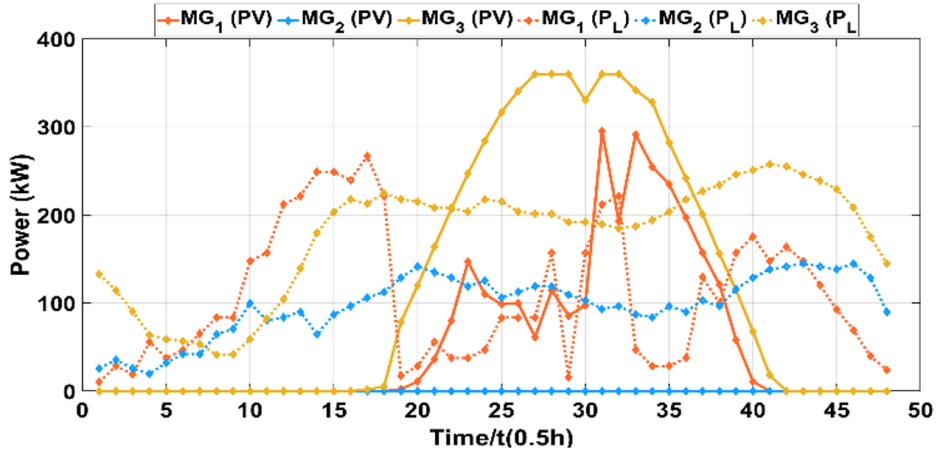
Figure 2.11: The power generation data for all the PV systems and the load profiles
