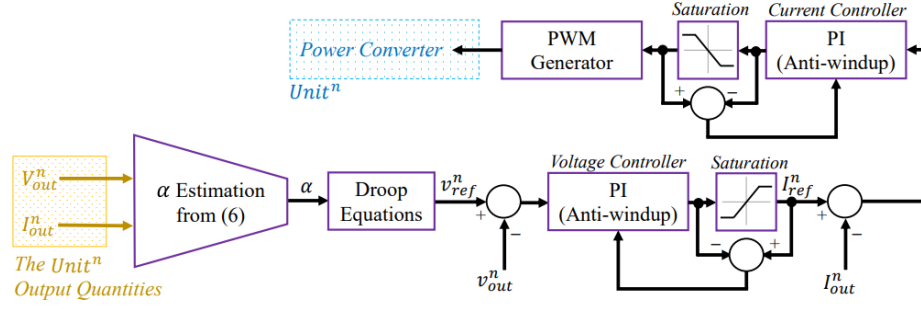
Figure 4.3: Control diagram of unit's power converter
