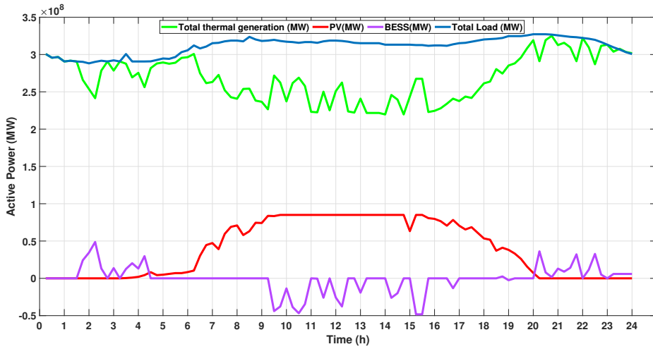
Figure 2.17: Total generation, battery power, PV and the total load demand in (MW)
