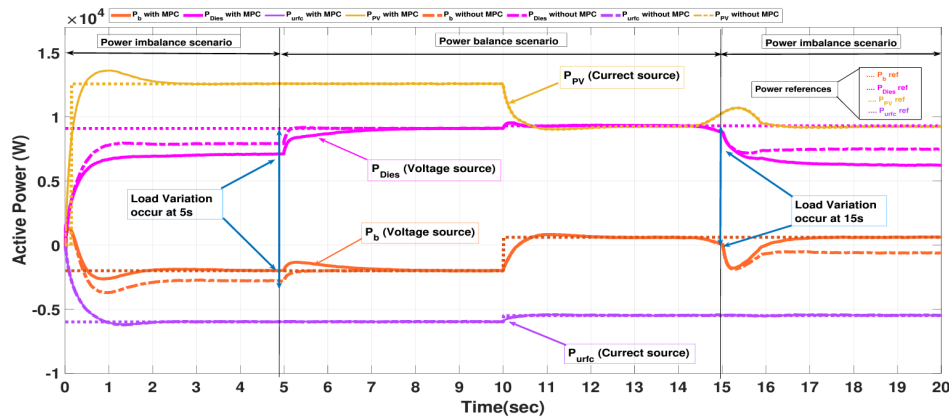
Figure 3.15: Results of the \omega_{Dies} and \omega_b with and without MPC consideration
