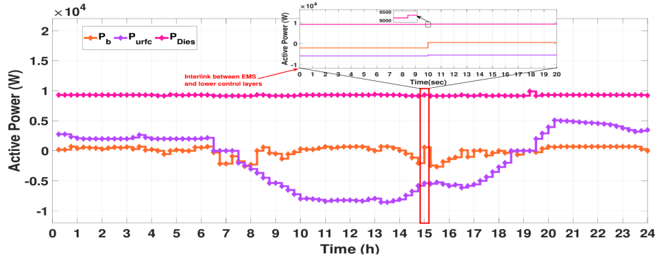
Figure 3.13: EMS dispatch results for the P_{Dies} , P_b and P_{urfc}
