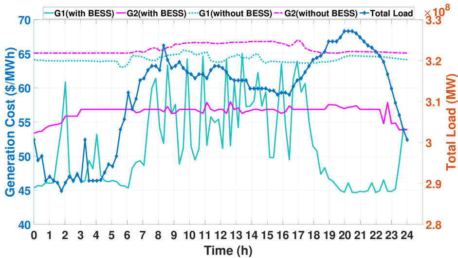
Figure 2.21: Generation costs ($/MWh) with and without BESS, along with total load demand (MW)
