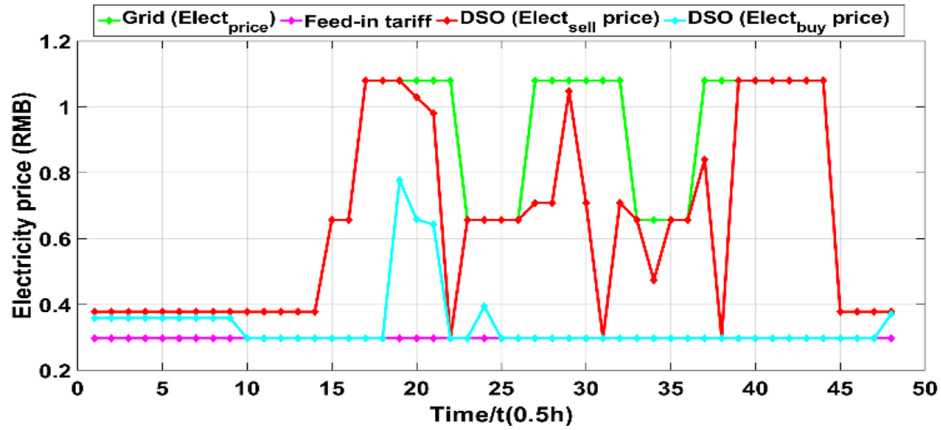
Figure 2.12: Outcomes of optimizing the internal electricity price
