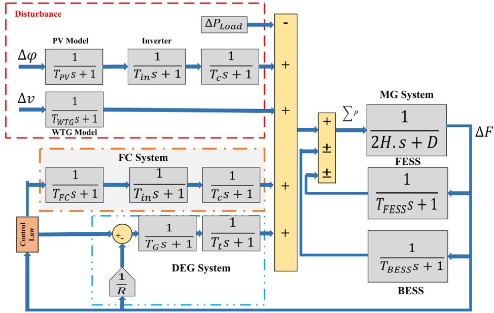
Figure 3.3: Frequency response of MG model, under study
