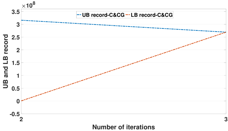
Figure 2.20: C&amp;CG Convergence
