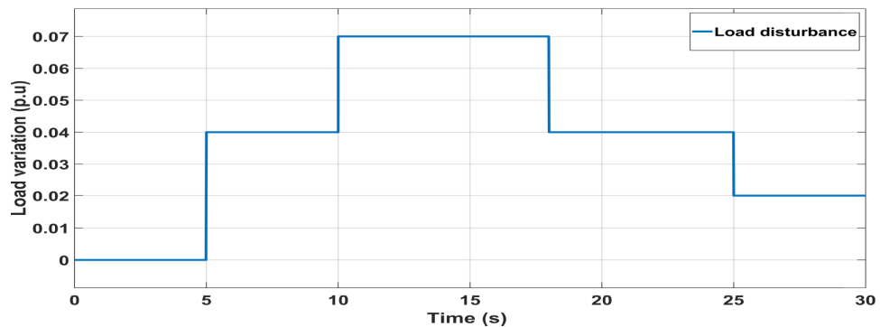
Figure 3.6: Load Variation
