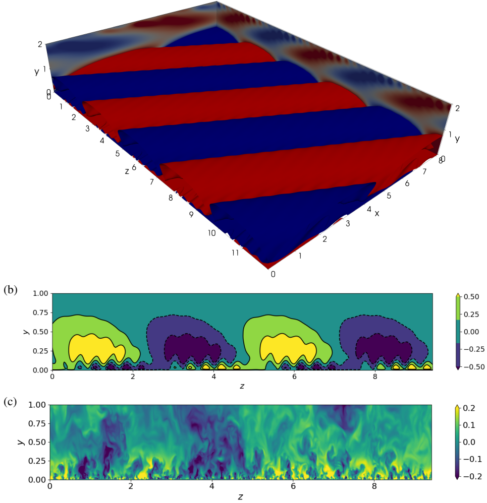
Figure 13: (a) Streamwise velocity component iso-contours (mode amplitude normalized to one, contour value 0.1) of the leading unstable eigenmode reported in the DNS x - y - z reference frame at Re_\tau = 1000 ( \alpha = 1.0 , A_s = 0.20 , \theta \approx 14^\circ , N_u = 60 ). (b) y - z cut of the same mode in (a). (c) Instantaneous streamwise component of the turbulent fluctuation extracted from a snapshot of the large-domain DNS at Re_\tau = 1000 (C1000 L ), y - z cut.
