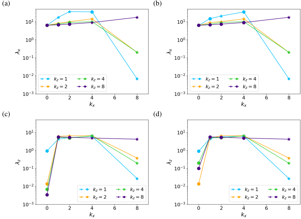
Figure 11: Streamwise (a,b) and spanwise (c,d) wavelengths of the streamwise velocity component of the leading unstable modes (★) or least stable modes (●) reported in the DNS reference frame as functions of base flow wavenumbers \{k_x, k_z\} for (a,c) Re_\tau = 590 and (b,d) Re_\tau = 1000 . All computations were performed with \alpha = 1.0 , A_s = 0.20 and N_u = 60 .
