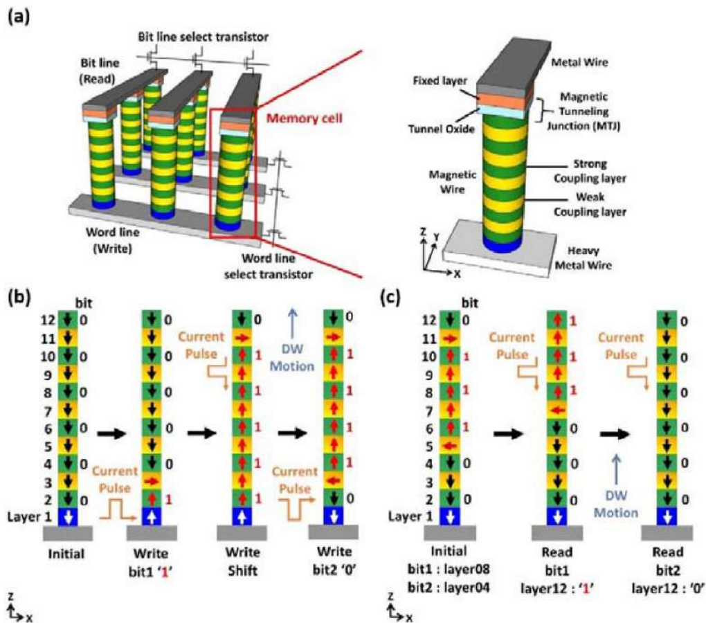
Figure 33. (a) Illustration of the vertical DW motion memory with artificial ferromagnets. Left panel: Memory array with vertically arranged word line and bit line. The columns within the array are the multi-bit memory cells constructed with artificial ferromagnets. Right panel: Detailed structure of a column. (b) Data writing scheme: A current is applied to the bottom electrode to invert the magnetization direction of layer 1 by spin-orbit torque. A DW is then generated in layer 3. The current is then passed through the column to shift this DW up to any DW layer. The next information is then written by inverting the magnetization direction of layer 1 by applying a current to the bottom electrode. By repeating this operation, any bit sequence can be stored in the column. (c) Readout can be done in batches by reading out the information at the top MTJ while shifting all DWs upwards with a current. Reproduced from [194]. CC BY 4.0.
