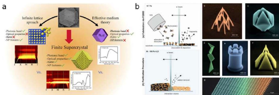
Figure 17. (a) Approaches to calculate the properties of photonic crystals, i.e. infinite lattice for band structure calculations, effective medium theory for optical properties like reflectance, and proposed FDTD simulation for finite supercrystals. (b) Fabrication, purification, and 3D possibilities. Top-left side: a gas injection system (GIS) injects preheated precursor molecules in gaseous states ( \text{Me}_2(\text{acac})\text{Au}(\text{III}) in this study) in close proximity to the substrate, where they adsorb, diffuse and, if not dissociated, eventually desorb again. Upon interaction with a focused electron beam, local dissociation leads to immobilization of the respective metal, which forms the intended deposit. As a result of incomplete ligand cleavage not only Au atoms (orange spheres) but also carbonaceous fragments (grey spheres) are co-deposited, which is why FEBID structures naturally contain high amounts of carbon. The whole fabrication procedure is typically performed at 21 \pm 1^\circ\text{C} and 10–5 Pa. Right panel: 3D nano-printing design possibilities, ranging from meshed objects over sheet-like, semi-closed toward closed and mixed architectures. Also, scalability is provided, to generate micrometre-sized assemblies for individual applications (see tetrapod array). To remove the carbon, the scheme on the bottom-left panel illustrates a suitable purification process, which takes place in a low-pressure \text{H}_2\text{O} atmosphere ranging between 50–100 Pa at 21 \pm 1^\circ\text{C} . Using again the focused electron beam leads to the local removal of carbon, leaving nominally pure, polycrystalline gold nanostructures with a volume loss of up to two thirds. Depending on the height of the nanostructure, the beam conditions must be adapted such that the interaction volume can cover the whole structure volume. Panel (a) is reproduced from [106] with permission from the Royal Society of Chemistry. Panel (b) is [109] John Wiley & Sons. [Copyright © 2023 WILEY-VCH Verlag GmbH & Co. KGaA, Weinheim].
