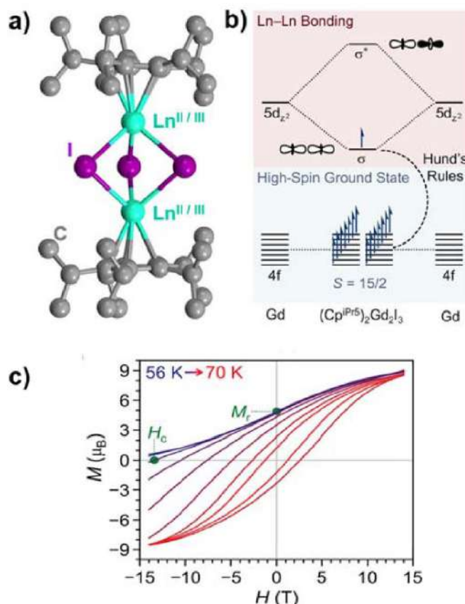
Figure 21. (a) Structure of the complexes of formula (\text{Cp}^{\text{iPr5}})_2\text{Ln}_2\text{I}_3 ( \text{Cp}^{\text{iPr5}} = penta-isopropylcyclopentadienyl; Ln = Y, Gd, Tb, or Dy), (b) Molecular orbital diagram for (\text{Cp}^{\text{iPr5}})_2\text{Gd}_2\text{I}_3 illustrating the mechanism leading to strong ferromagnetic exchange interaction through the formation of a singly occupied \sigma -bonding orbital. (c) Temperature dependence of the magnetic hysteresis of the (\text{Cp}^{\text{iPr5}})_2\text{Dy}_2\text{I}_3 single-molecule magnet showing extremely hard magnetism. Adapted from Ref. [126]. Reprinted with permission from AAAS.
