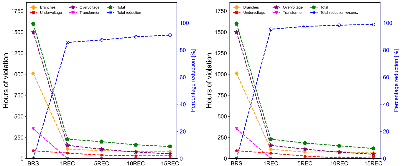
Fig. 4. Analysis of hours with violation as a function of the increasing number of RECs participating in the VI service.
