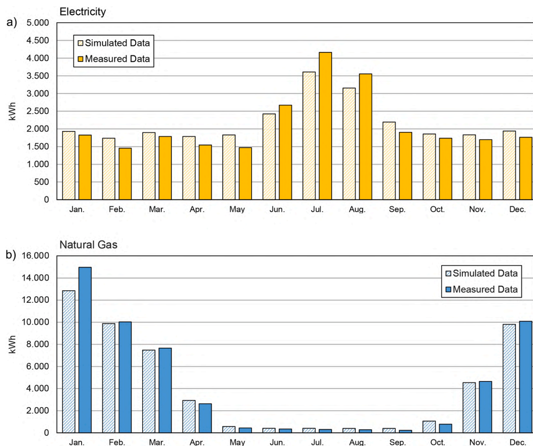
Fig. 11. Energy consumption comparison between simulated and measured data on a monthly basis for electricity (a) and natural gas (b).
