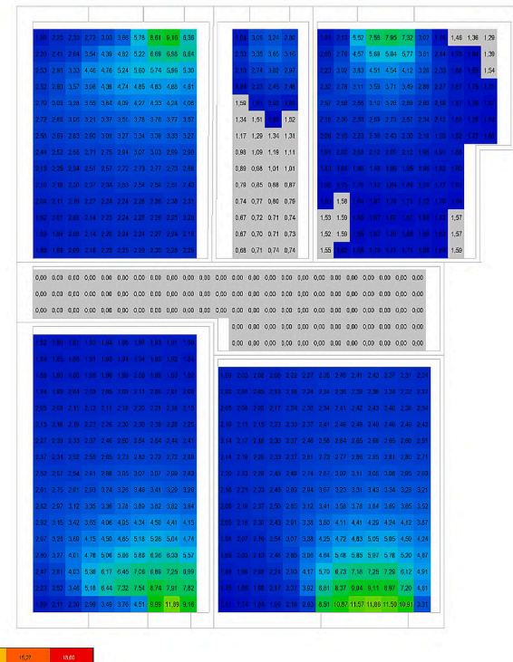
Fig. 17. Minimum Daylight factor ( D_{TM} ) (a) and Reference Daylight Factor ( D_T ) (b) consistency analysis with EN 17037 without and without en-SOLEX system.
