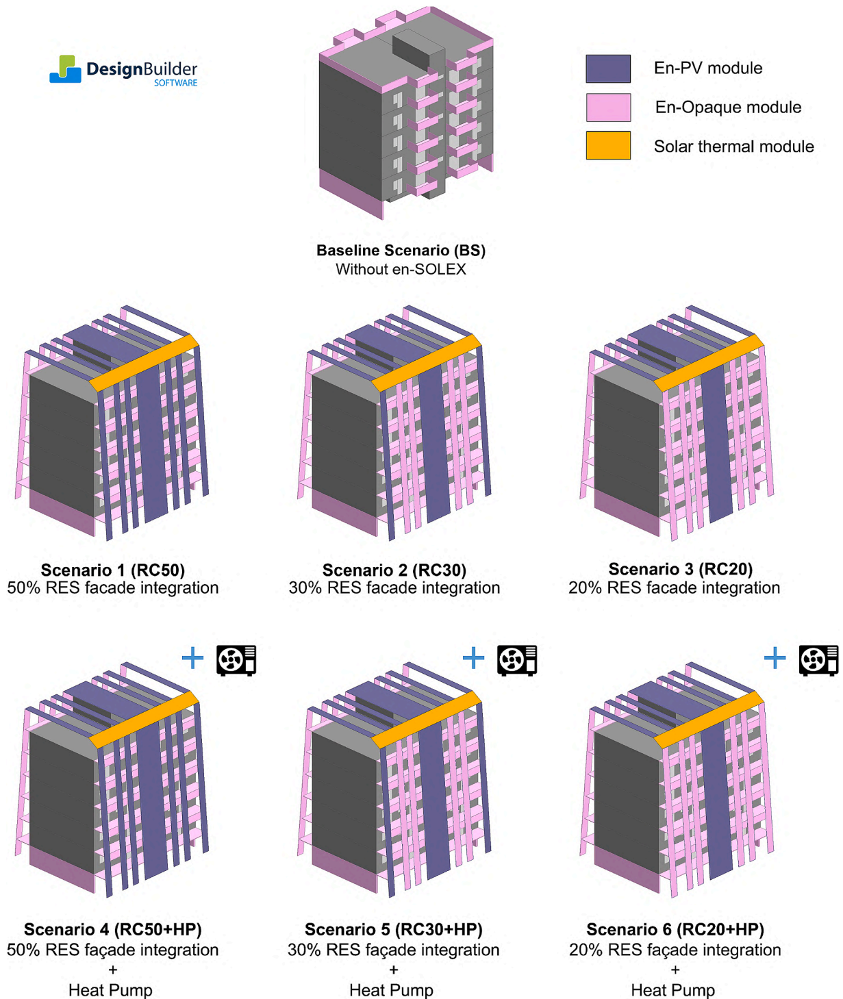
Fig. 9. Design builder 3D model for each analysed scenario.
