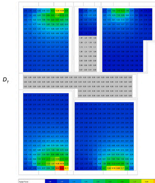
Fig. 17. Minimum Daylight factor ( D_{TM} ) (a) and Reference Daylight Factor ( D_T ) (b) consistency analysis with EN 17037 without and without en-SOLEX system.
