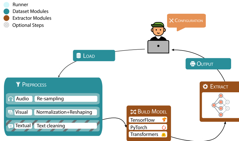
Figure 1: DUCHO's pipeline for multimodal feature extraction, managed by the Dataset, Extractor, and Runner modules.
