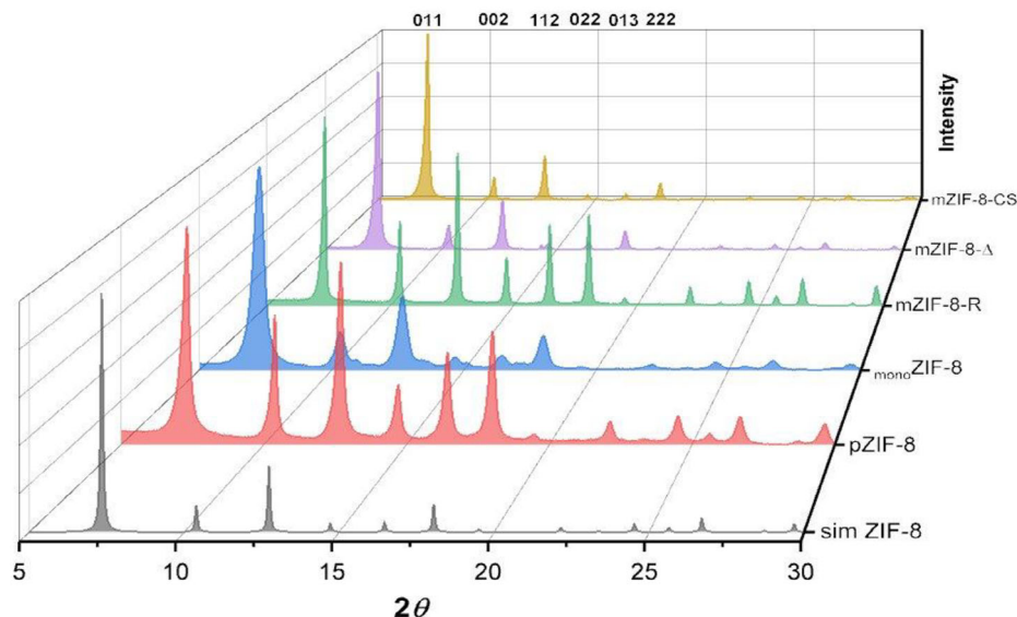
Figure 1. Selected PXRD data, including hkl reflections, for samples in Experimental Section Table 4 (see below). — Simulated ZIF-8; — \text{monoZIF-8} (entry 1); — \text{pZIF-8} (entry 3); — \text{mZIF-8-R} (entry 11); — \text{mZIF-8-}\Delta (entry 12); — \text{mZIF-8-CS} (entry 13).
