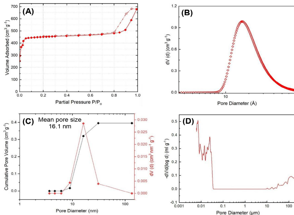
Figure 3. For mZIF-8-Δ: A) N_2 adsorption-desorption isotherm collected in the range 0–1 bar at 77 K (♦ adsorption, ◇ desorption), B) Corresponding microporous DA PSD, C) BJH mean (◆) and PSD (♦) obtained from the N_2 isotherm data, and D) Macroporous PSD obtained from Hg Porosimetry.
