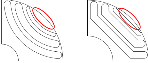
Fig. 10. Main difference between the 3C (a) and the I2U (b) optimal rotors.
