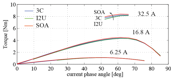
Fig. 16. Comparison of the measured average torque as a function of the current phase angle at different current amplitudes for the three prototypes.
