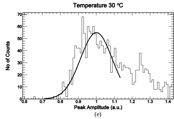
Fig. 9. Peak spectra measured when the compensation system is active, for different temperatures: 25°C (a), 22.5 °C (b), 25 °C (c), 27.5 °C (d), 30 °C (e).
