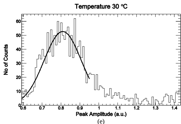
Fig. 8. Peak spectra measured when the compensation system is disabled, for different temperatures: 25°C (a), 22.5 °C (b), 25 °C (c), 27.5 °C (d), 30 °C (e).
