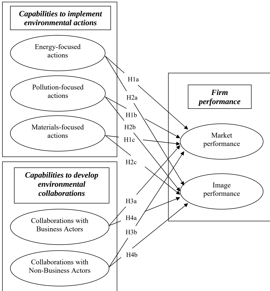
Figure 1: Theoretical framework
