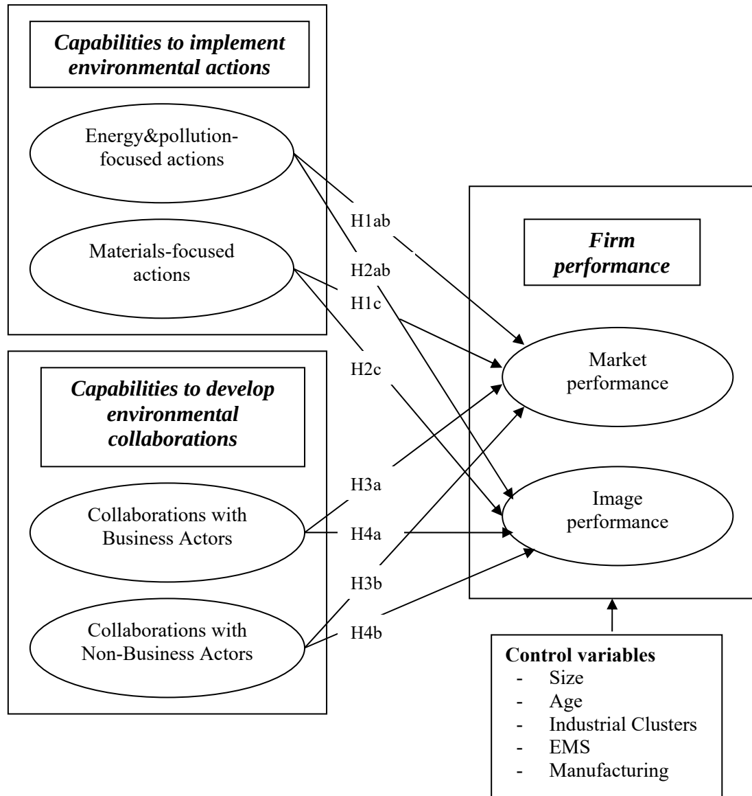
Figure 2: Tested model
