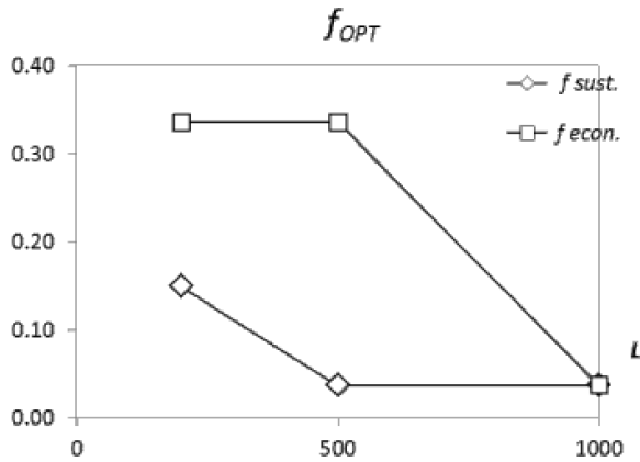
Fig. 3. f_{OPT} values in case of cv = 0 for different transportation distances.
