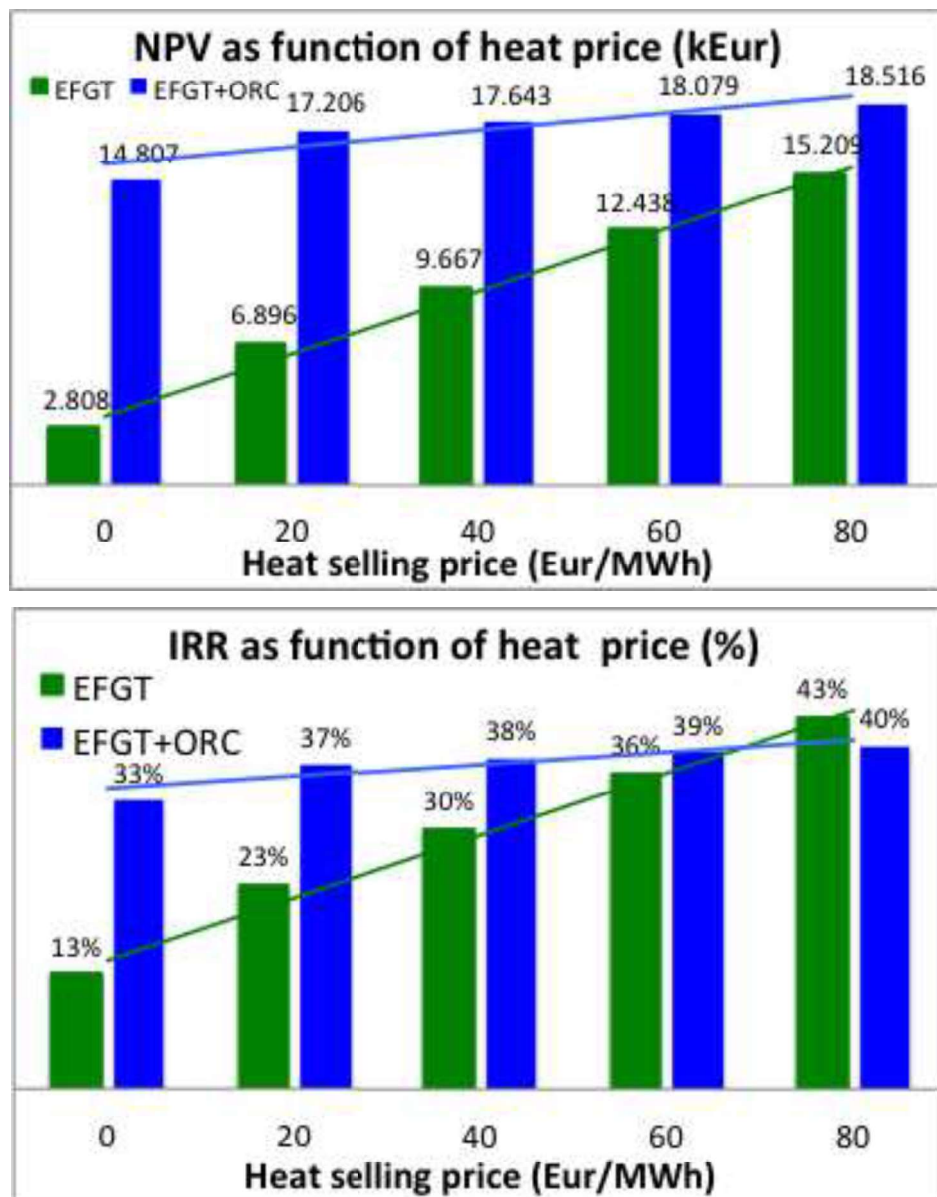
Figure 12. NPV (top) and IRR (bottom) of the investment as a function of the heat selling price P_T
