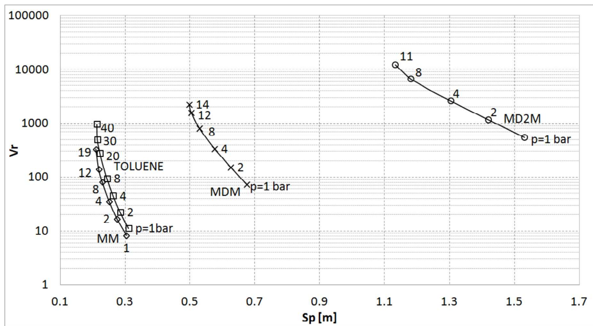
Figure 9 – Volumetric expansion ratio and Size Parameter chart. Comparison between MM, MDM, MD2M and Toluene
