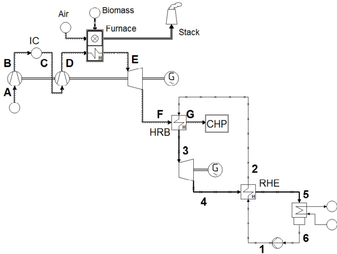
Figure 1 – EFGT+ORC Combined Cycle Plant Layout
