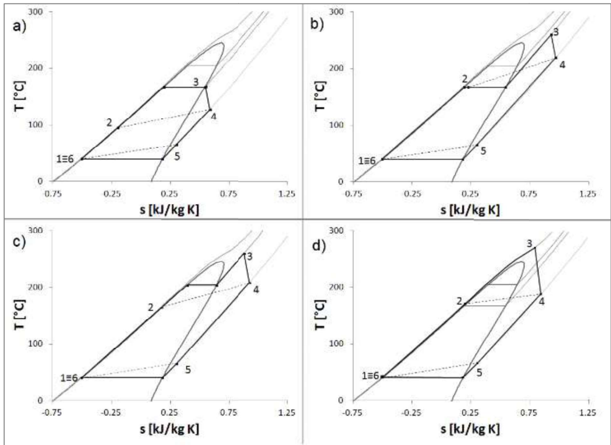
Figure 3 – T-s chart for some examined cases: a) p_{ev}=5 bar, saturated; b) p_{ev}=5 bar, T_3=260^\circ\text{C} ; c) p_{ev}=10 bar, T_3=260^\circ\text{C} ; d) supercritical cycle p_{ev}=25 bar, T_3=270^\circ\text{C}
