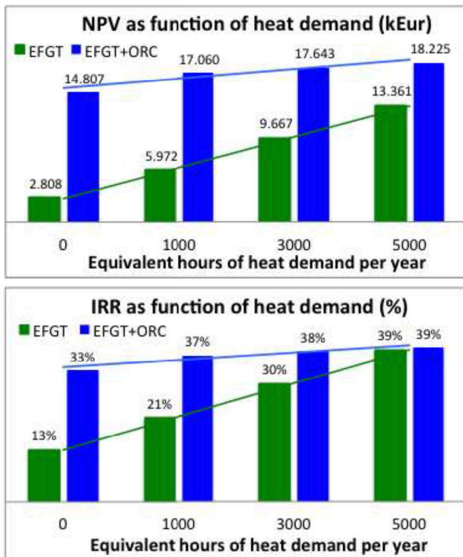
Figure 11. NPV (top) and IRR (bottom) of the investment as a function of the heat demand H_T (hour/y)
